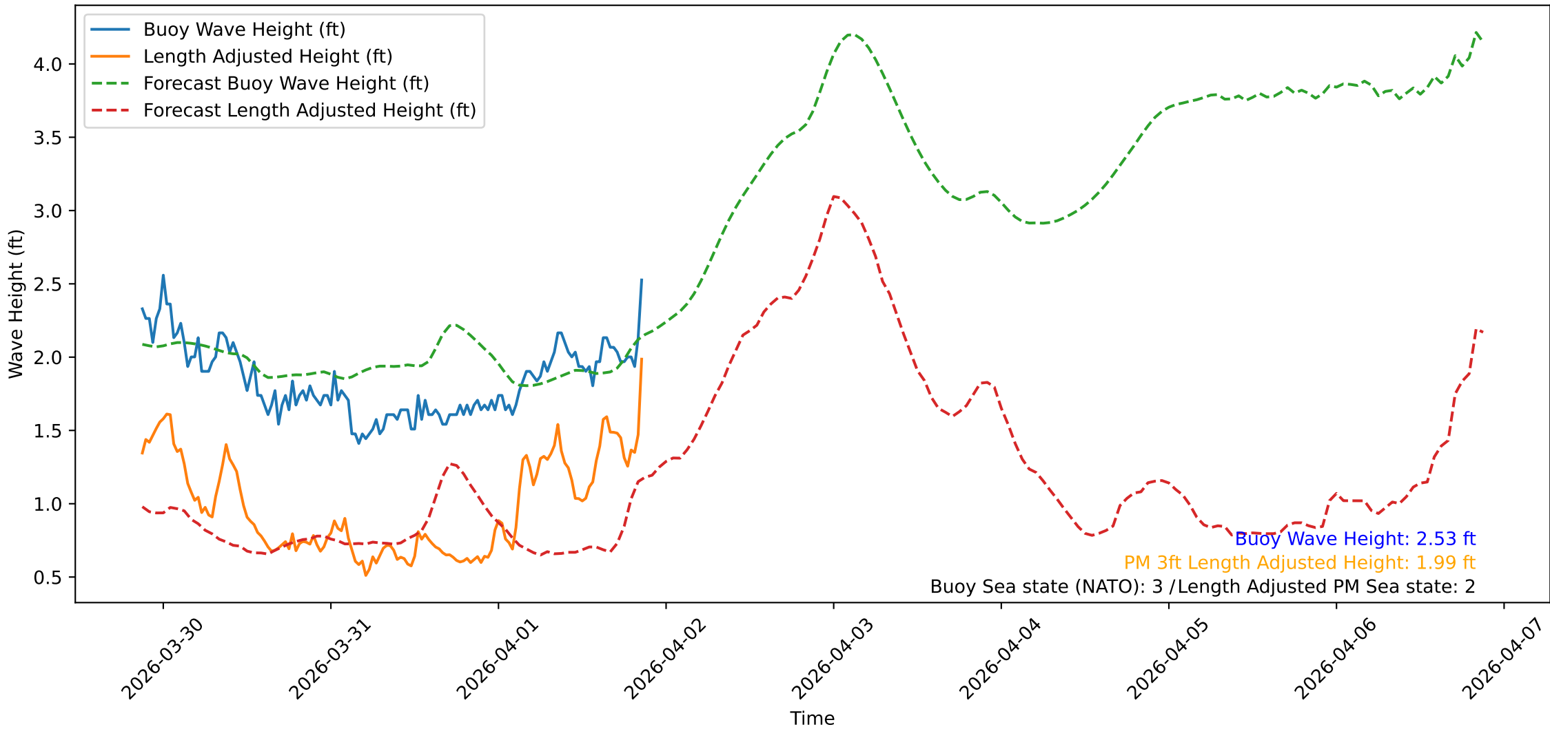
Wave Heights over Time for Green Beach at 2026-04-01 21:11:09
