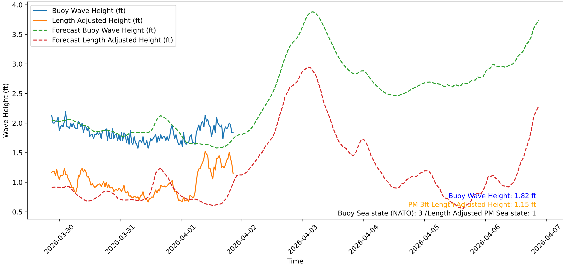
Wave Heights over Time for Oceanside Harbor at 2026-04-01 21:10:31
