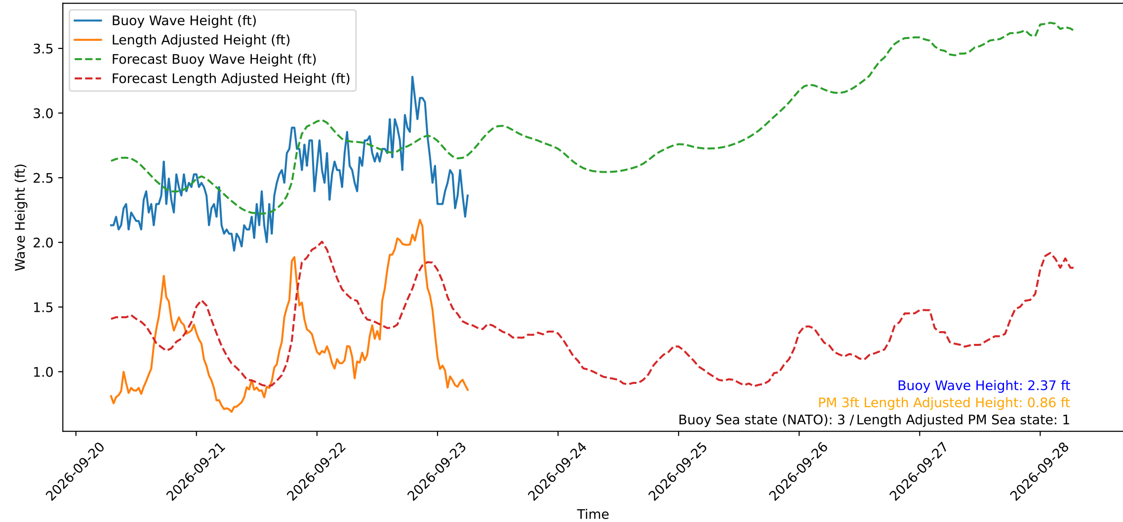
Wave Heights over Time for Red Beach at 2026-09-23 06:40:49
