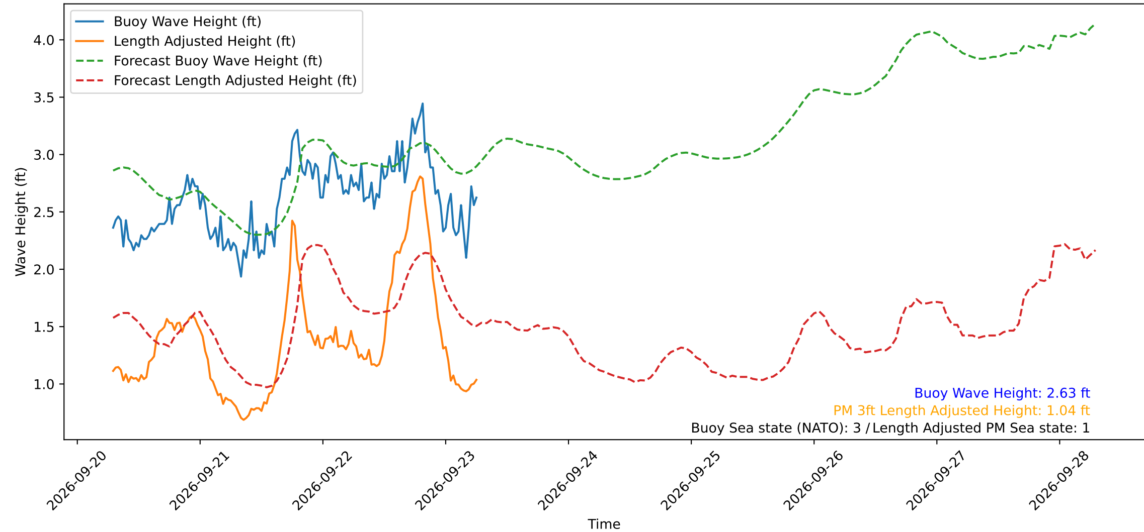
Wave Heights over Time for Green Beach at 2026-09-23 06:41:11
