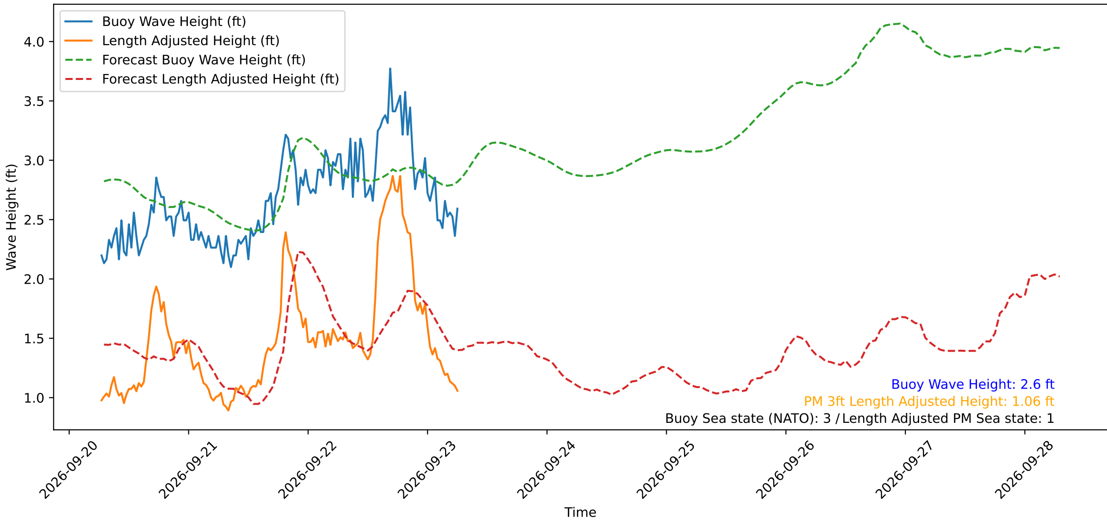
Wave Heights over Time for Oceanside Harbor at 2026-09-23 06:40:29
