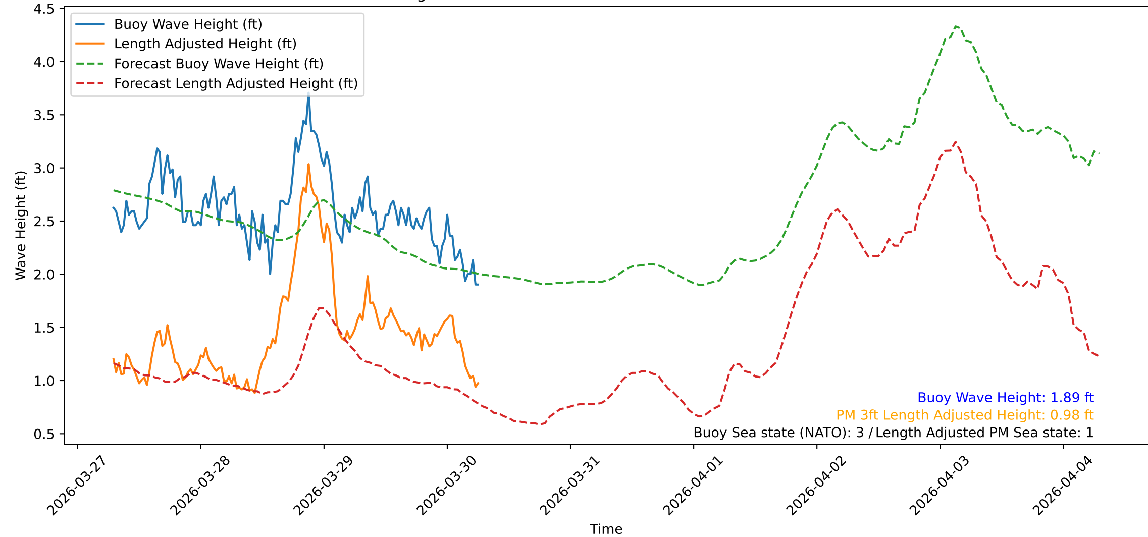
Wave Heights over Time for Green Beach at 2026-03-30 07:01:09
