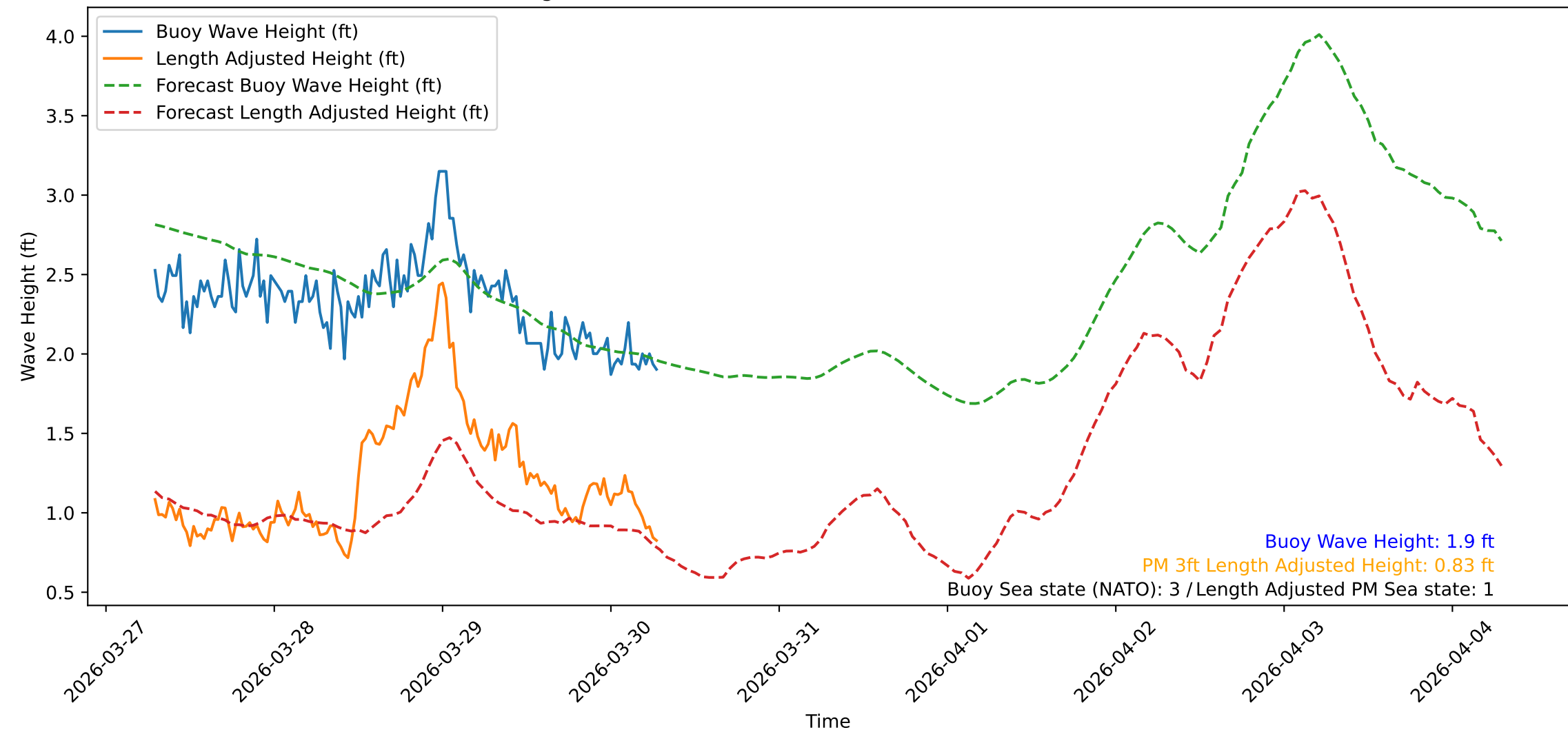
Wave Heights over Time for Oceanside Harbor at 2026-03-30 07:00:31
