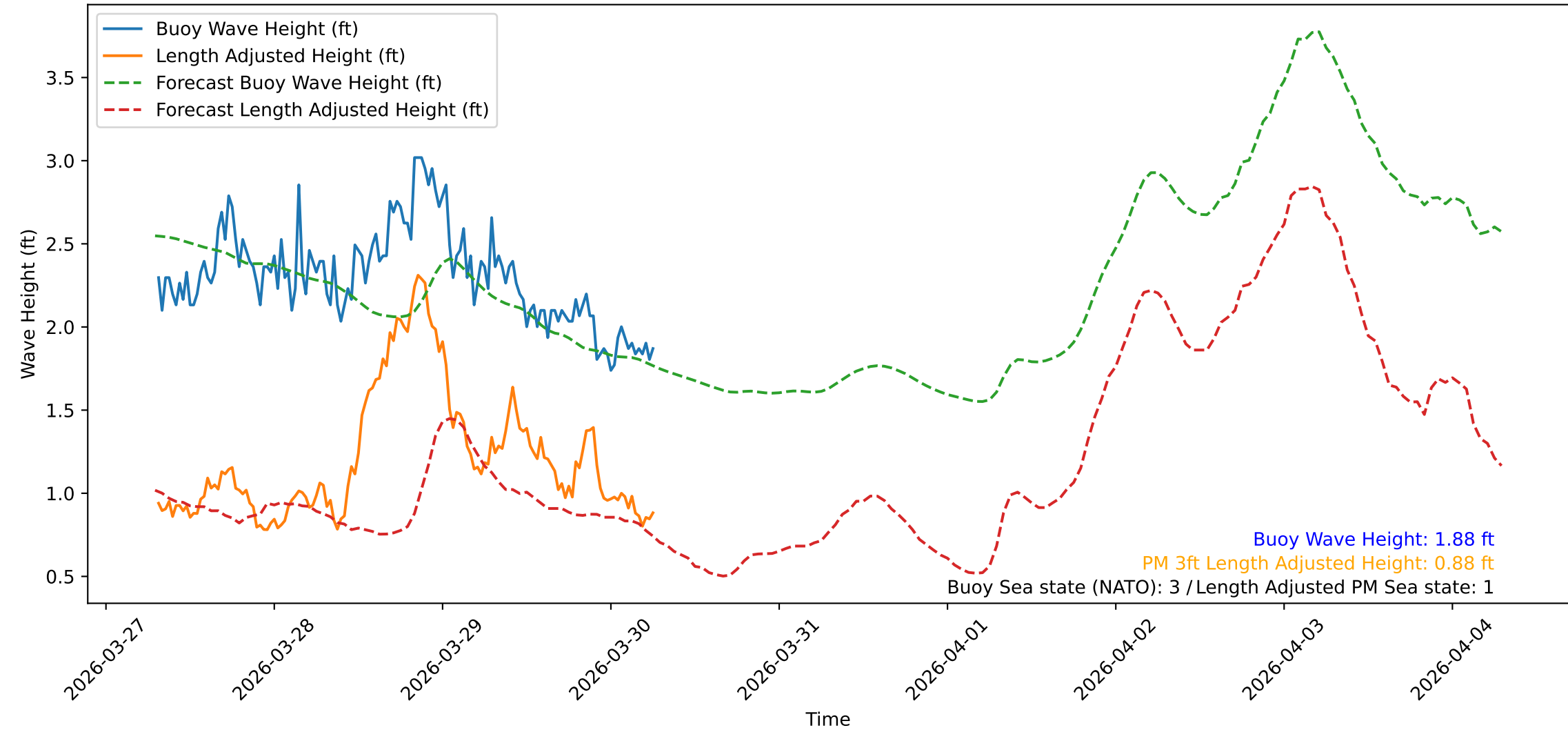
Wave Heights over Time for Red Beach at 2026-03-30 07:00:47
