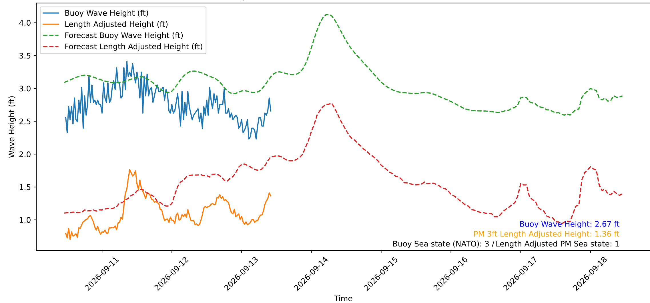
Wave Heights over Time for Red Beach at 2026-09-13 11:00:49
