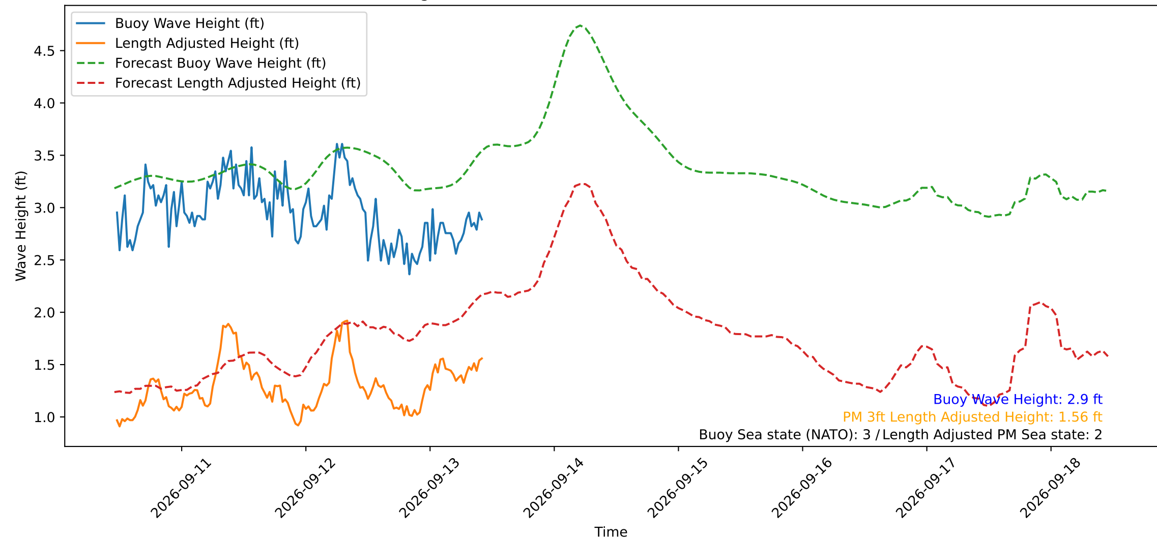
Wave Heights over Time for Green Beach at 2026-09-13 11:01:12
