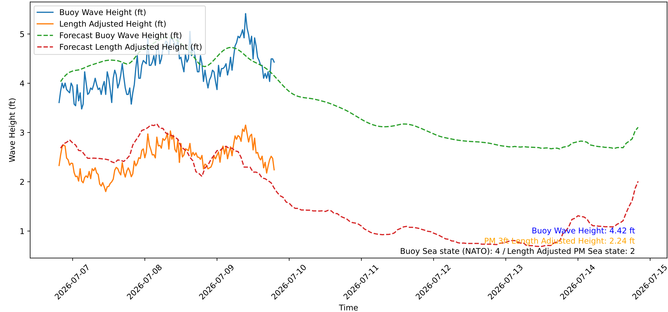
Wave Heights over Time for Oceanside Harbor at 2026-07-09 19:40:26
