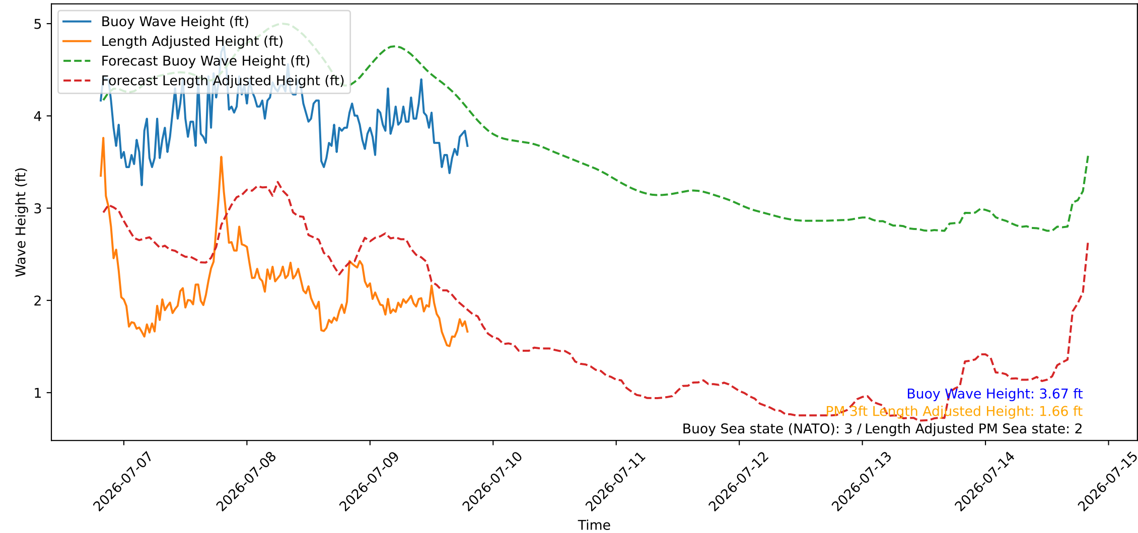
Wave Heights over Time for Green Beach at 2026-07-09 19:41:08
