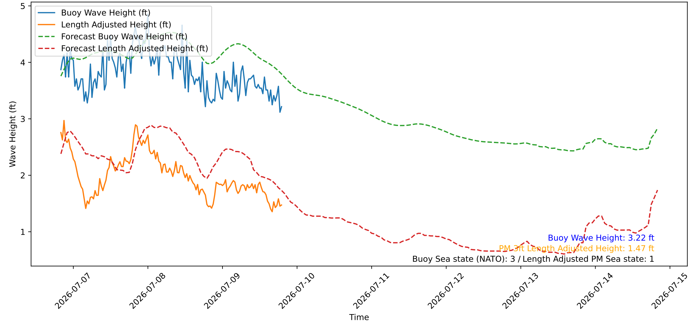
Wave Heights over Time for Red Beach at 2026-07-09 19:40:45
