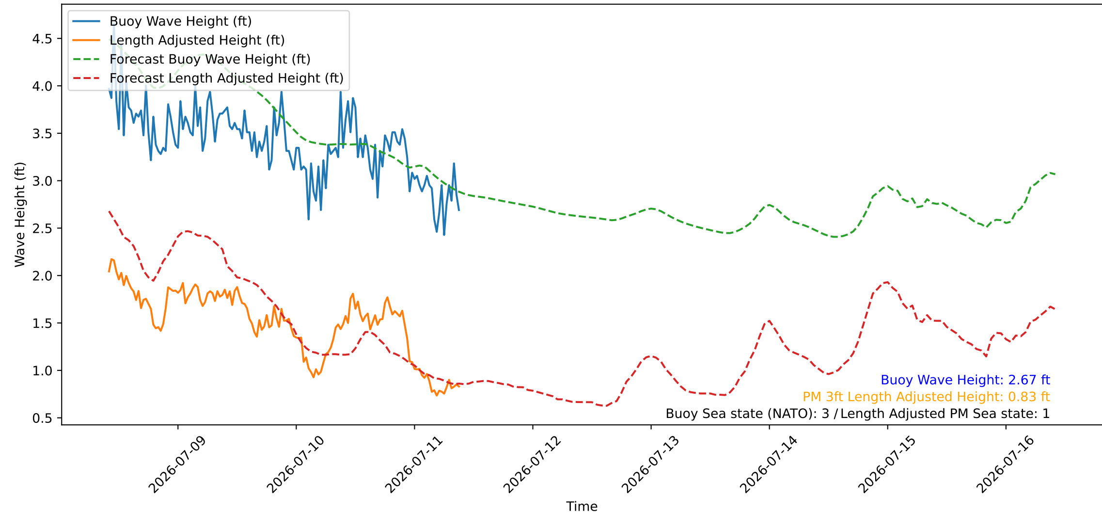
Wave Heights over Time for Red Beach at 2026-07-11 09:50:47
