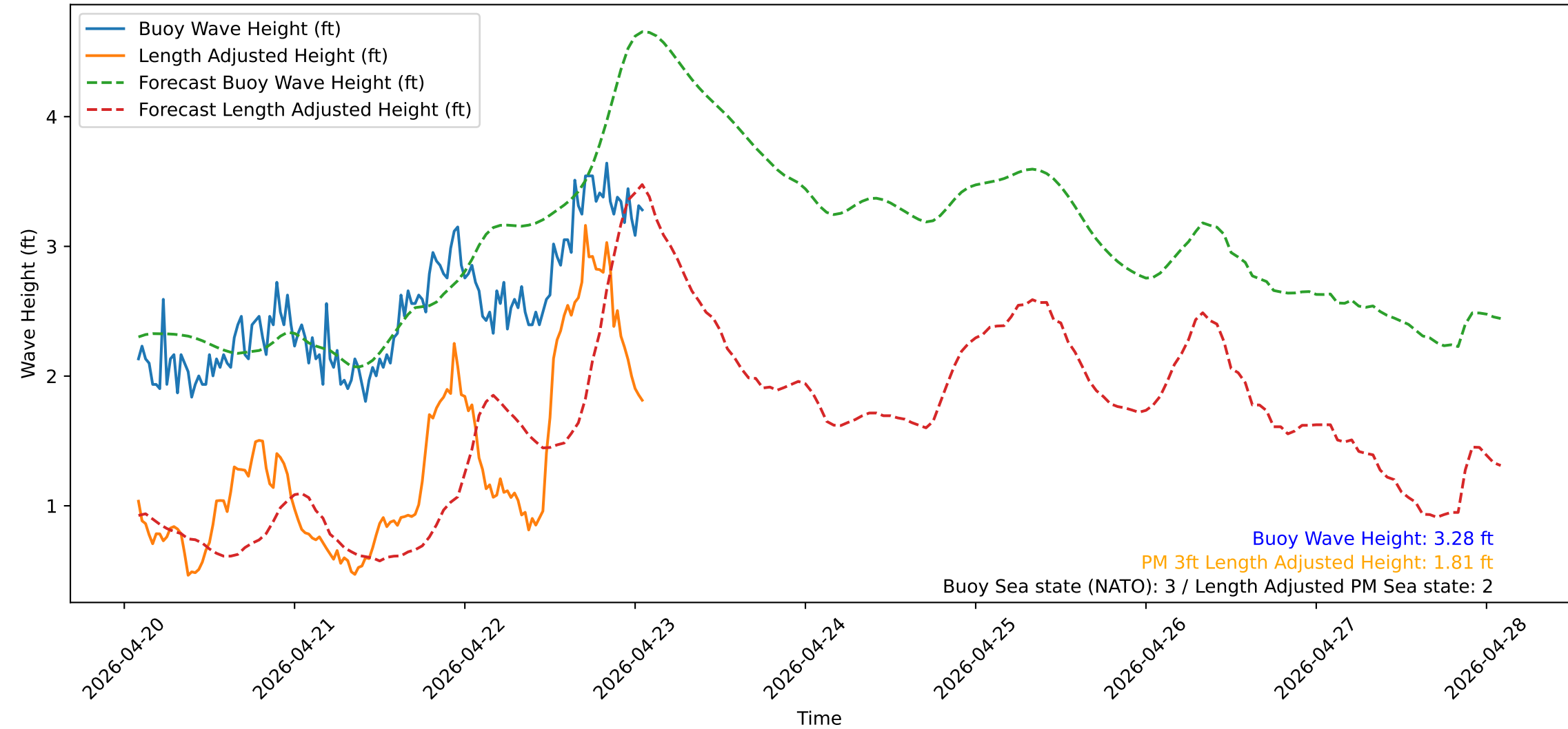
Wave Heights over Time for Red Beach at 2026-04-23 01:50:51
