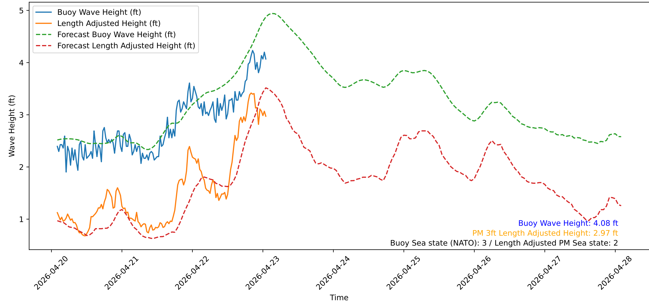
Wave Heights over Time for Oceanside Harbor at 2026-04-23 01:50:31
