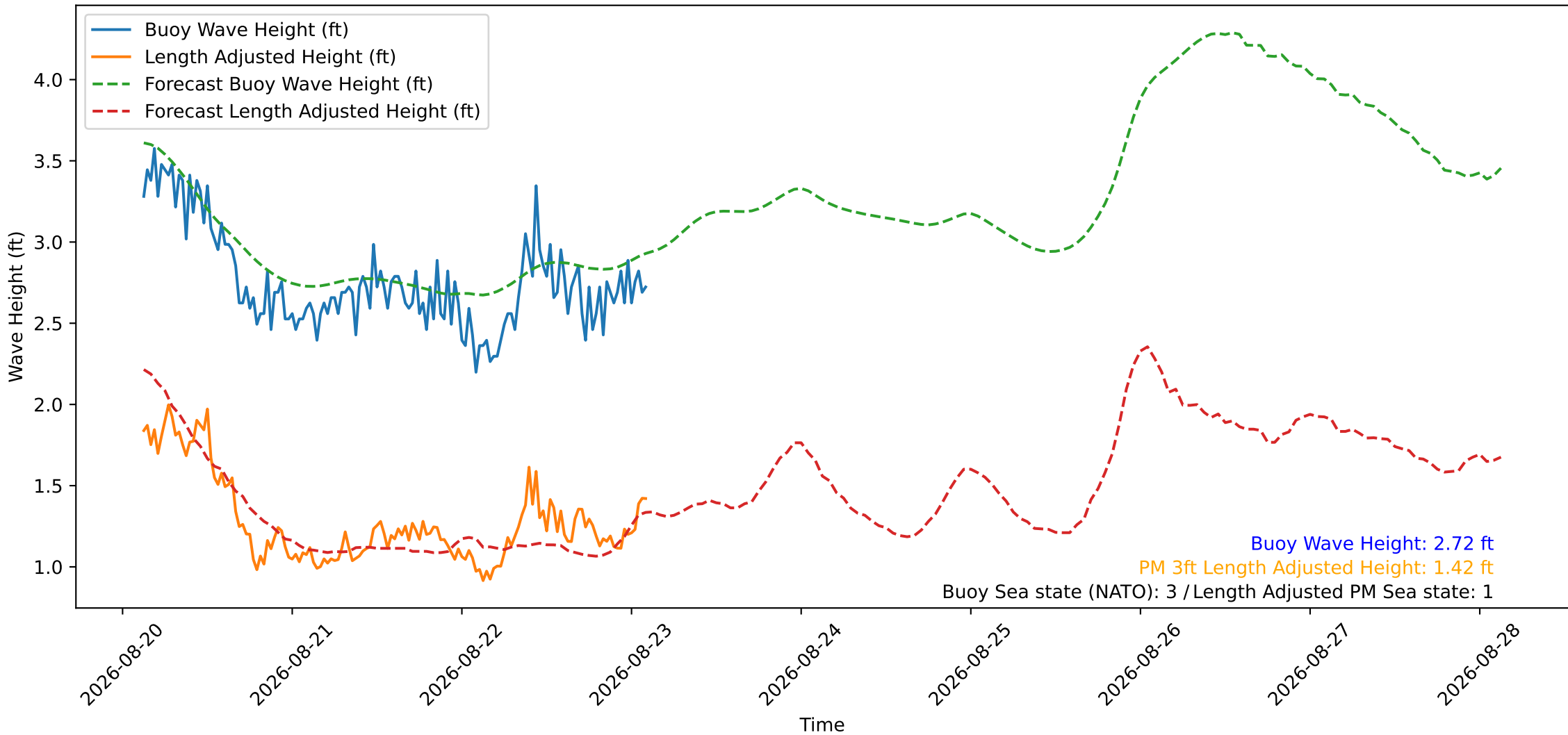
Wave Heights over Time for Oceanside Harbor at 2026-08-23 03:00:29
