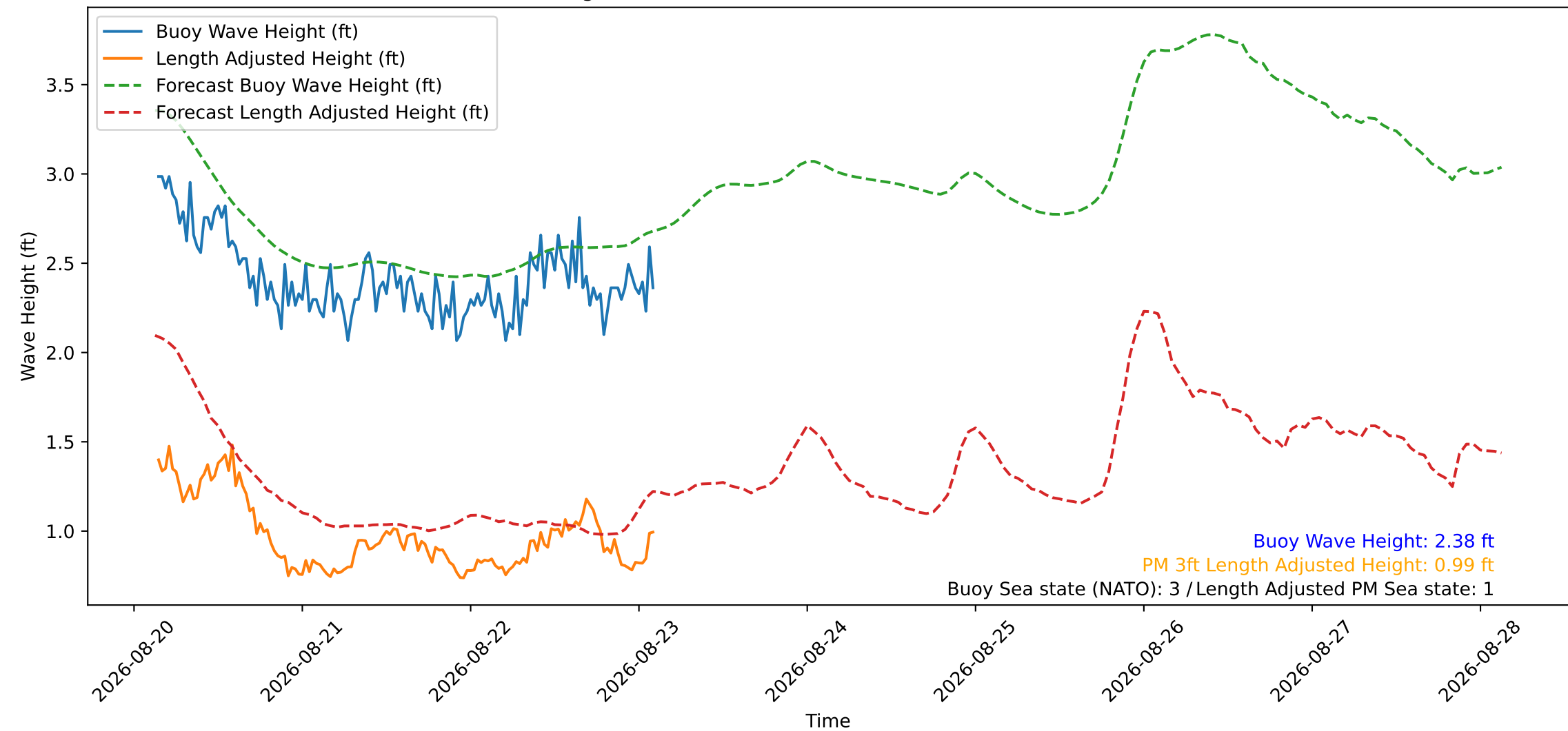
Wave Heights over Time for Red Beach at 2026-08-23 03:00:49
