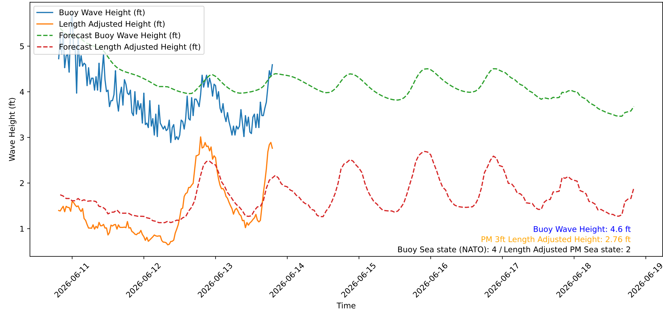
Wave Heights over Time for Green Beach at 2026-06-13 19:41:09
