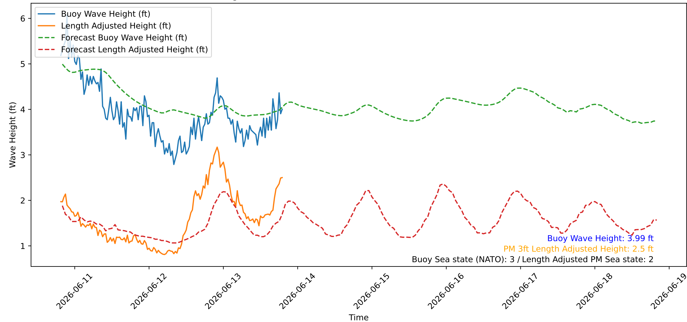
Wave Heights over Time for Oceanside Harbor at 2026-06-13 19:40:26
