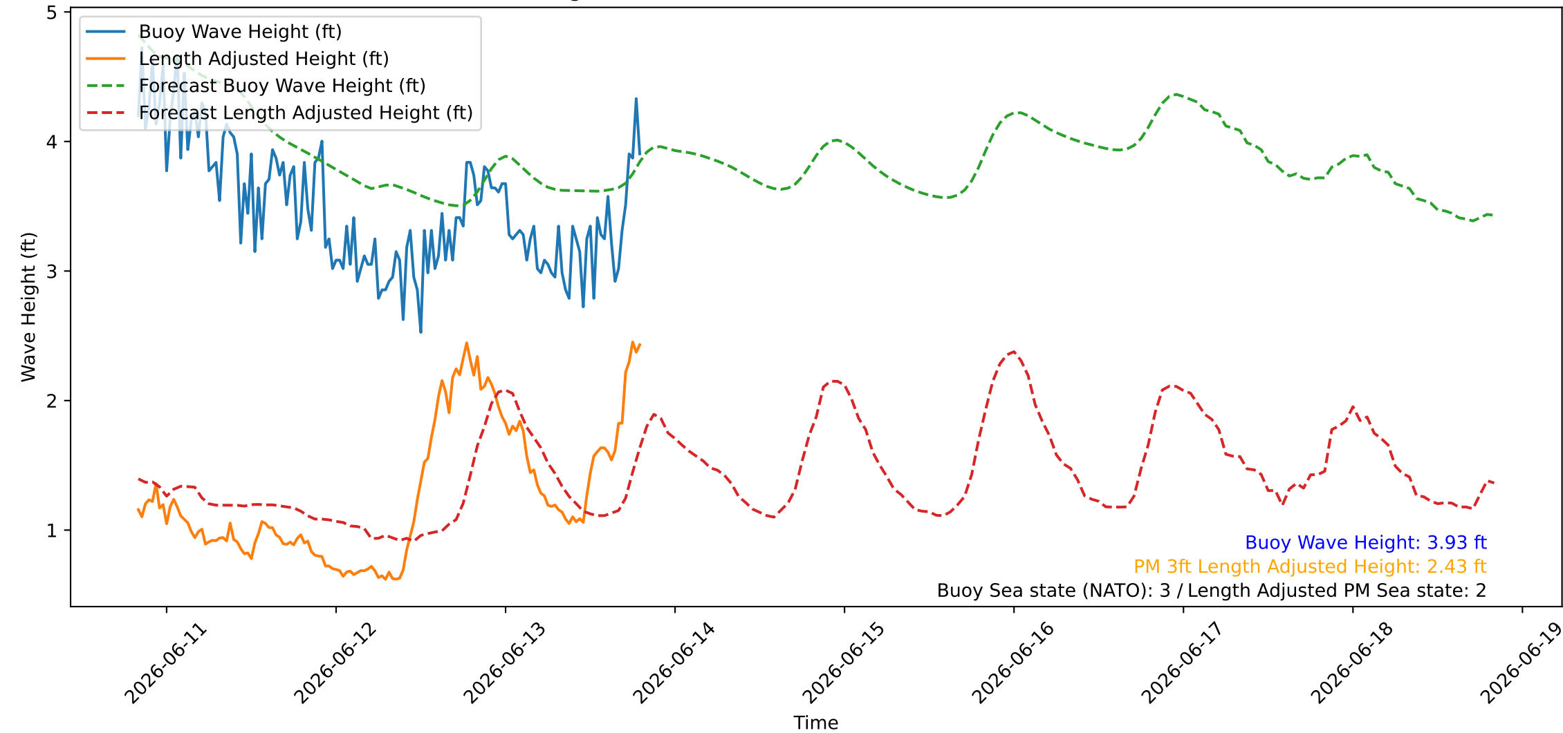
Wave Heights over Time for Red Beach at 2026-06-13 19:40:46
