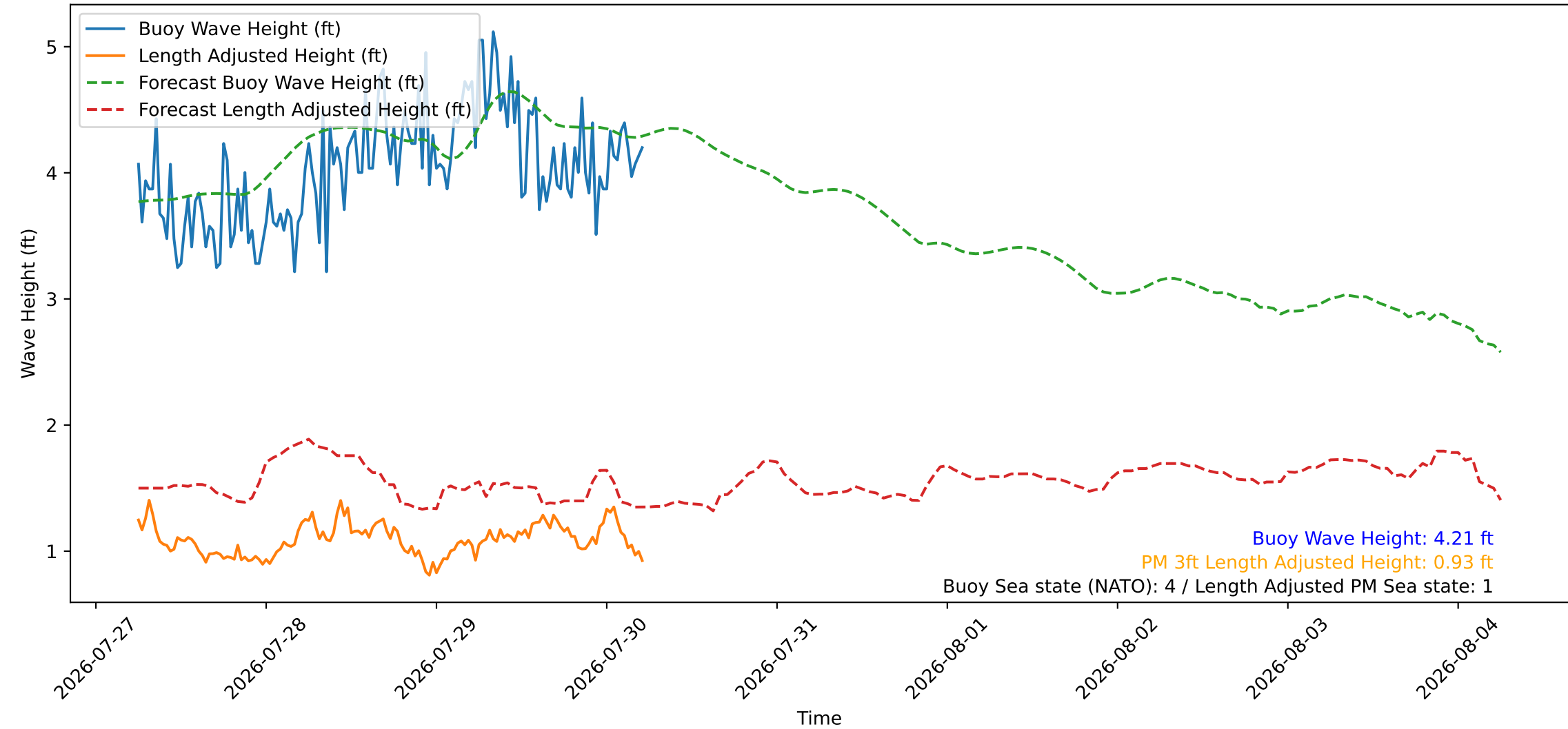
Wave Heights over Time for Red Beach at 2026-07-30 05:40:47
