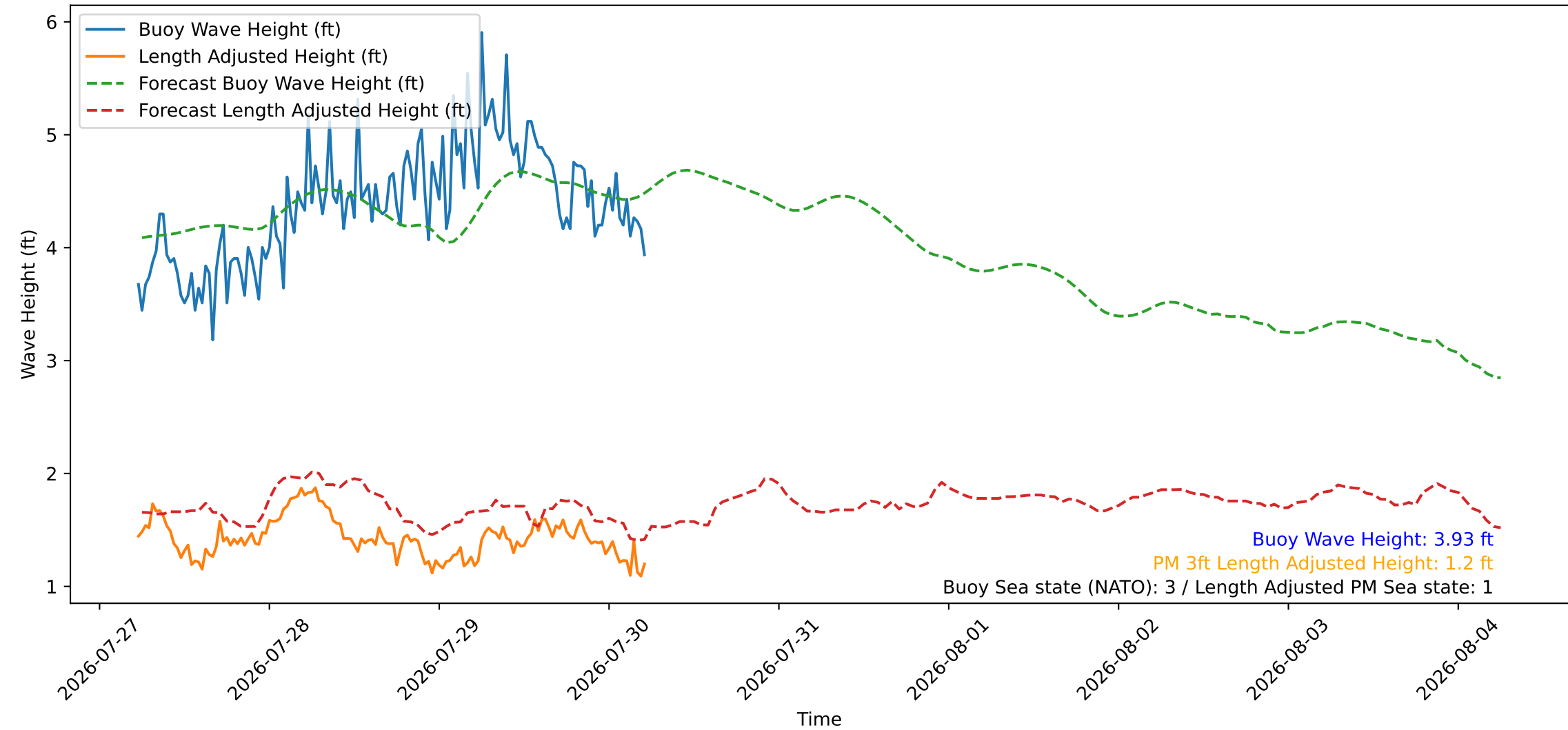
Wave Heights over Time for Oceanside Harbor at 2026-07-30 05:40:27
