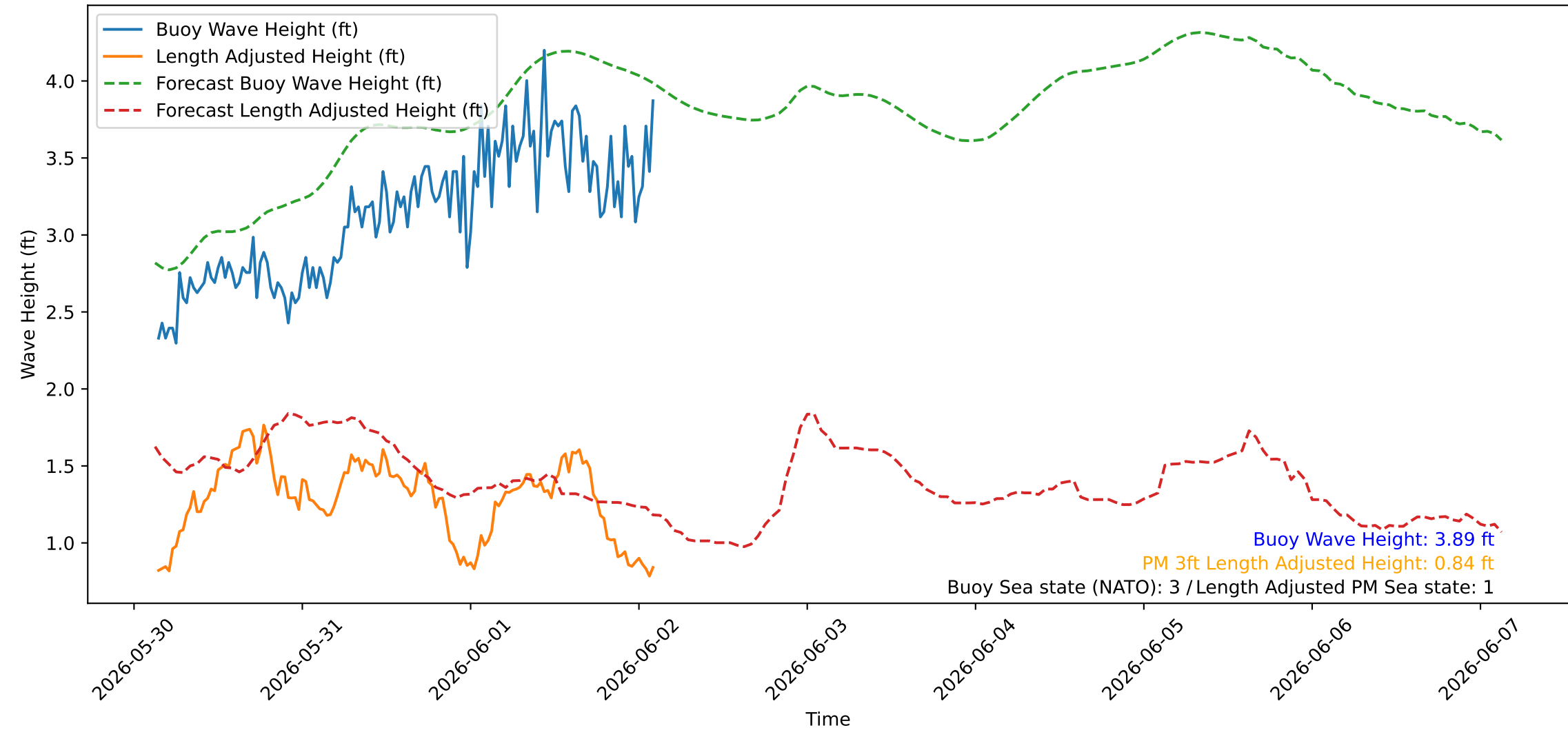
Wave Heights over Time for Red Beach at 2026-06-02 03:10:44
