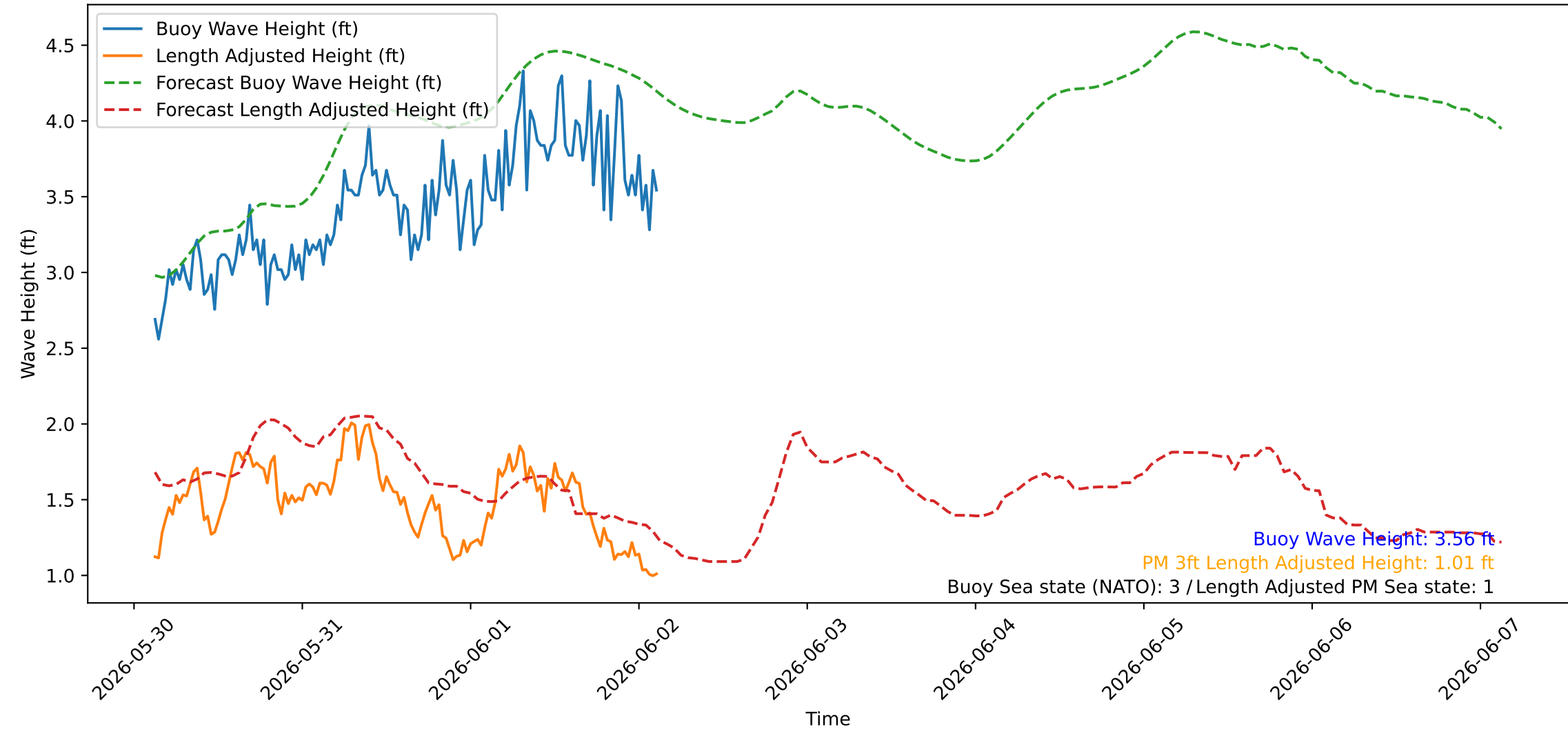
Wave Heights over Time for Green Beach at 2026-06-02 03:11:06
