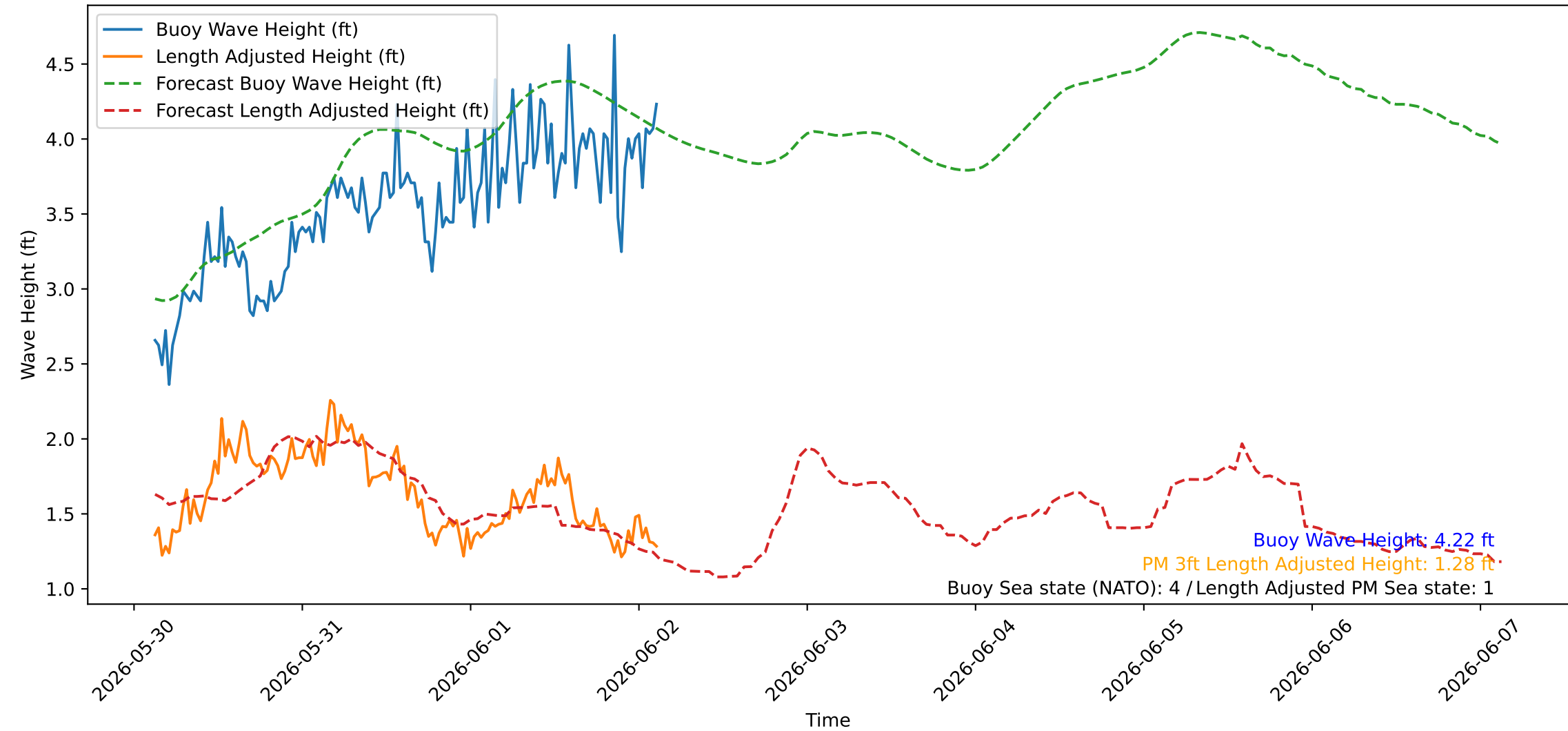
Wave Heights over Time for Oceanside Harbor at 2026-06-02 03:10:25
