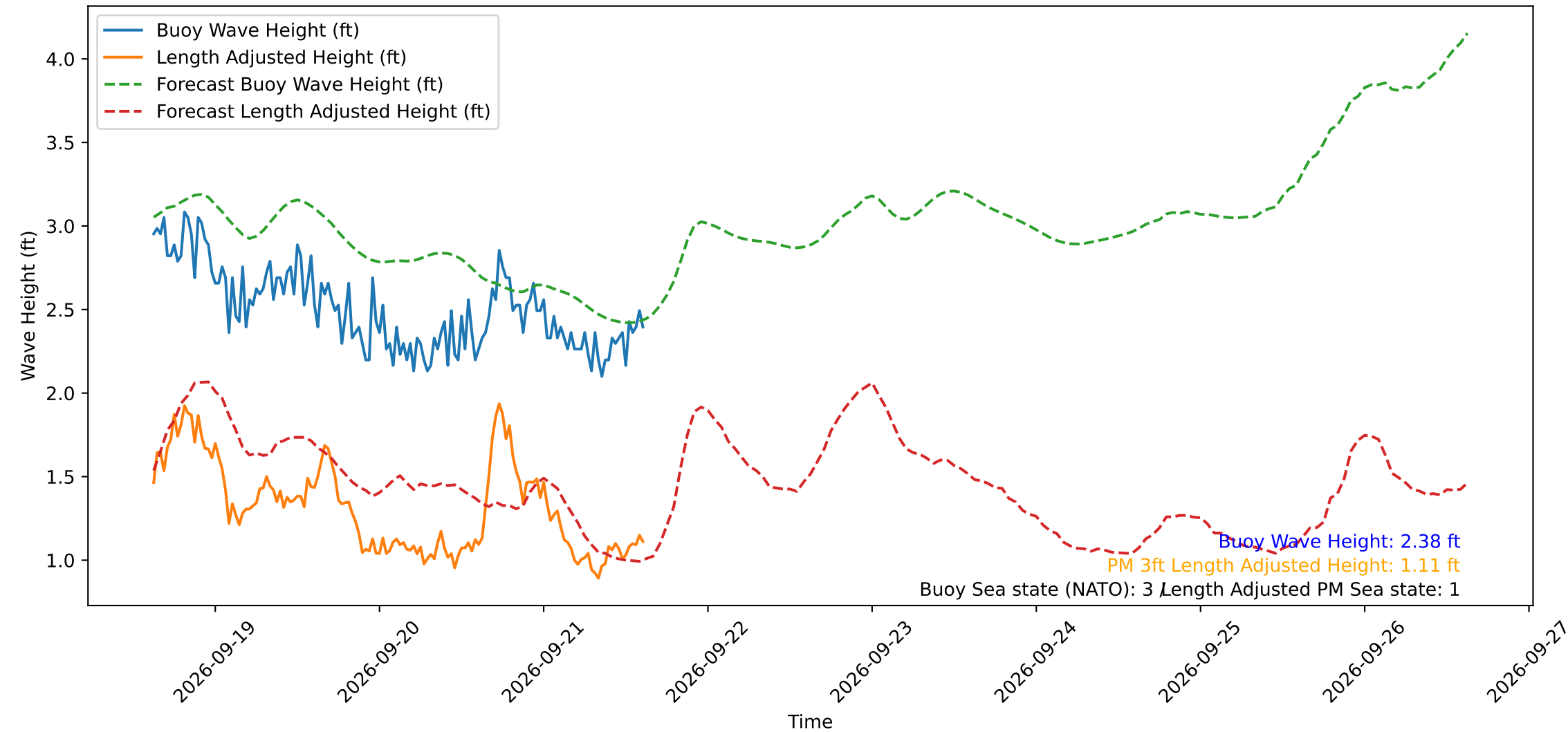
Wave Heights over Time for Oceanside Harbor at 2026-09-21 15:10:29
