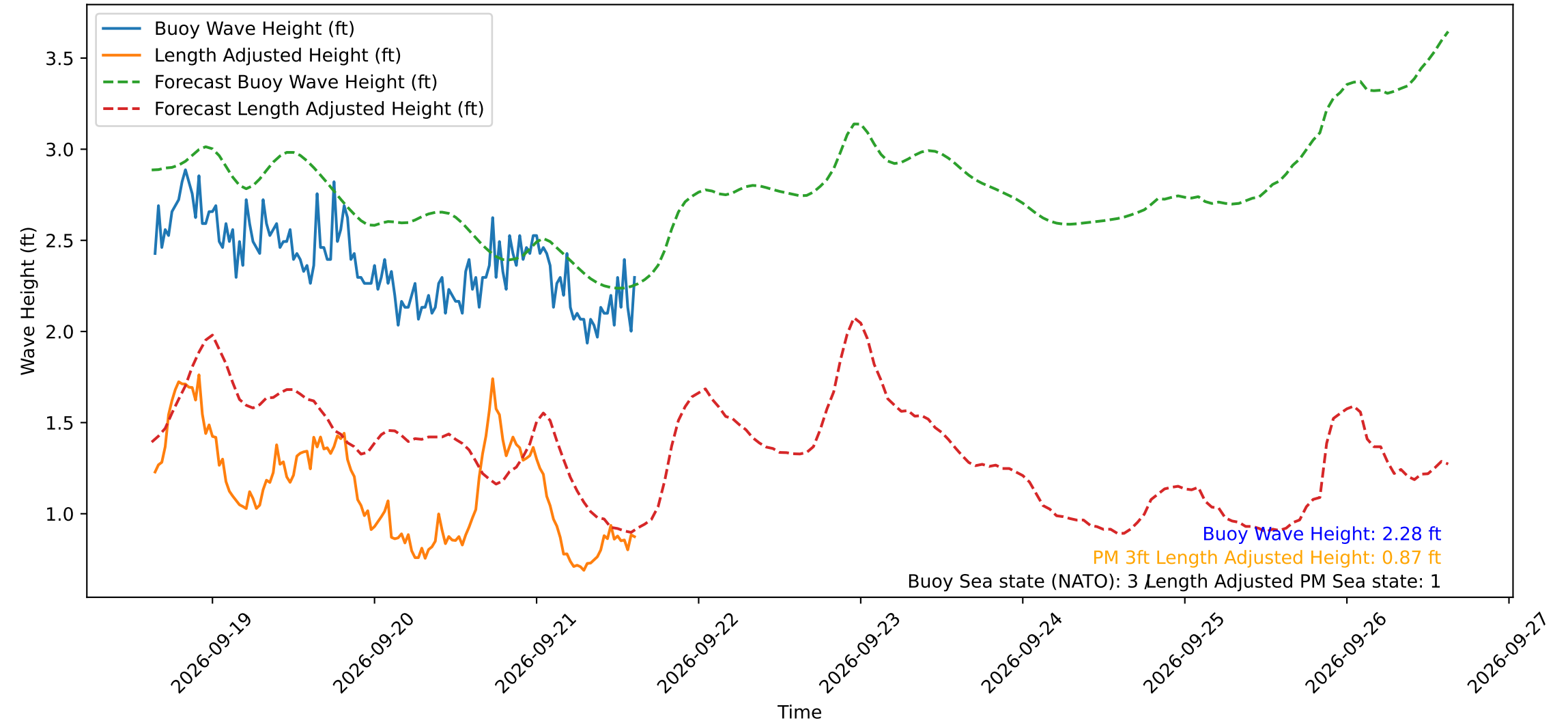
Wave Heights over Time for Red Beach at 2026-09-21 15:10:49
