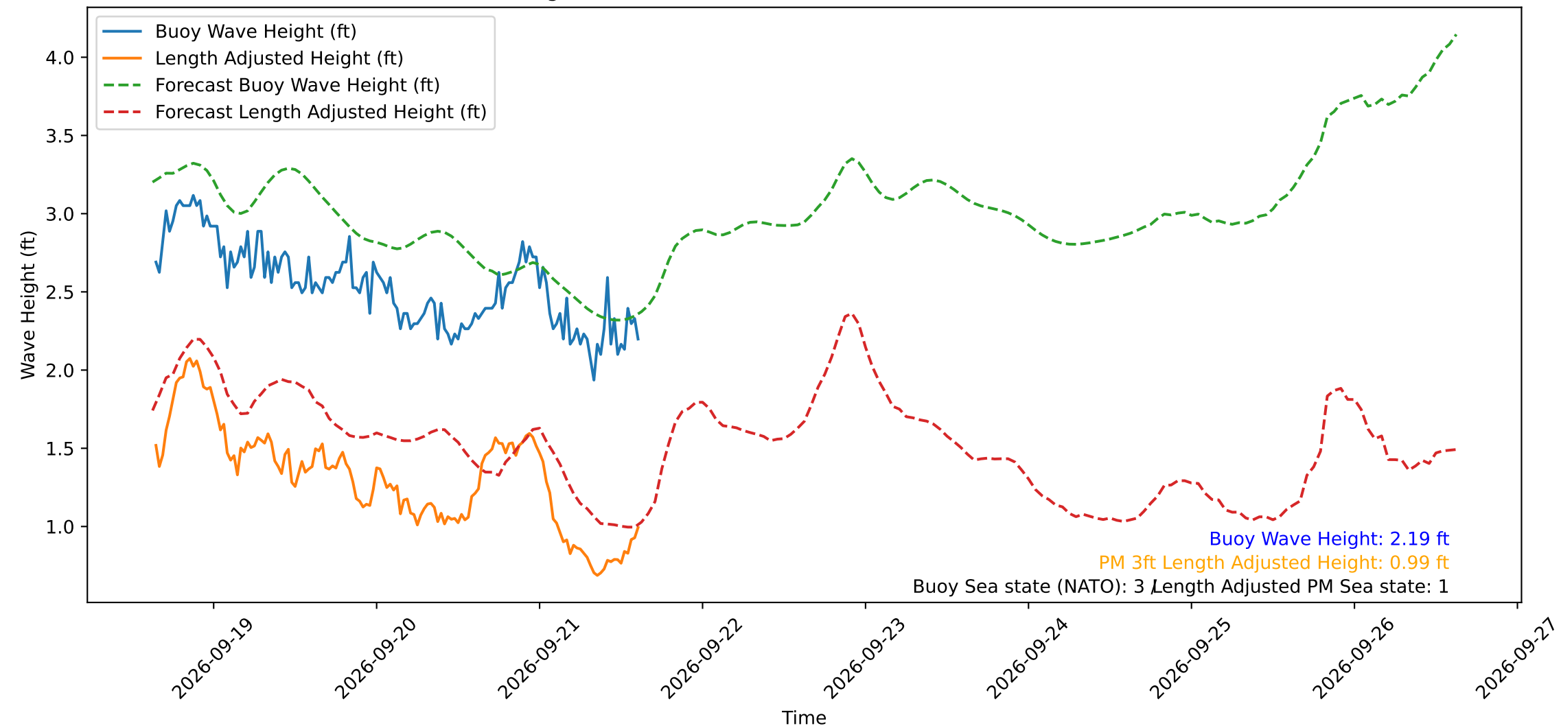
Wave Heights over Time for Green Beach at 2026-09-21 15:11:12
