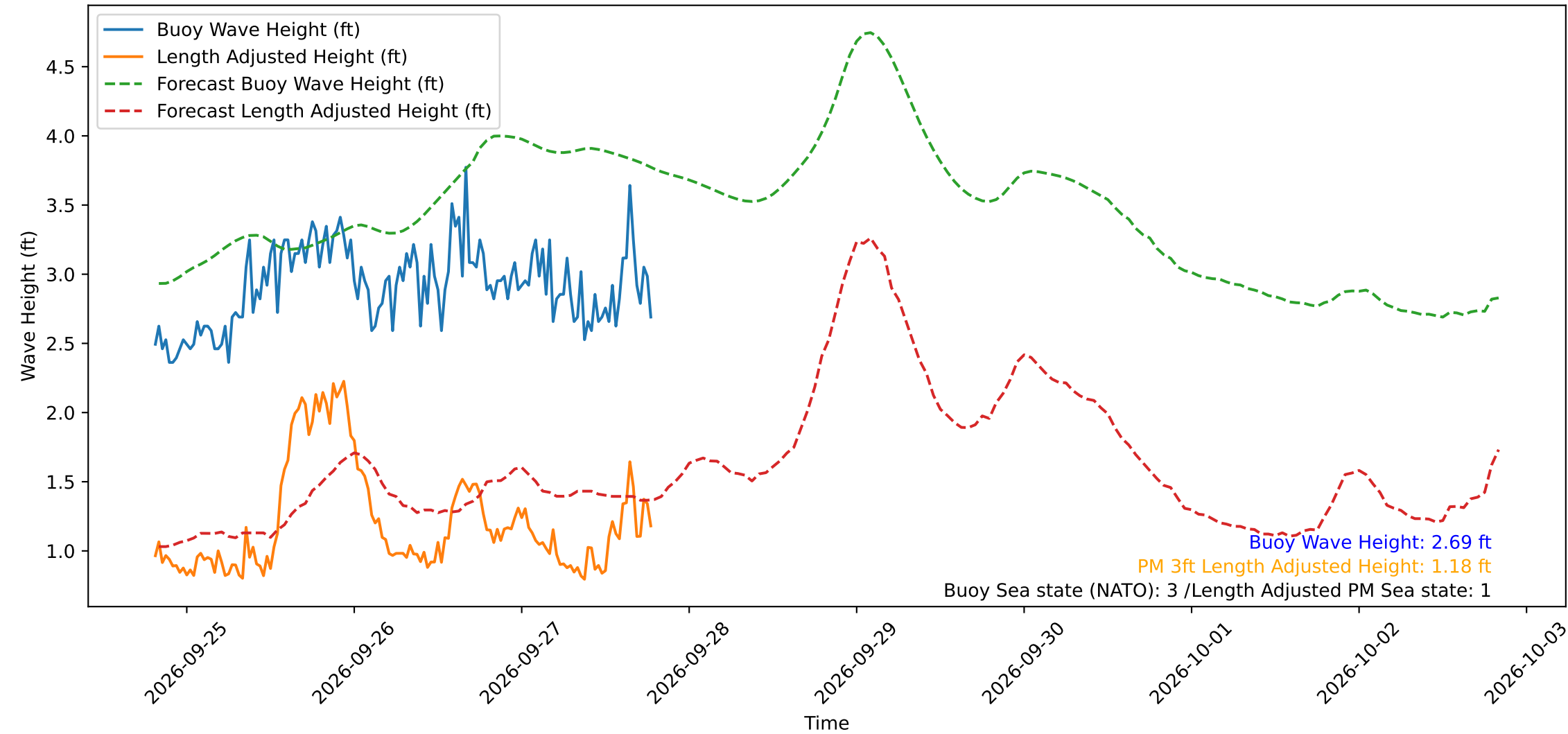
Wave Heights over Time for Oceanside Harbor at 2026-09-27 19:30:31
