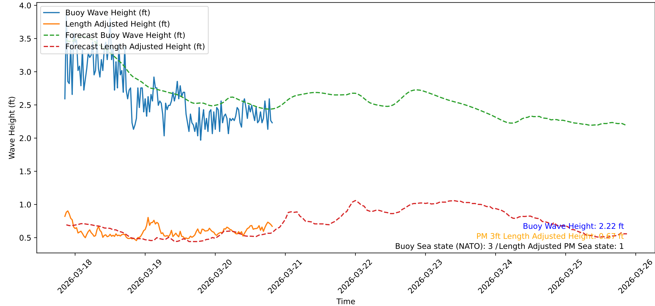
Wave Heights over Time for Oceanside Harbor at 2026-03-20 20:40:31
