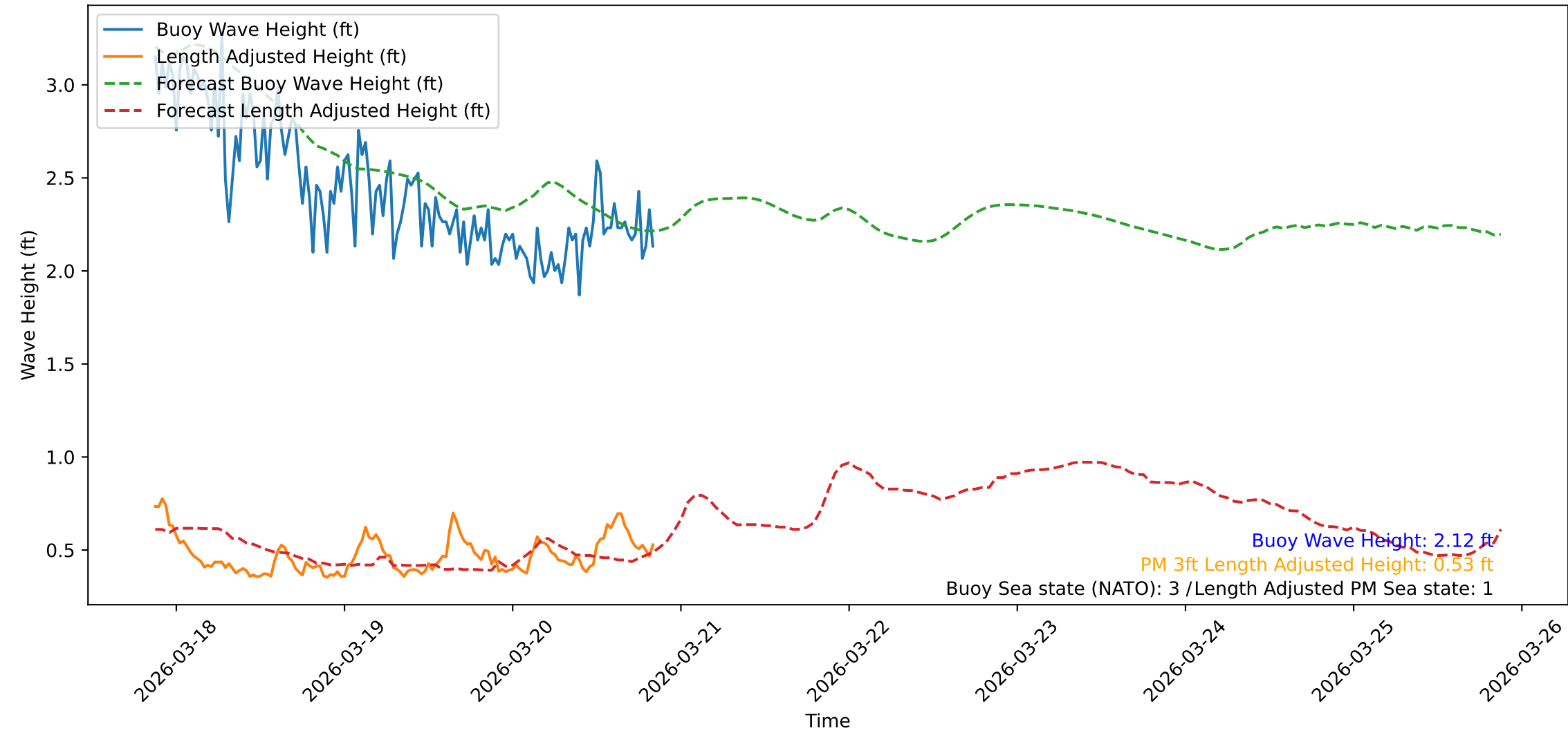
Wave Heights over Time for Red Beach at 2026-03-20 20:40:48
