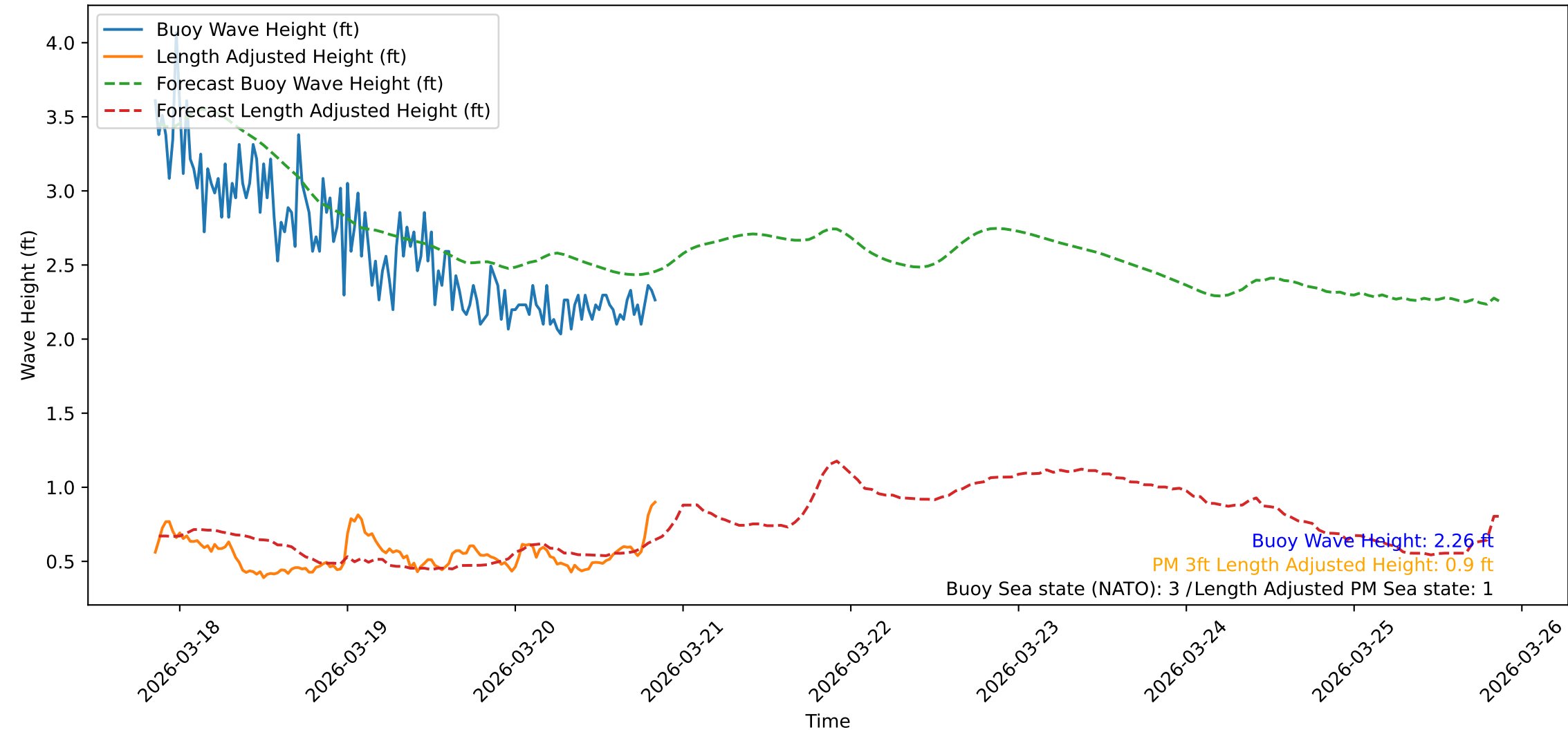
Wave Heights over Time for Green Beach at 2026-03-20 20:41:10
