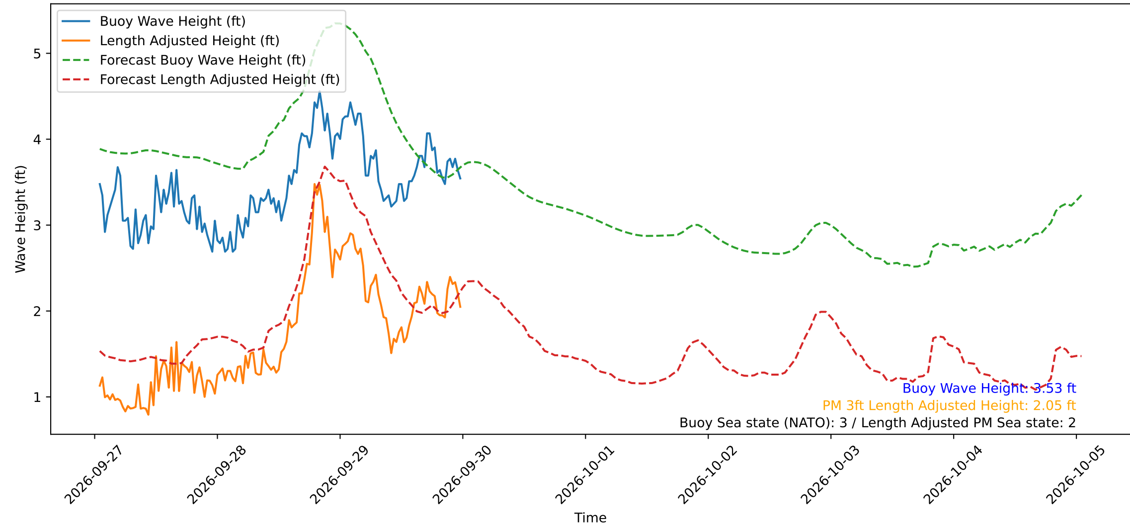
Wave Heights over Time for Green Beach at 2026-09-30 00:31:12
