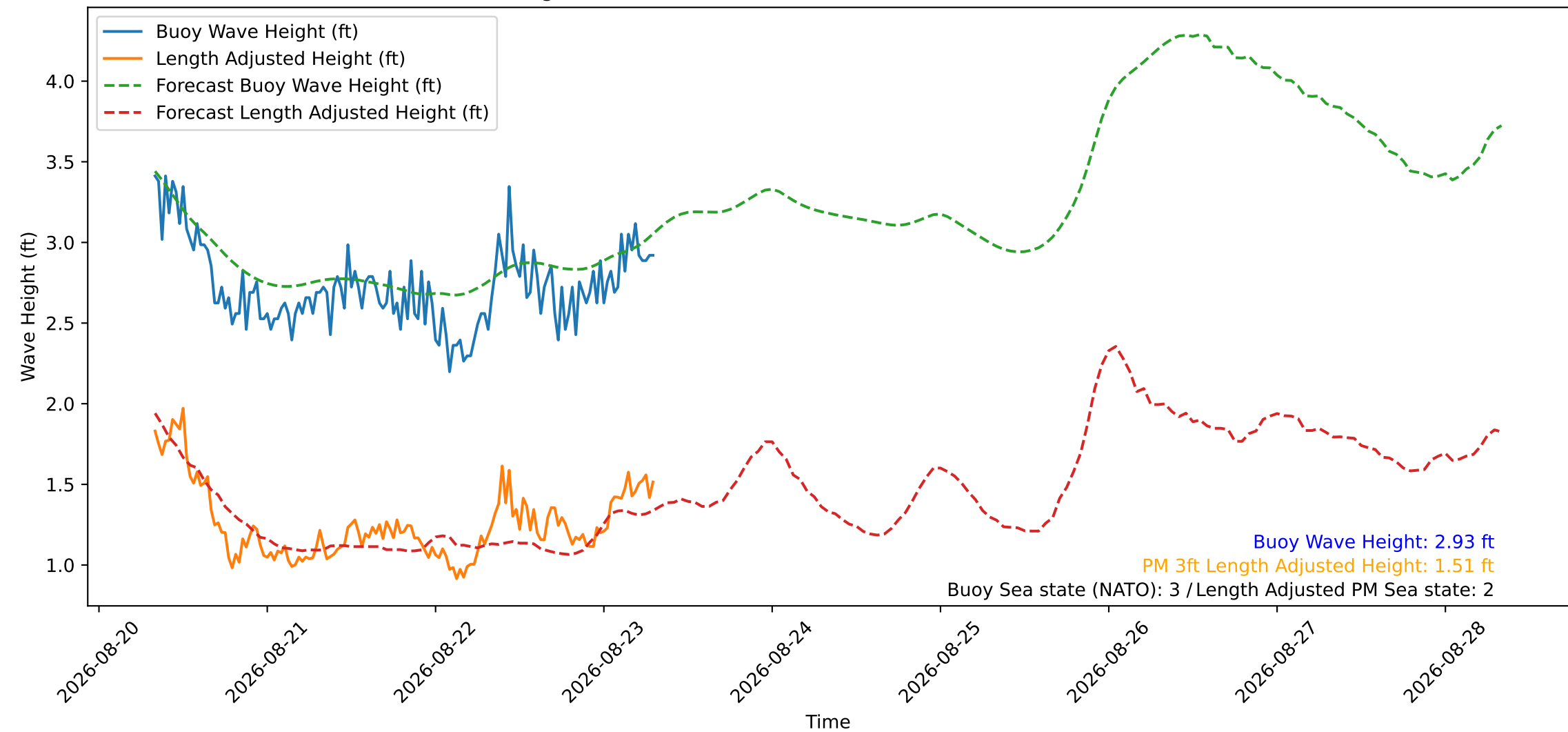
Wave Heights over Time for Oceanside Harbor at 2026-08-23 07:50:30
