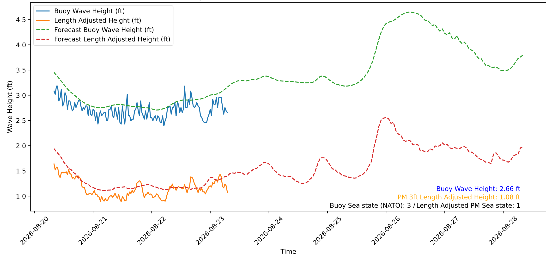
Wave Heights over Time for Green Beach at 2026-08-23 07:51:14
