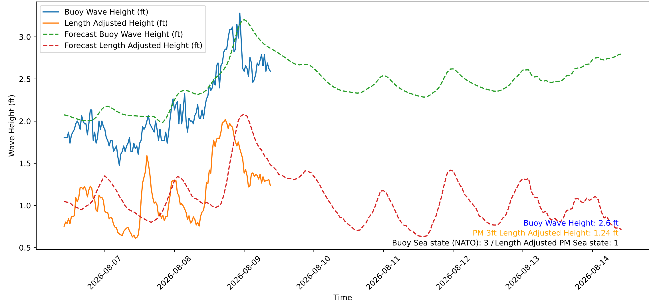
Wave Heights over Time for Red Beach at 2026-08-09 09:50:47
