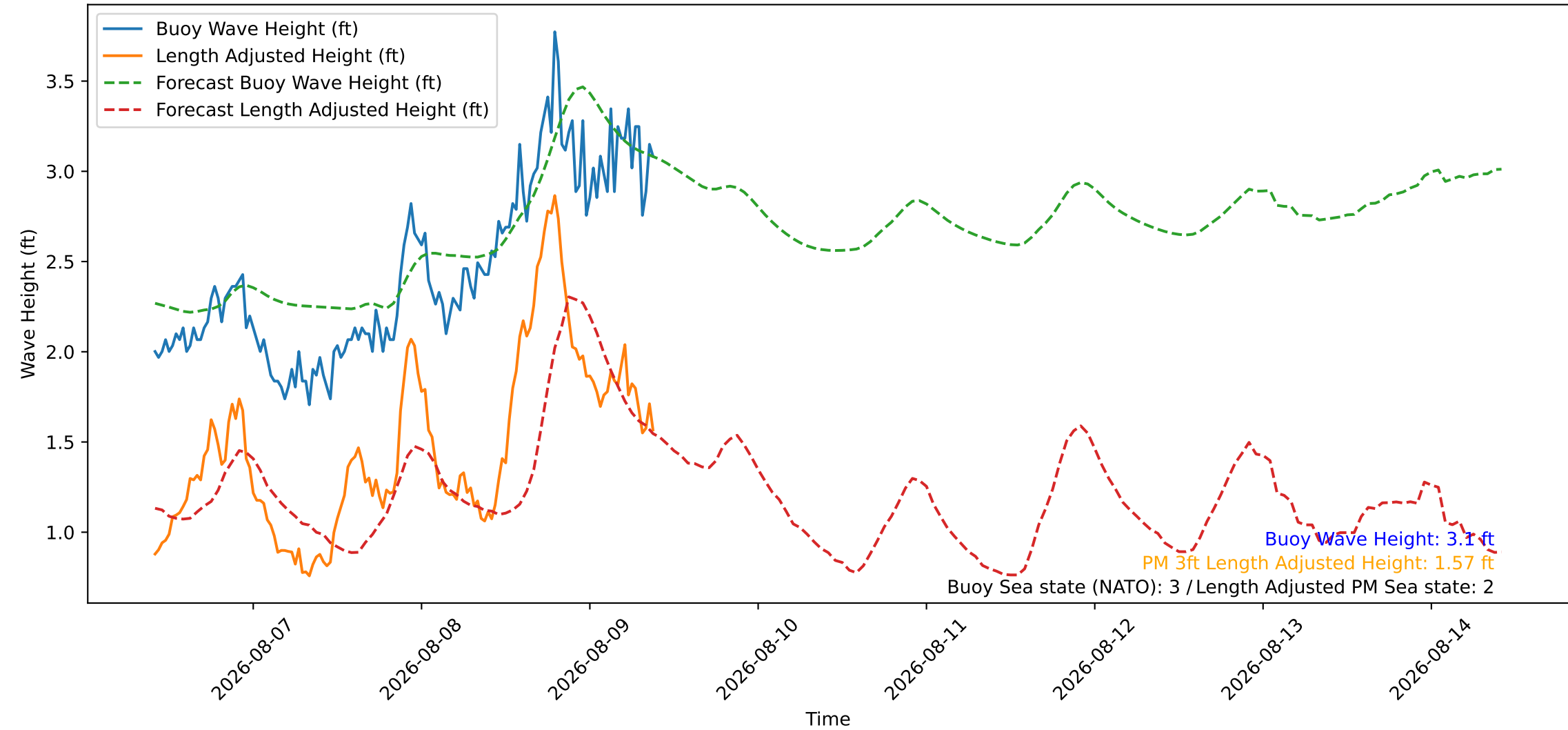
Wave Heights over Time for Green Beach at 2026-08-09 09:51:10
