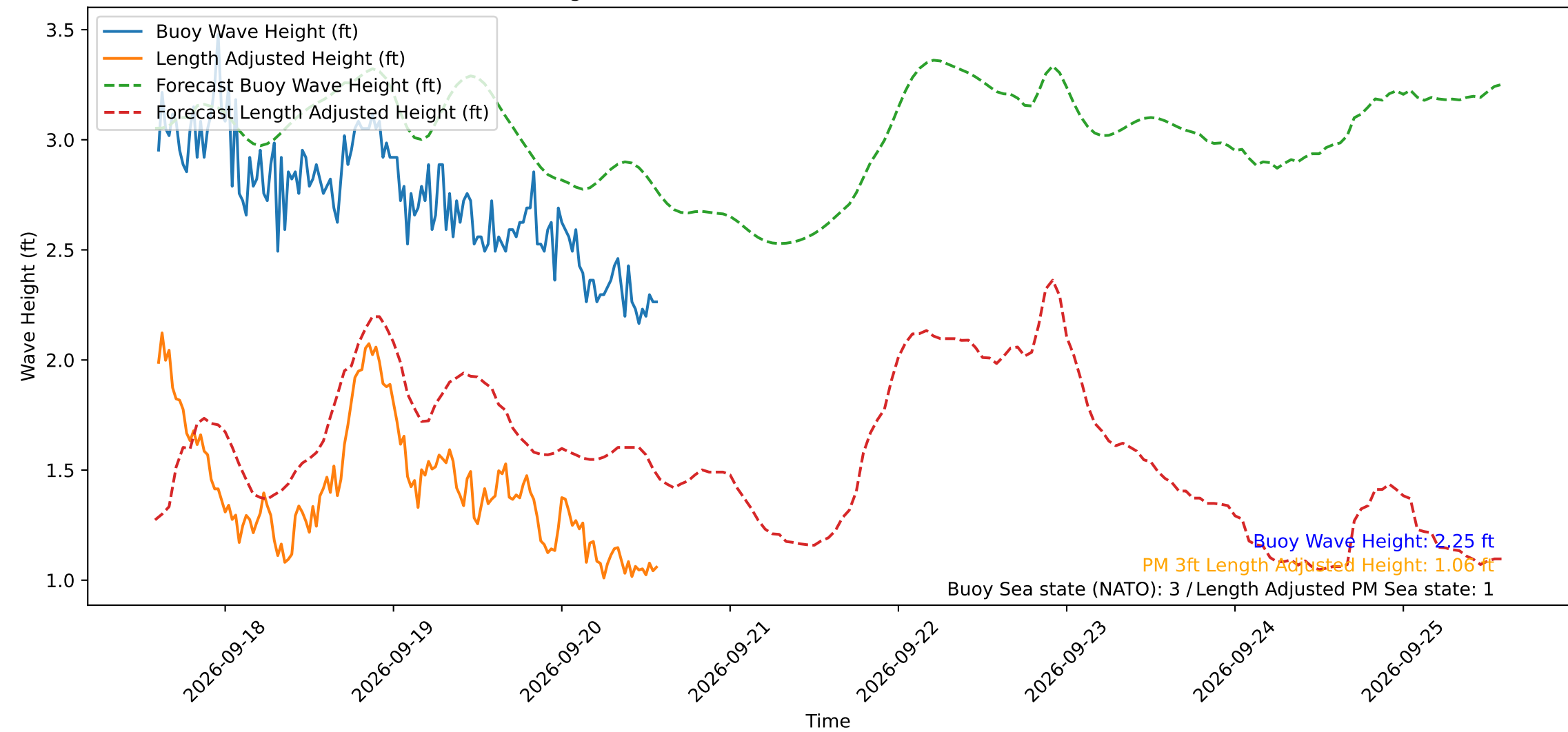
Wave Heights over Time for Green Beach at 2026-09-20 14:21:14
