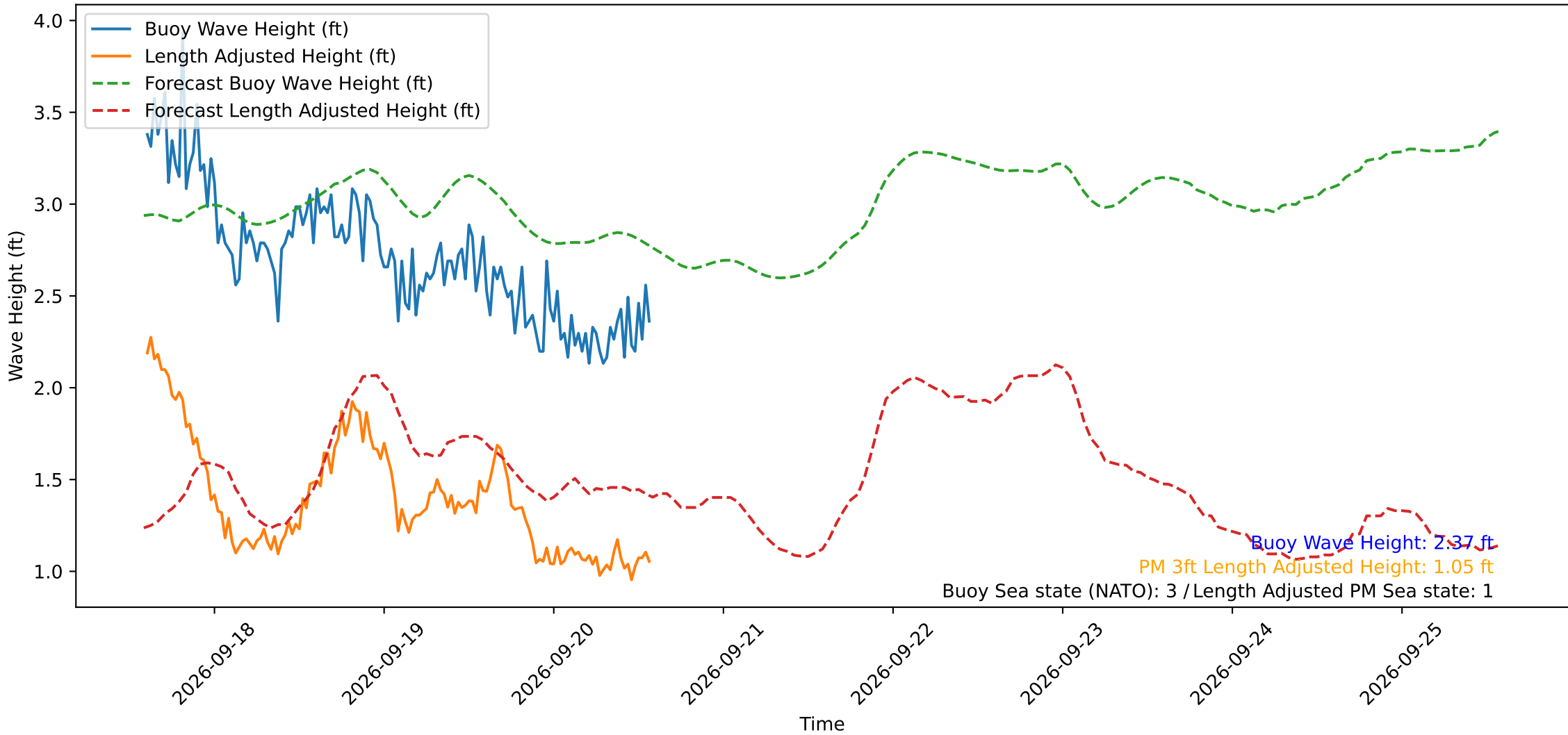
Wave Heights over Time for Oceanside Harbor at 2026-09-20 14:20:29
