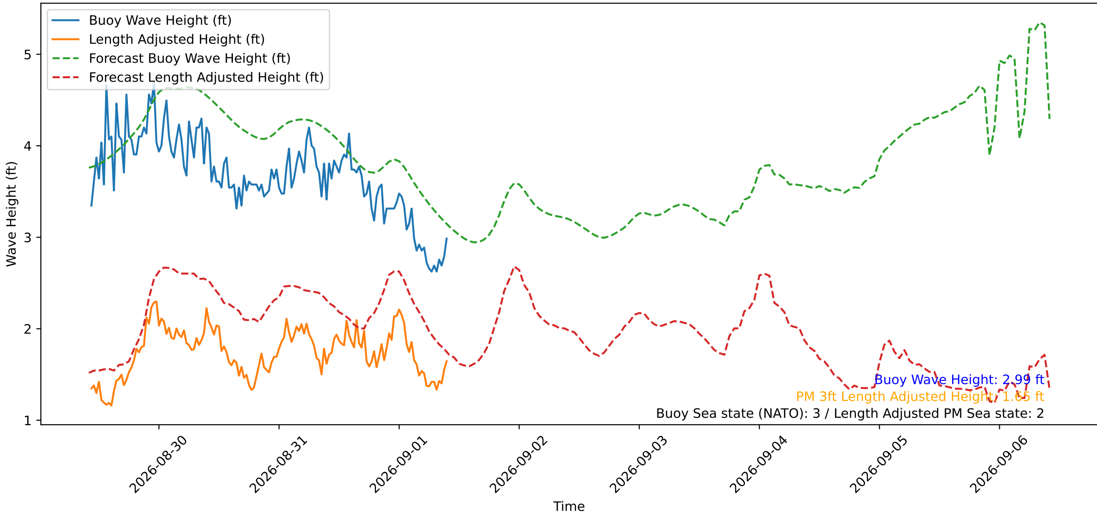
Wave Heights over Time for Red Beach at 2026-09-01 10:20:50
