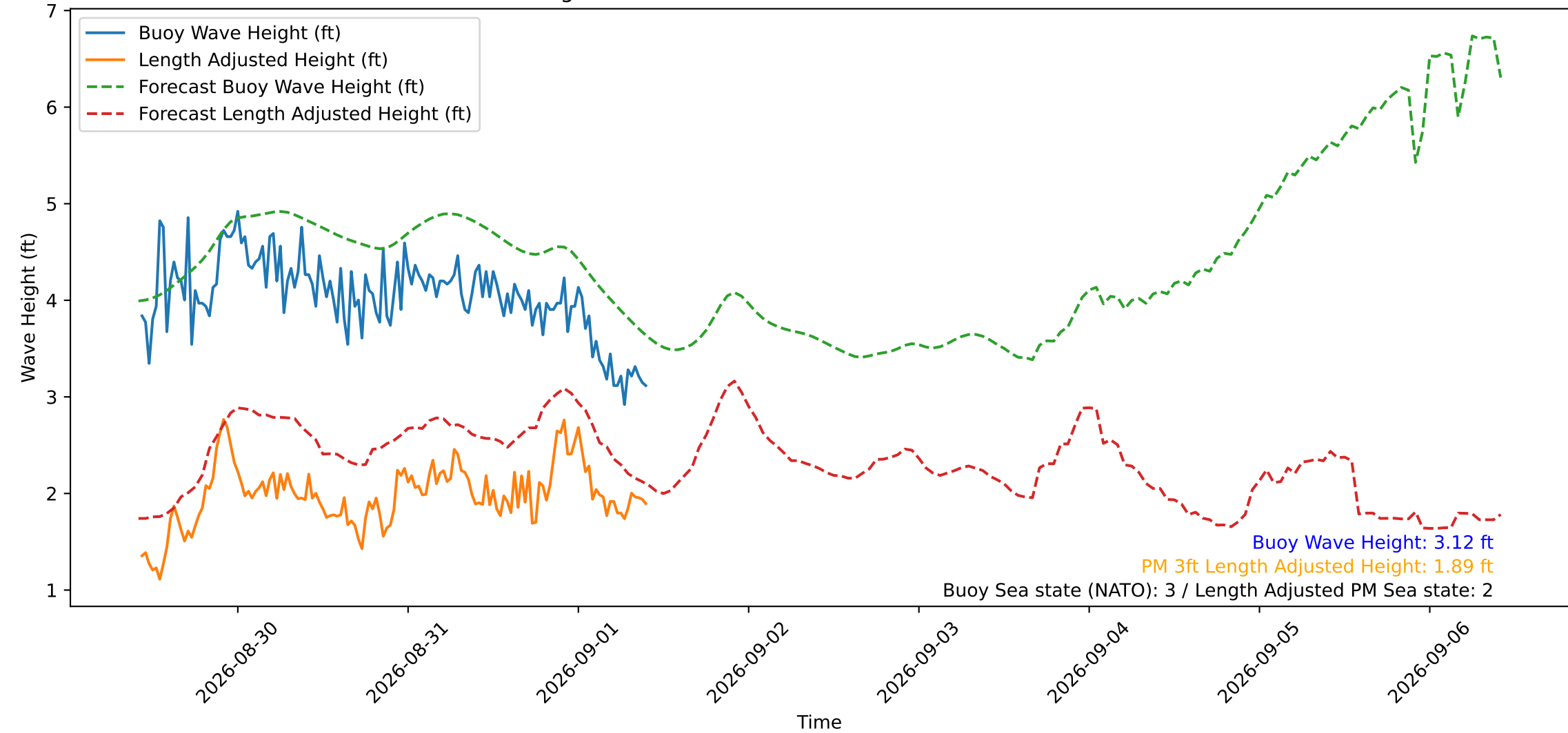
Wave Heights over Time for Green Beach at 2026-09-01 10:21:14
