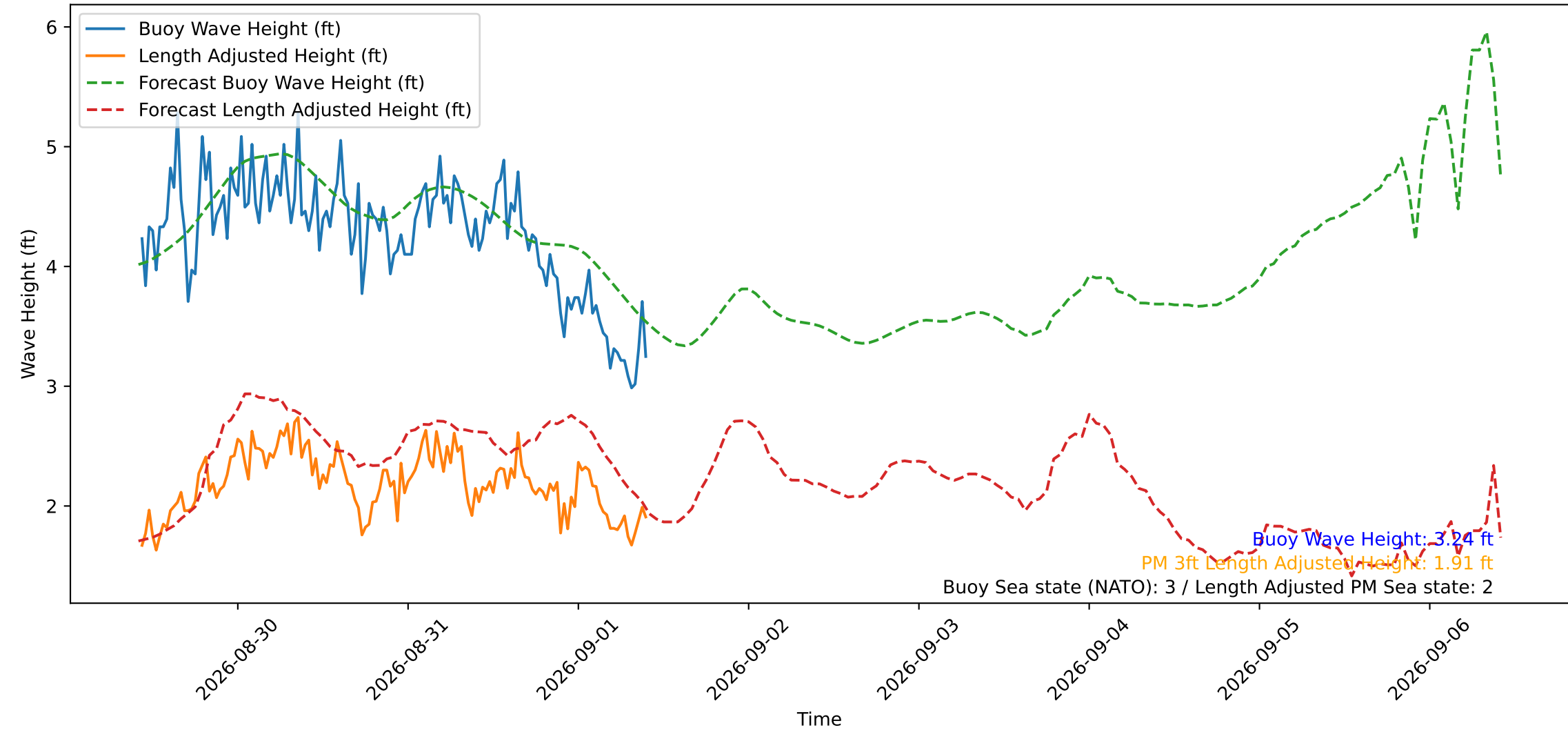
Wave Heights over Time for Oceanside Harbor at 2026-09-01 10:20:29
