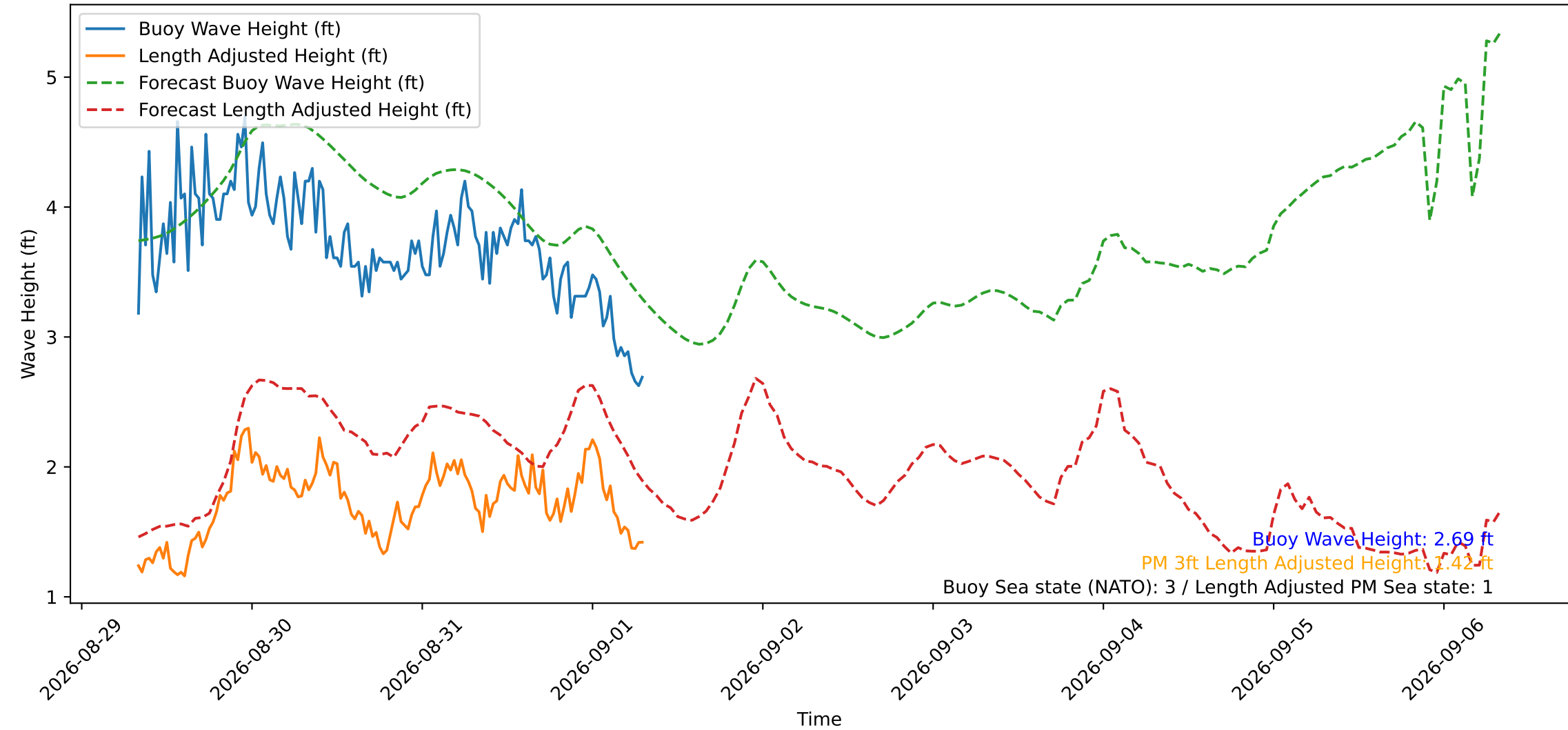
Wave Heights over Time for Red Beach at 2026-09-01 07:50:49
