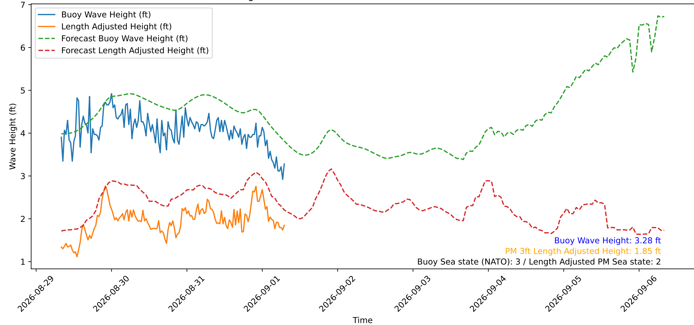
Wave Heights over Time for Green Beach at 2026-09-01 07:51:13
