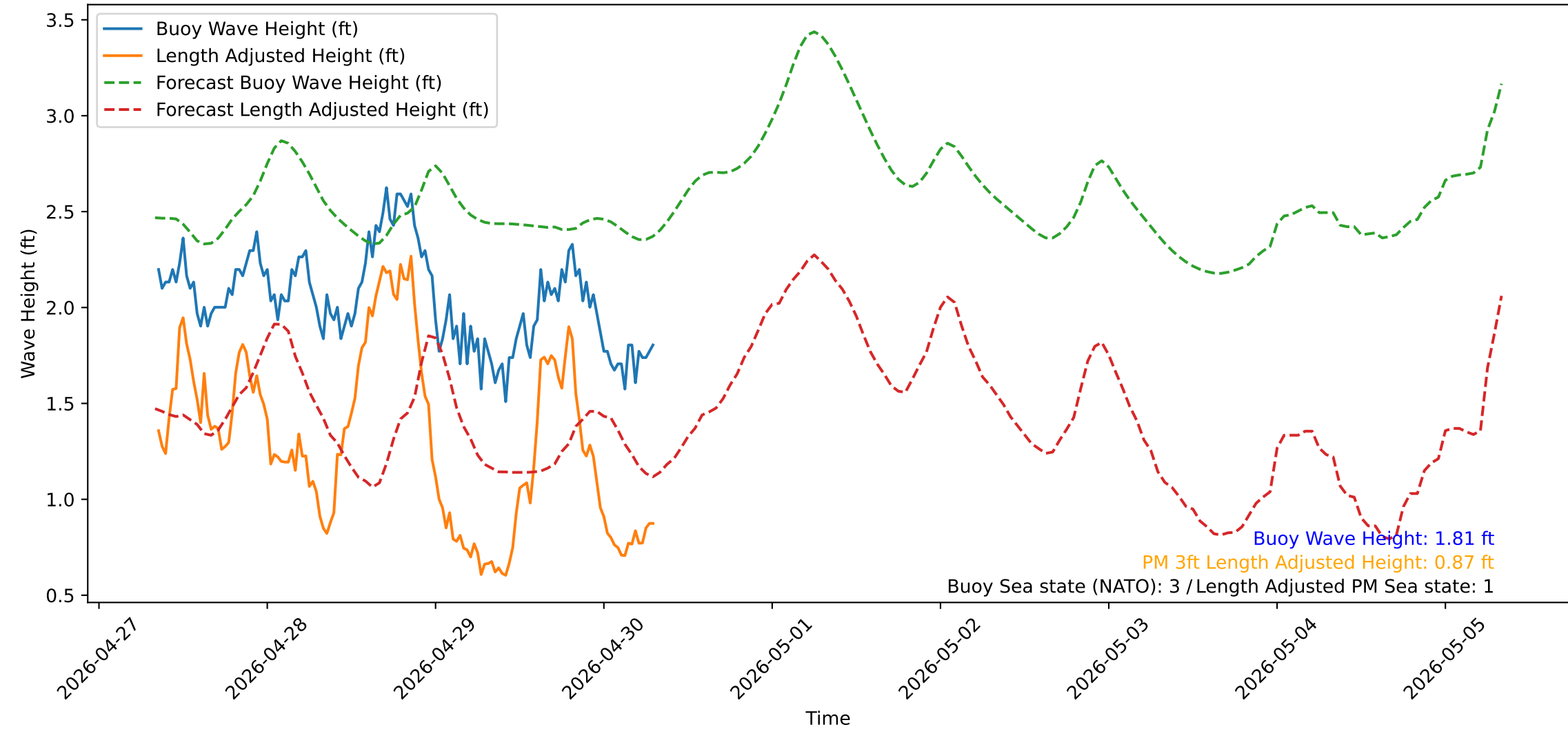
Wave Heights over Time for Red Beach at 2026-04-30 08:00:50
