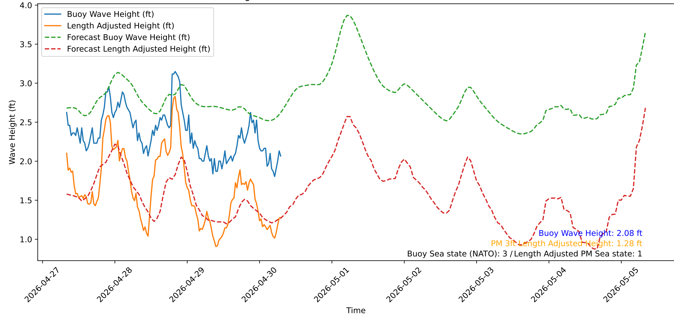
Wave Heights over Time for Green Beach at 2026-04-30 08:01:12
