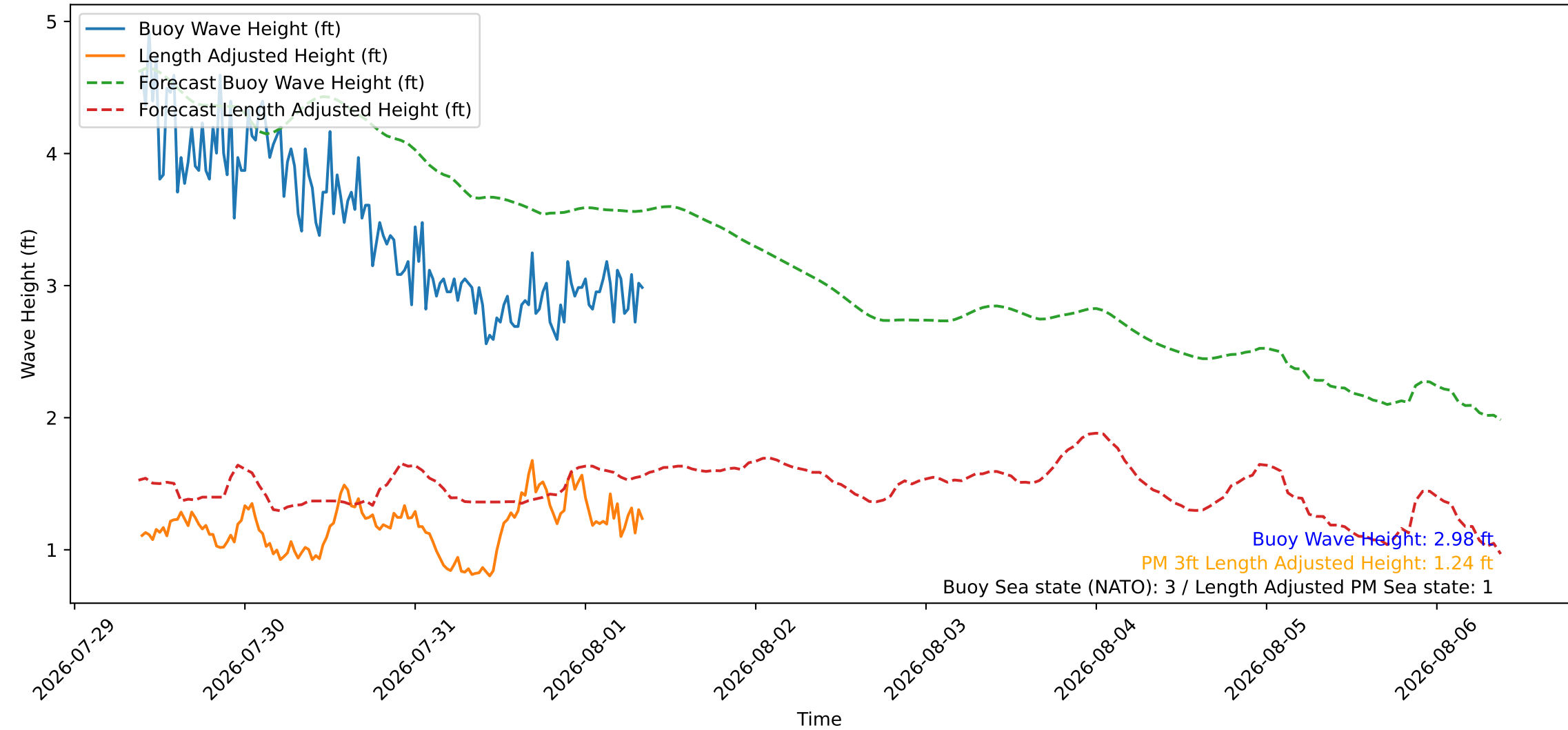
Wave Heights over Time for Red Beach at 2026-08-01 09:00:46
