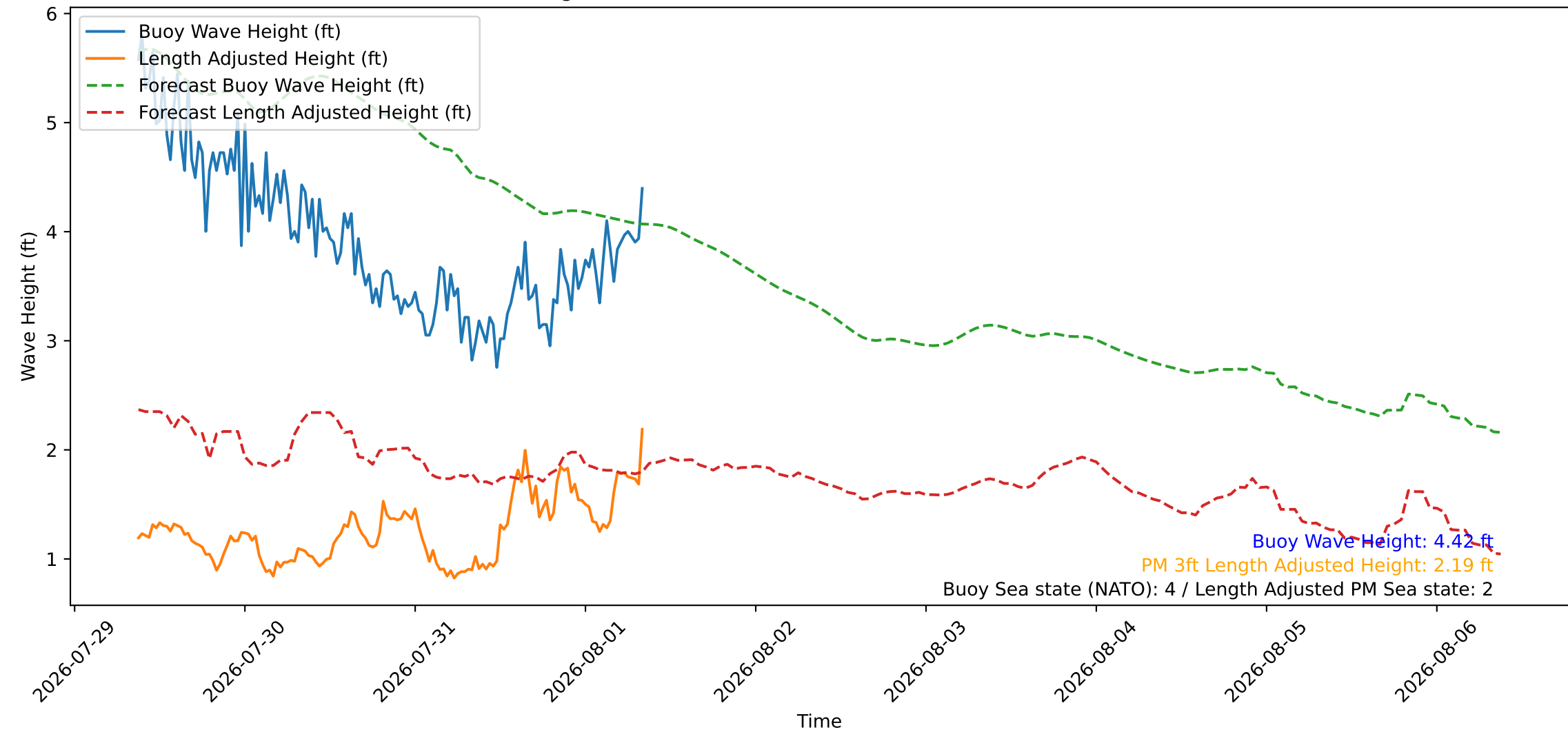
Wave Heights over Time for Green Beach at 2026-08-01 09:01:08
