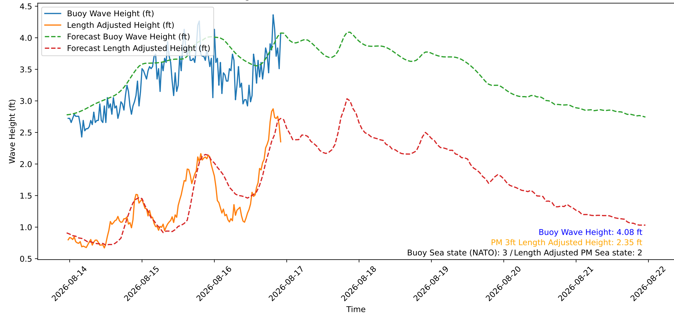
Wave Heights over Time for Green Beach at 2026-08-16 23:01:08
