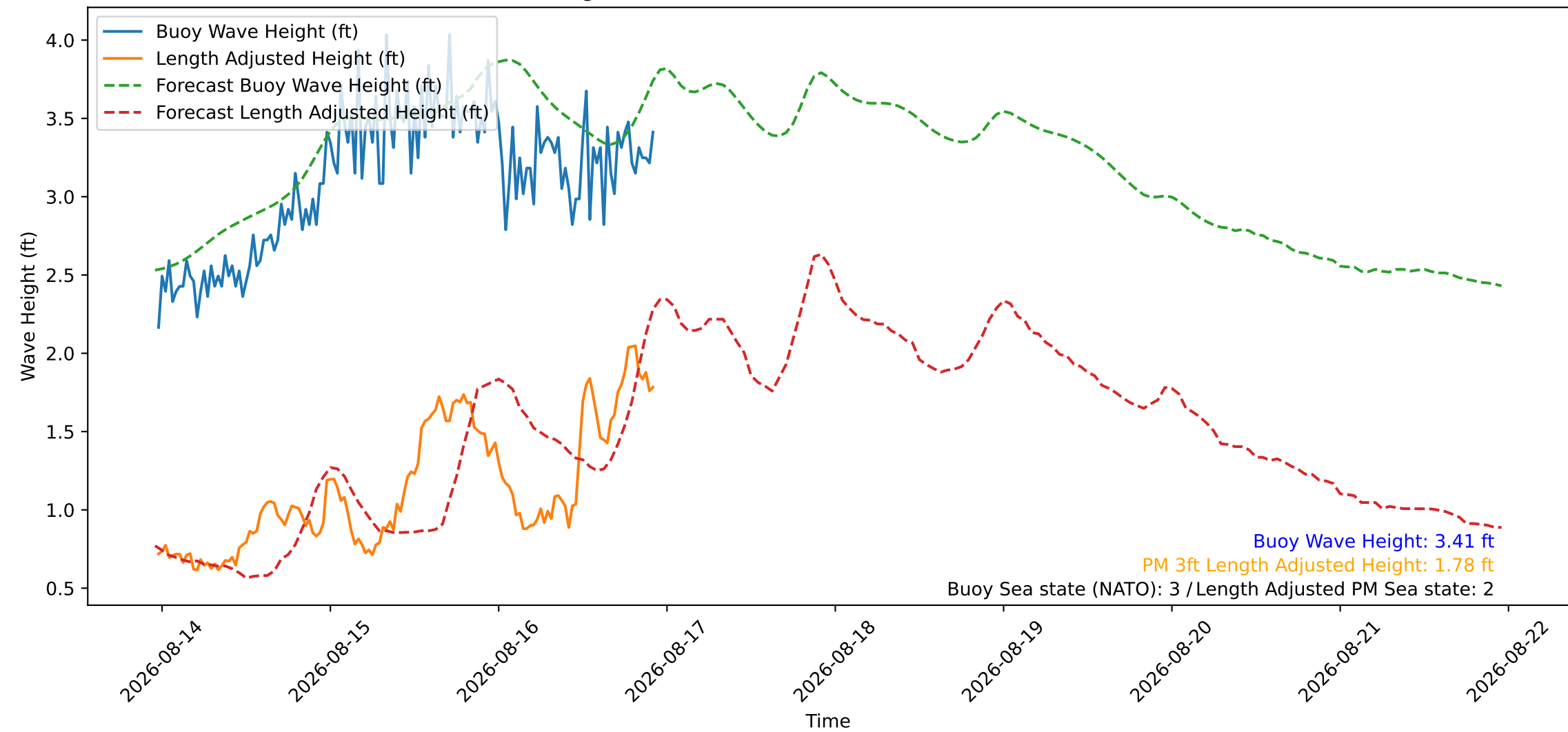
Wave Heights over Time for Red Beach at 2026-08-16 23:00:46
