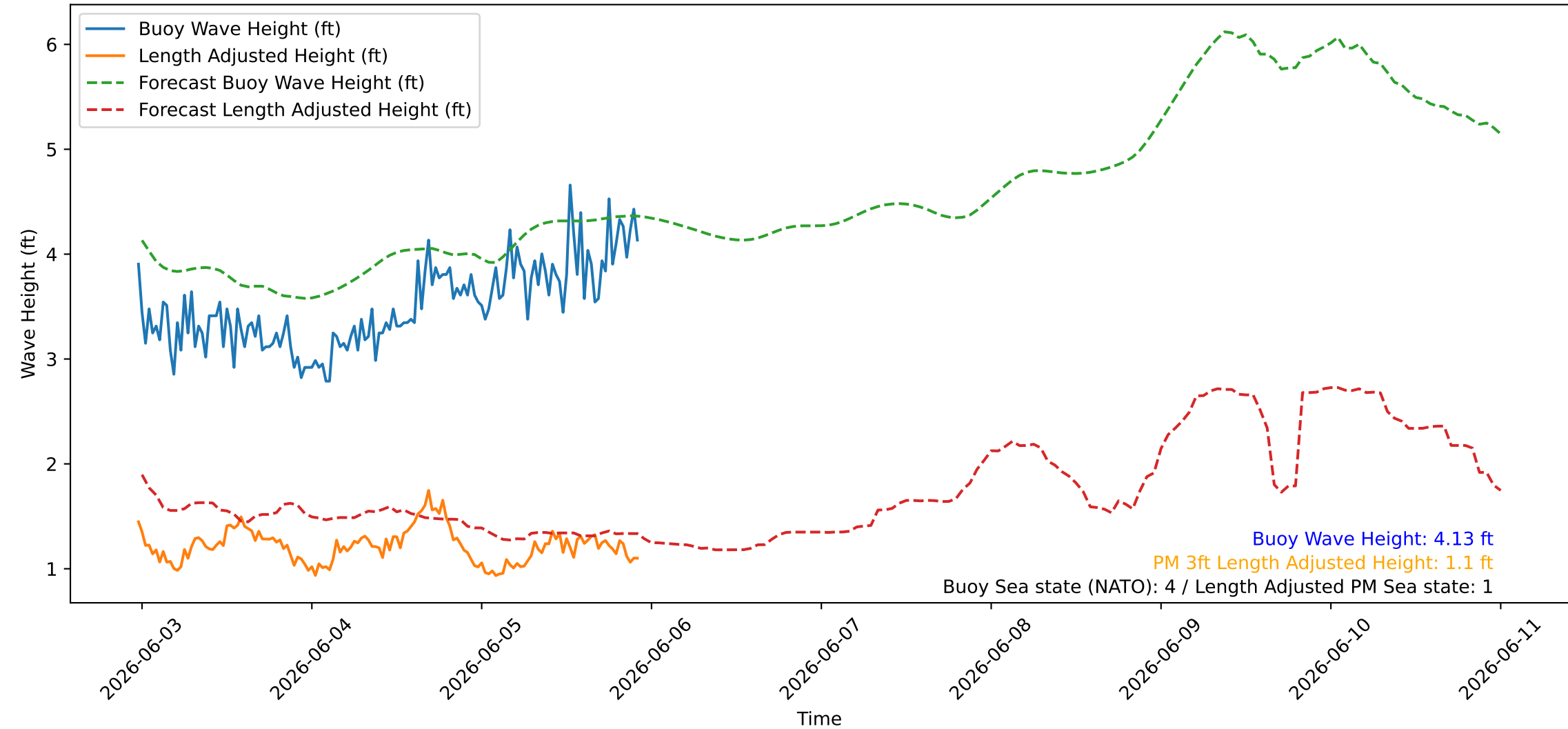
Wave Heights over Time for Green Beach at 2026-06-05 23:31:08
