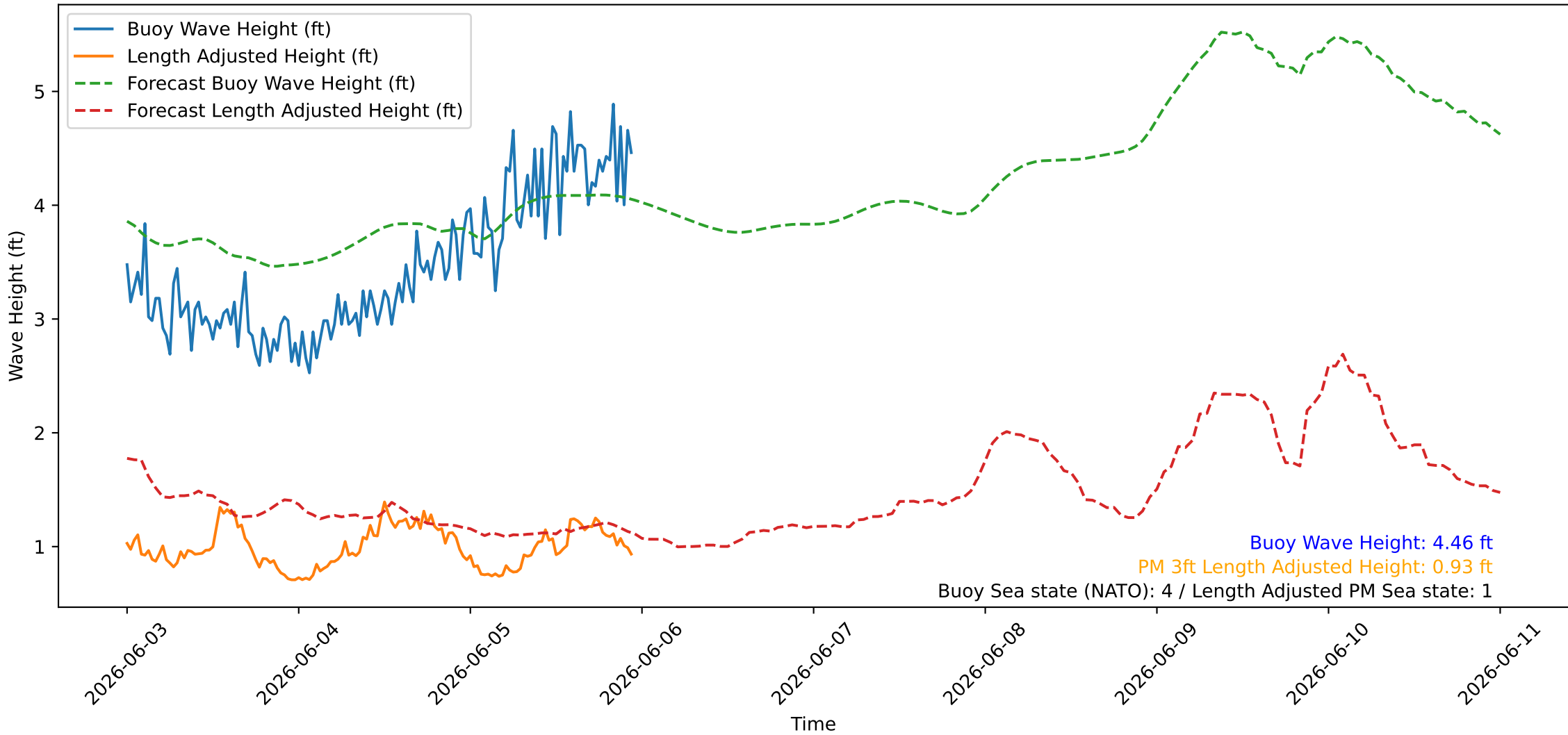
Wave Heights over Time for Red Beach at 2026-06-05 23:30:45
