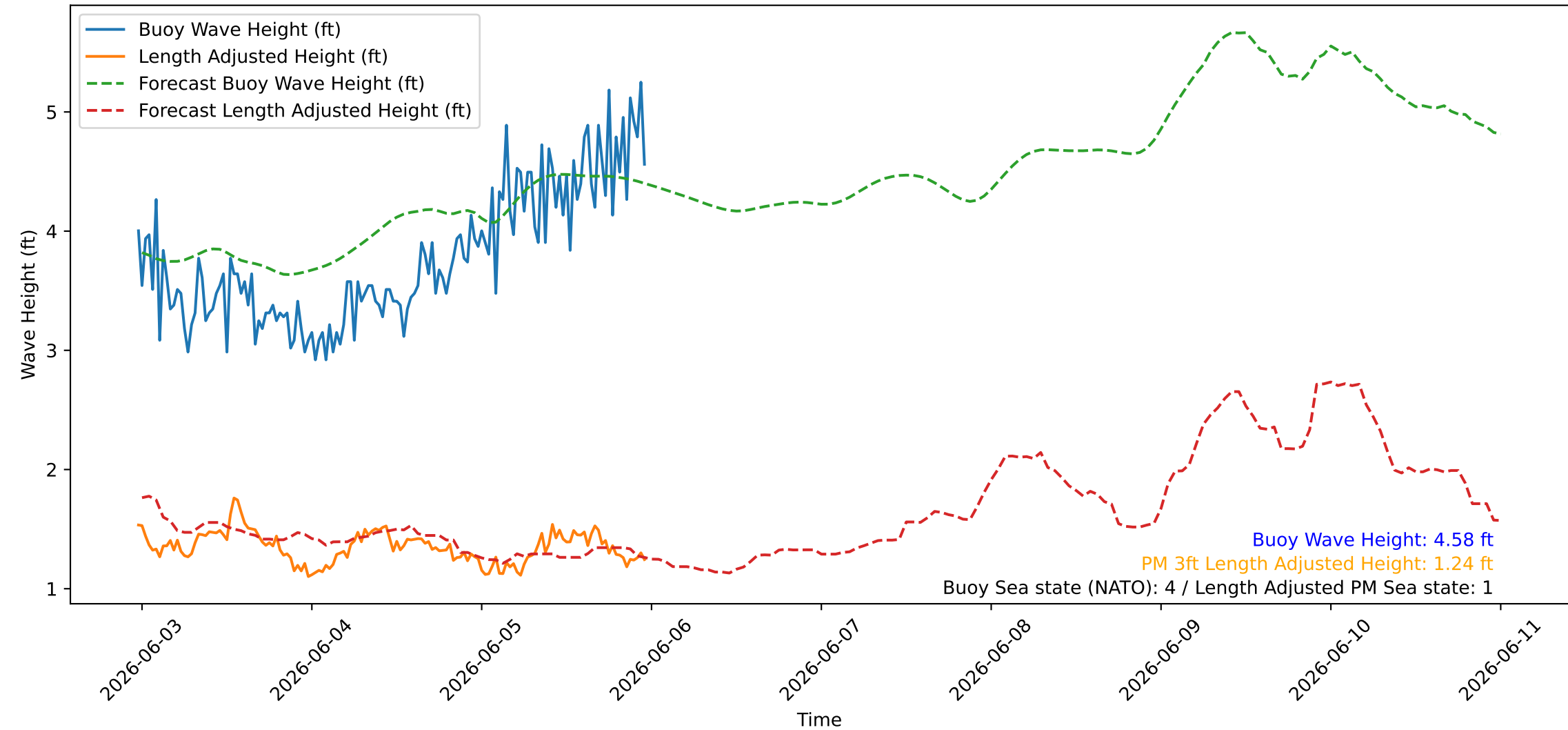
Wave Heights over Time for Oceanside Harbor at 2026-06-05 23:30:26
