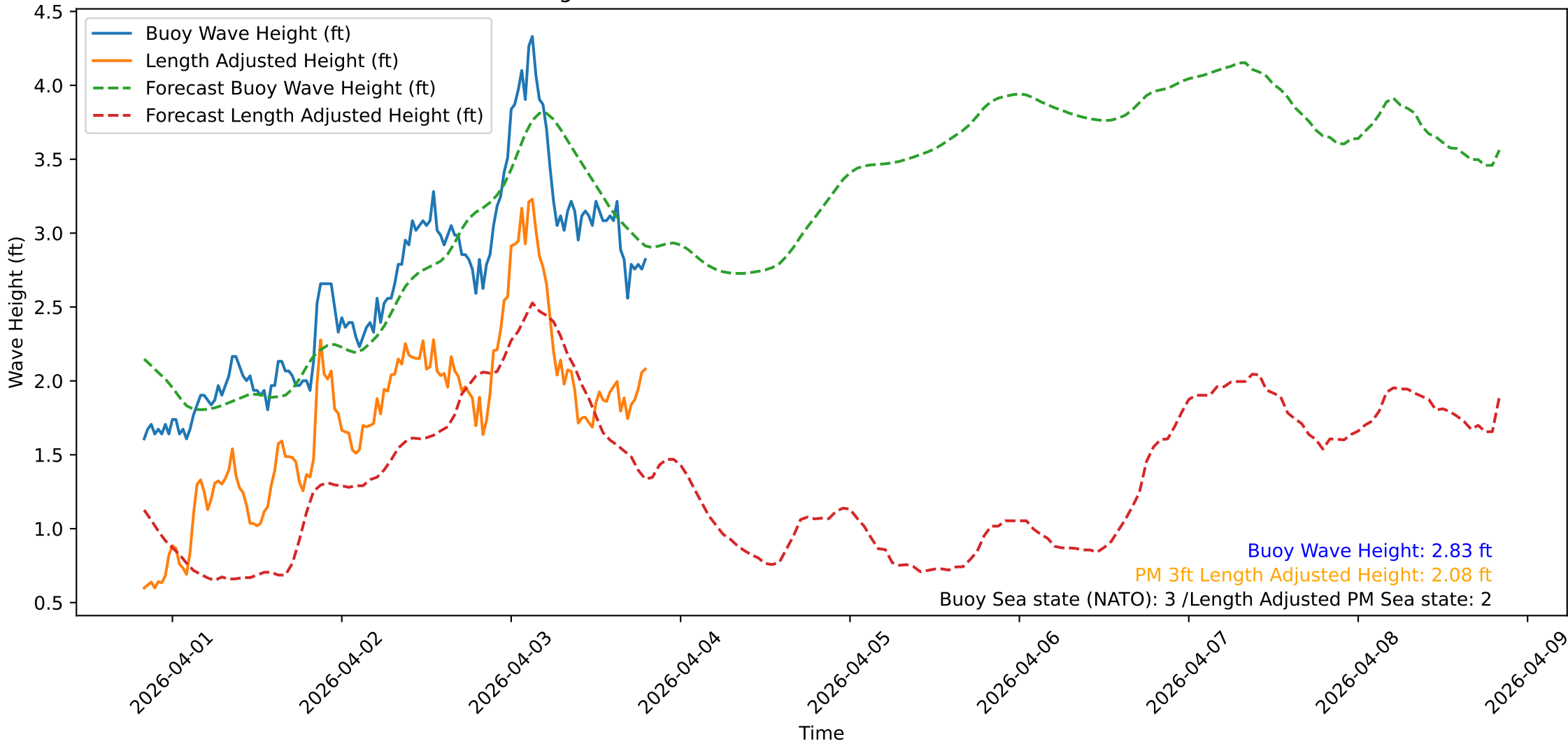
Wave Heights over Time for Green Beach at 2026-04-03 19:51:30
