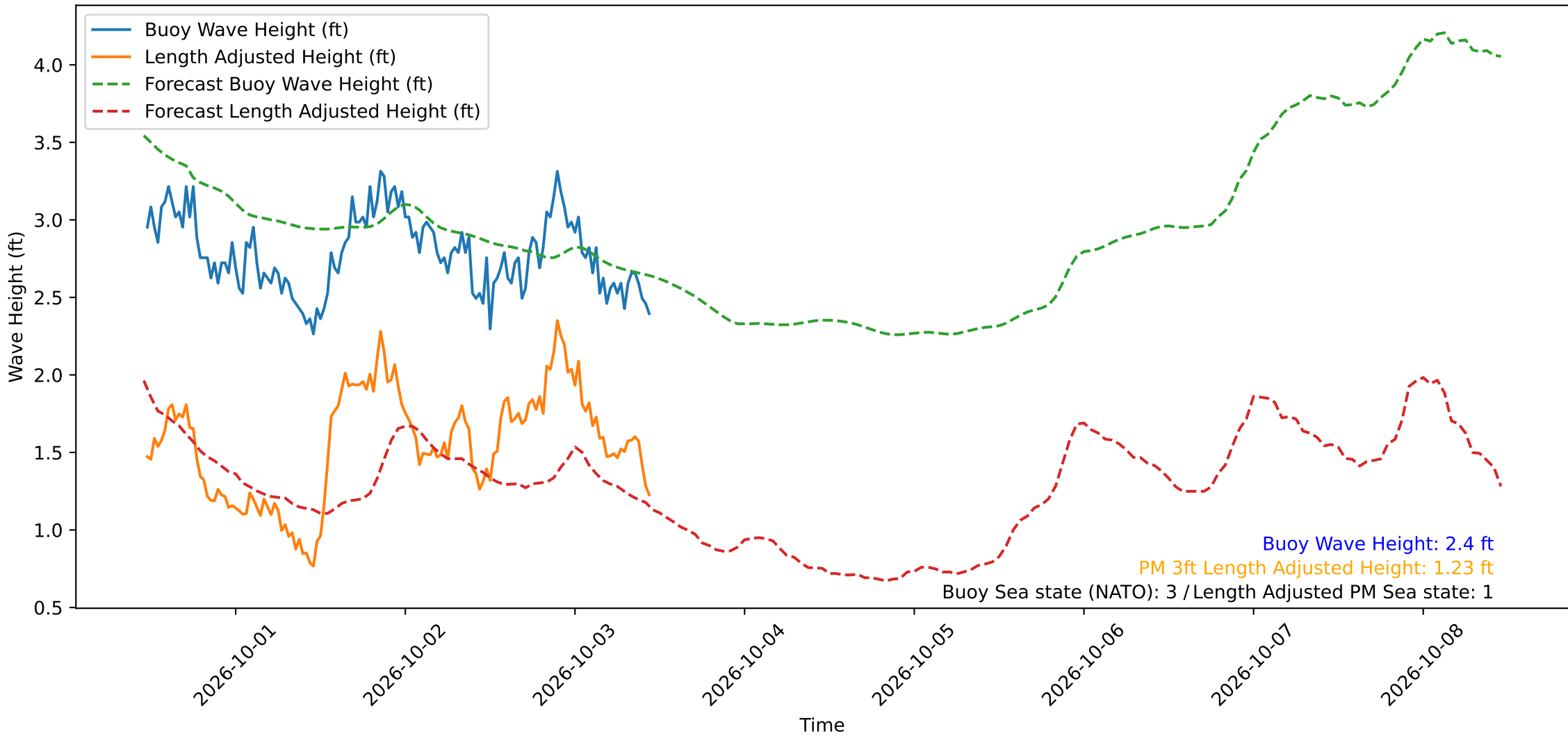
Wave Heights over Time for Oceanside Harbor at 2026-10-03 11:20:29
