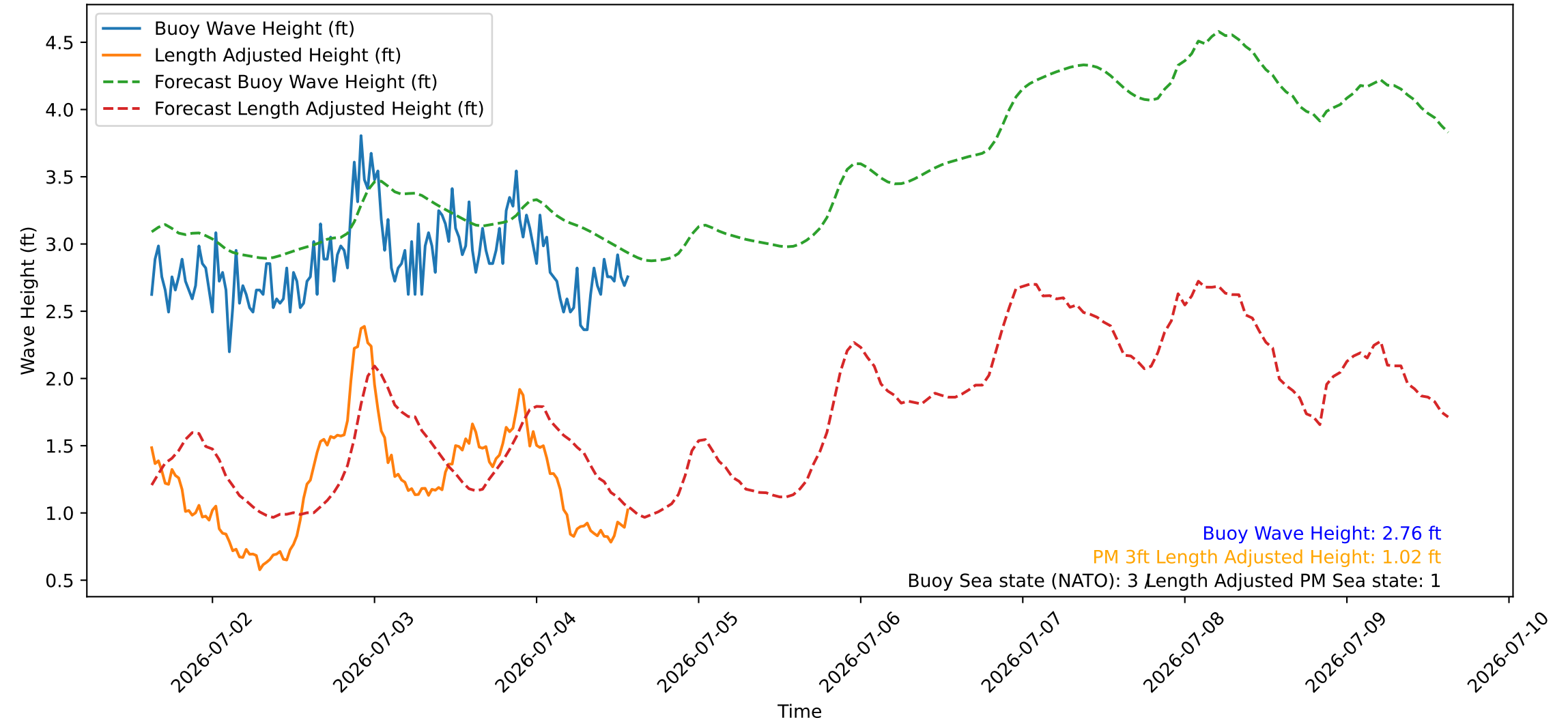
Wave Heights over Time for Red Beach at 2026-07-04 14:30:46
