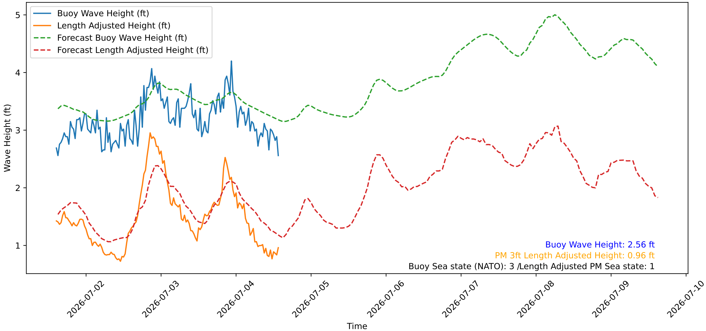
Wave Heights over Time for Green Beach at 2026-07-04 14:31:08
