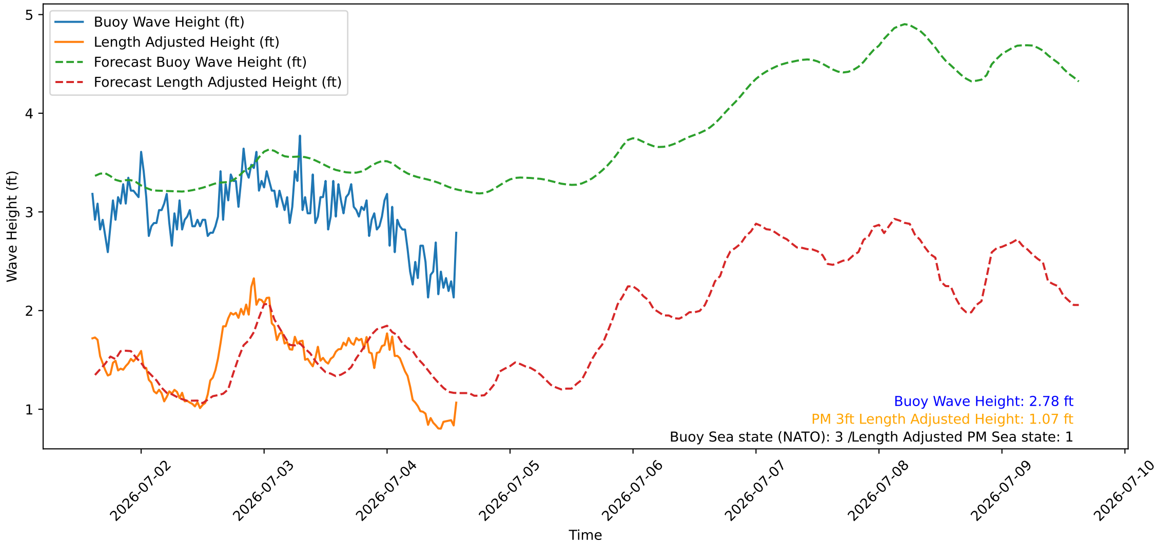
Wave Heights over Time for Oceanside Harbor at 2026-07-04 14:30:26
