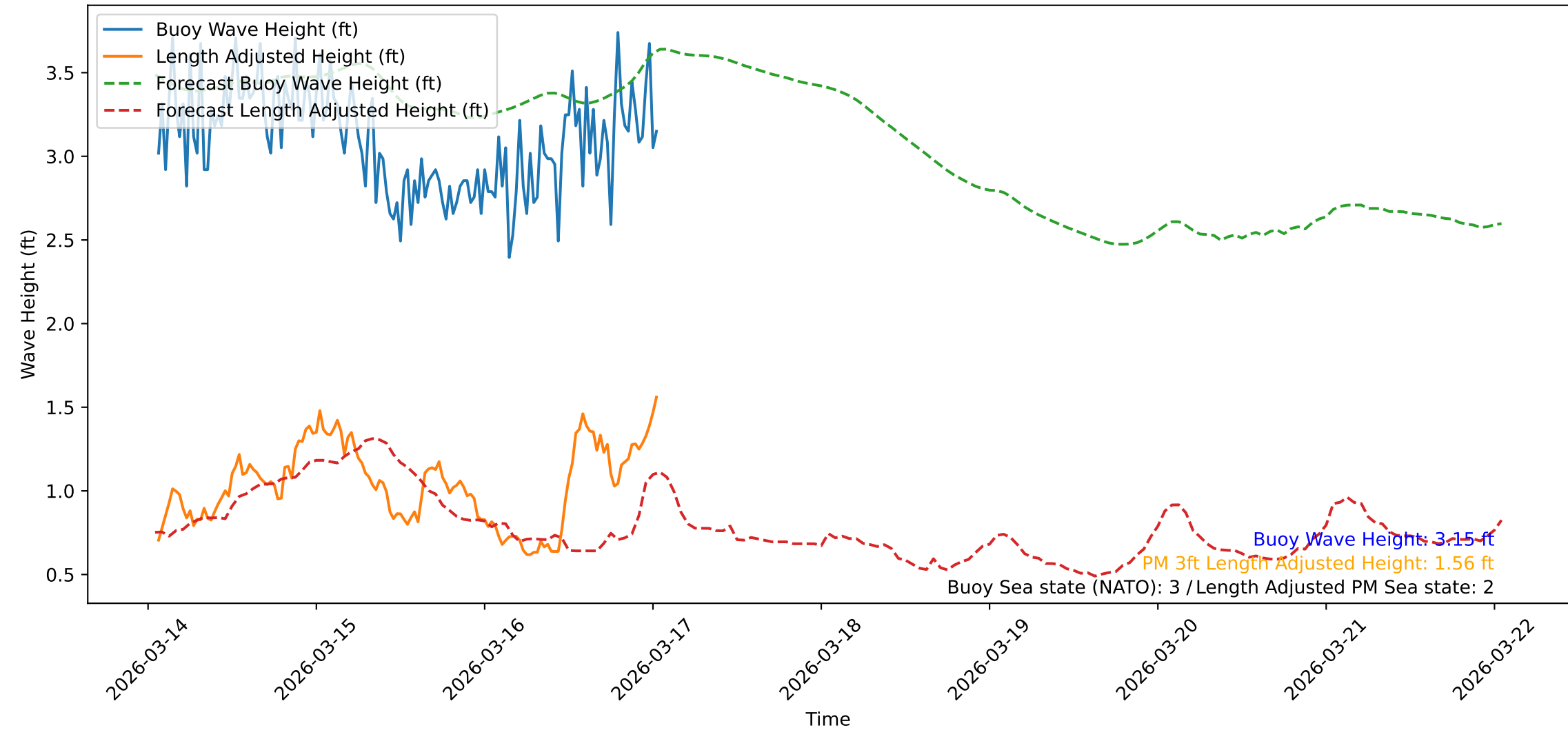
Wave Heights over Time for Oceanside Harbor at 2026-03-17 01:20:45
