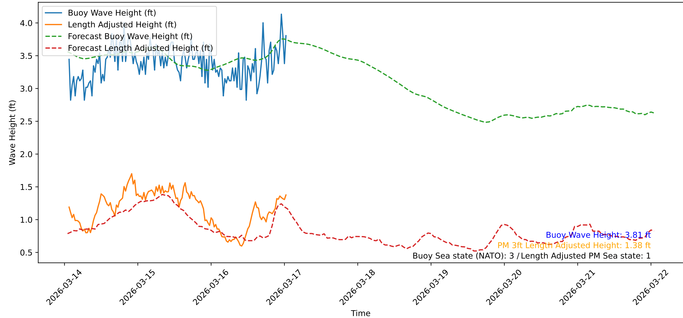
Wave Heights over Time for Green Beach at 2026-03-17 01:21:45
