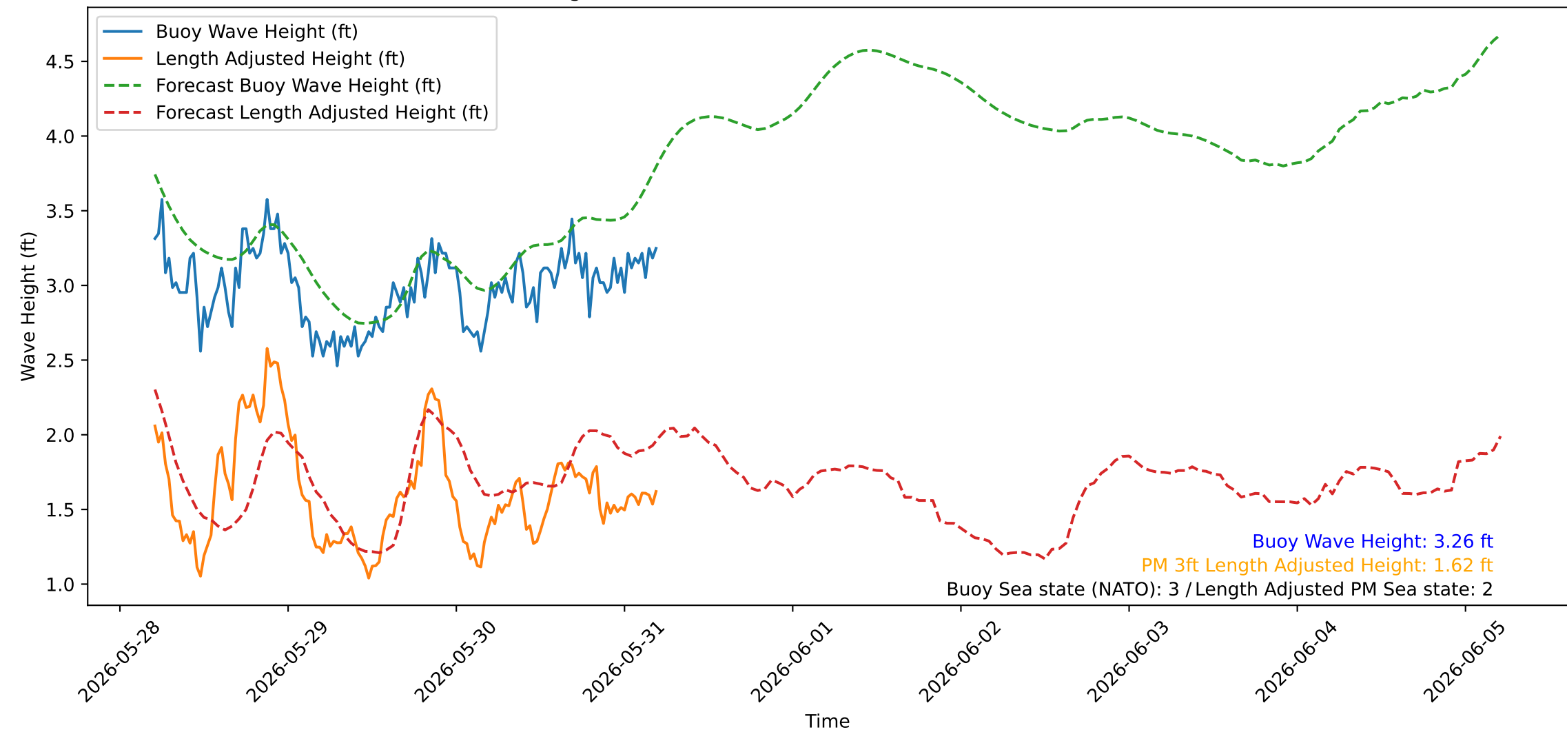
Wave Heights over Time for Green Beach at 2026-05-31 05:11:07
