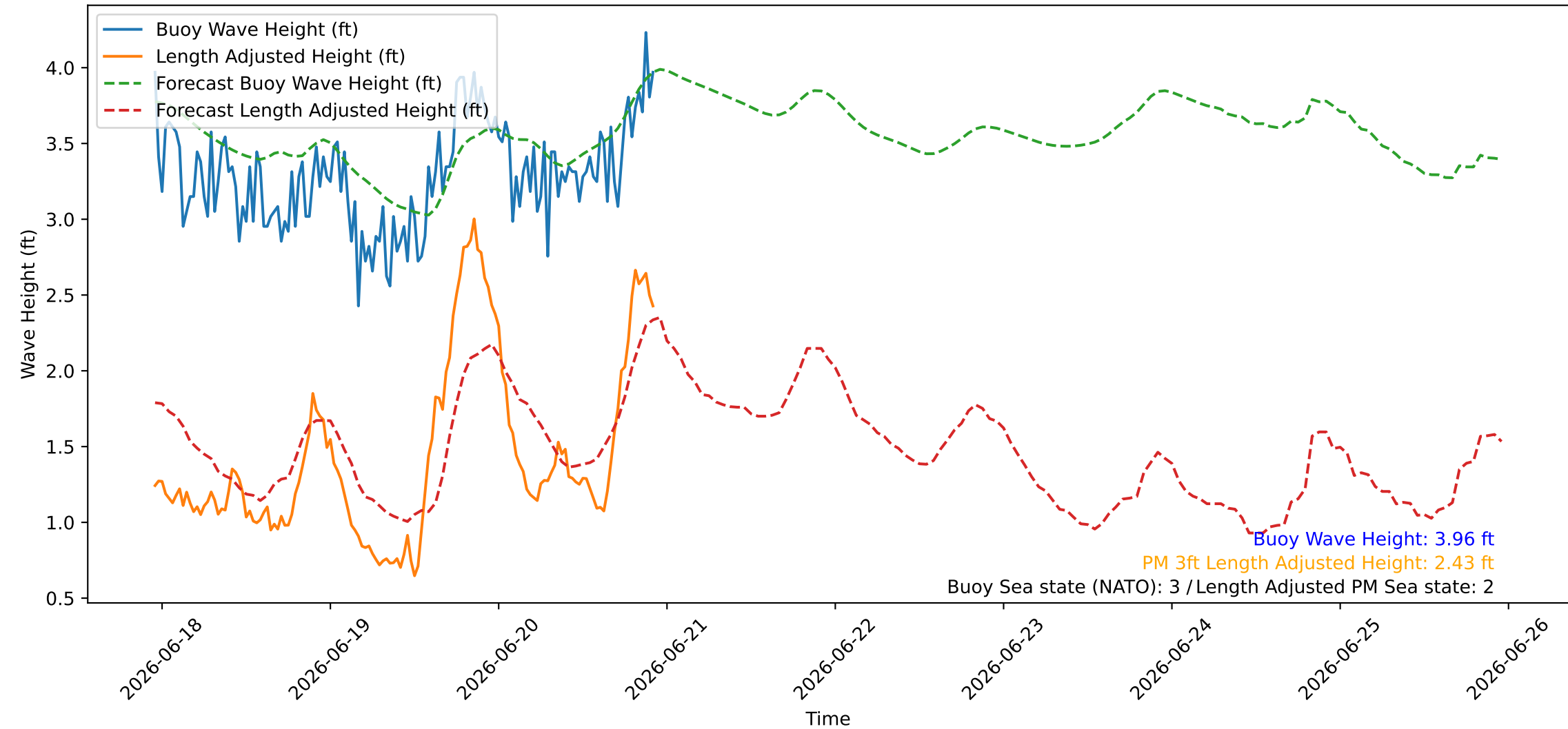
Wave Heights over Time for Green Beach at 2026-06-20 22:51:08
