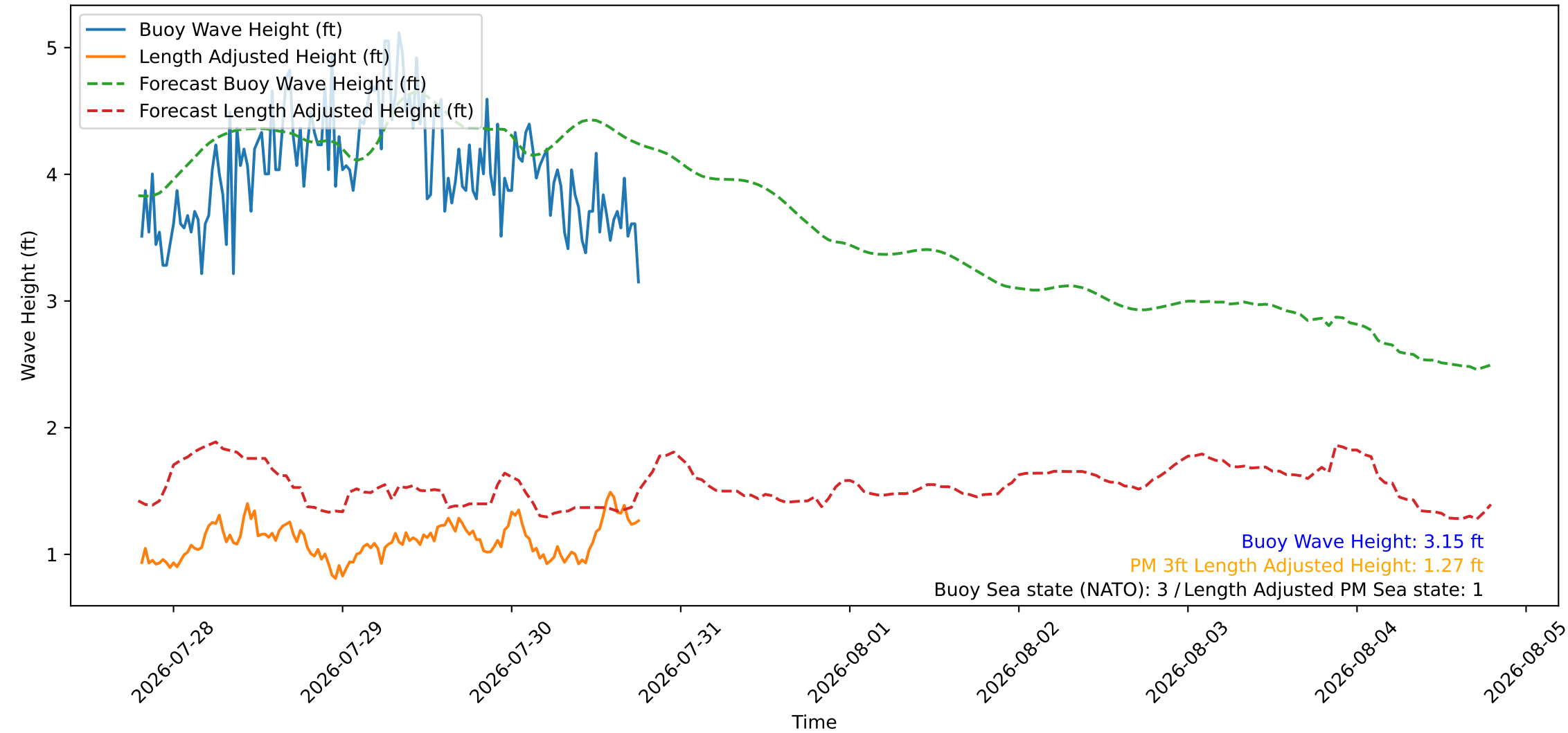
Wave Heights over Time for Red Beach at 2026-07-30 19:00:45
