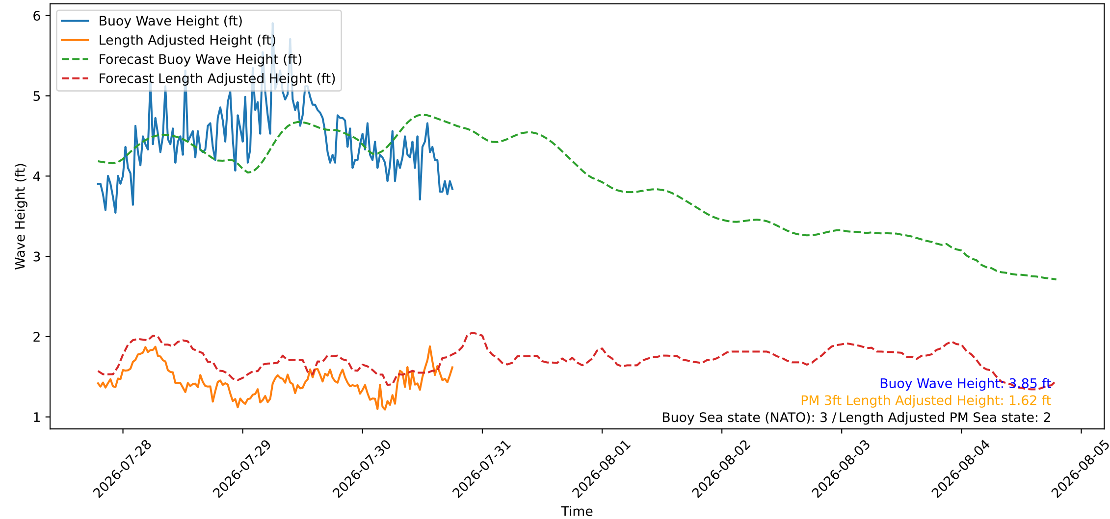
Wave Heights over Time for Oceanside Harbor at 2026-07-30 19:00:26
