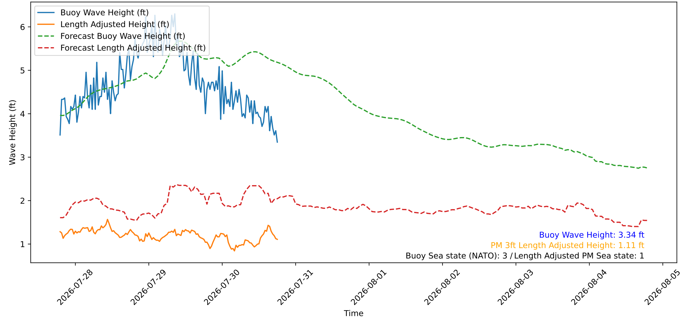
Wave Heights over Time for Green Beach at 2026-07-30 19:01:08
