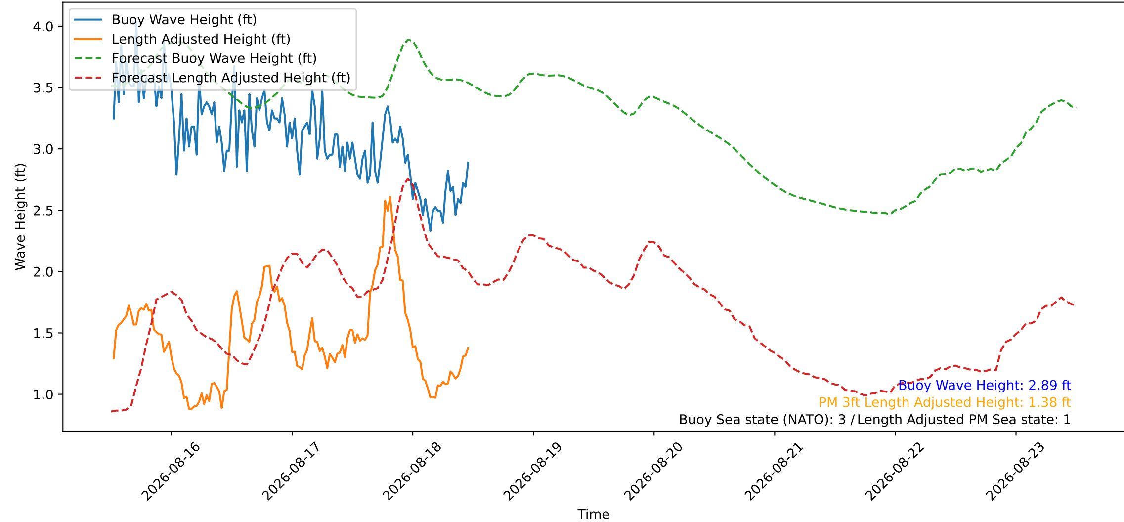
Wave Heights over Time for Red Beach at 2026-08-18 12:20:46
