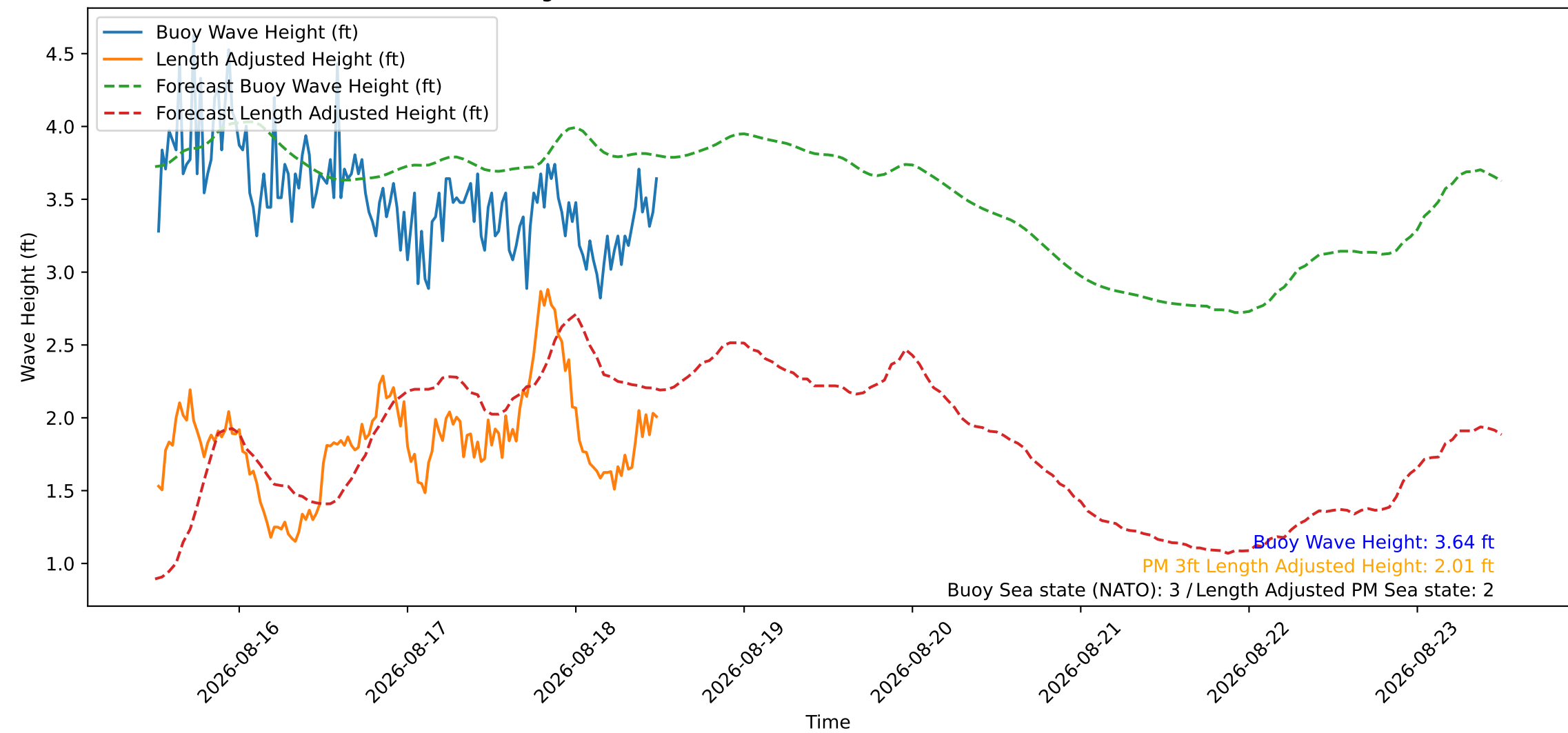
Wave Heights over Time for Oceanside Harbor at 2026-08-18 12:20:26
