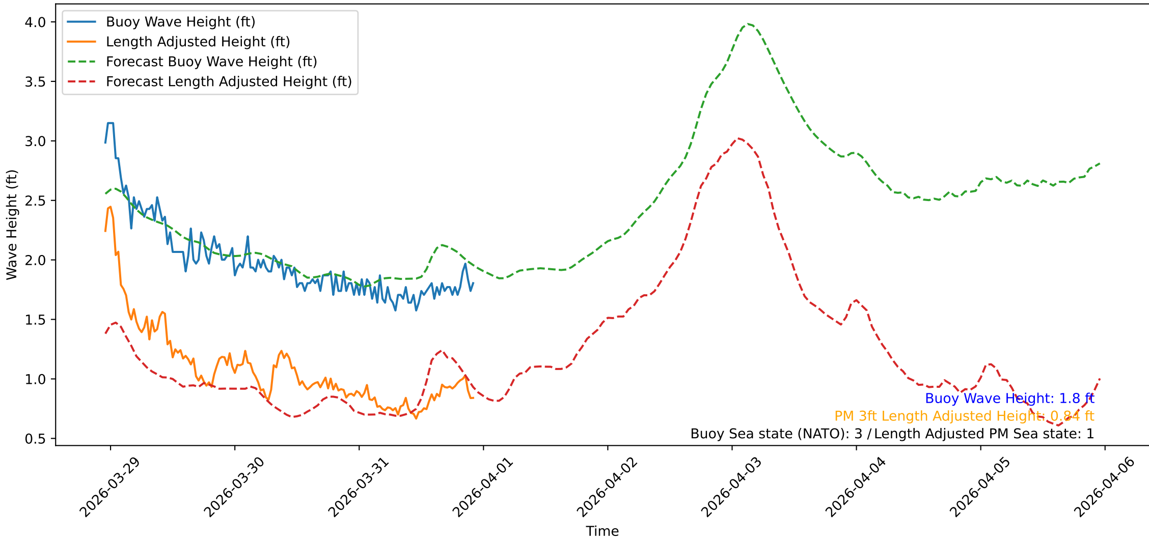
Wave Heights over Time for Oceanside Harbor at 2026-03-31 22:50:31
