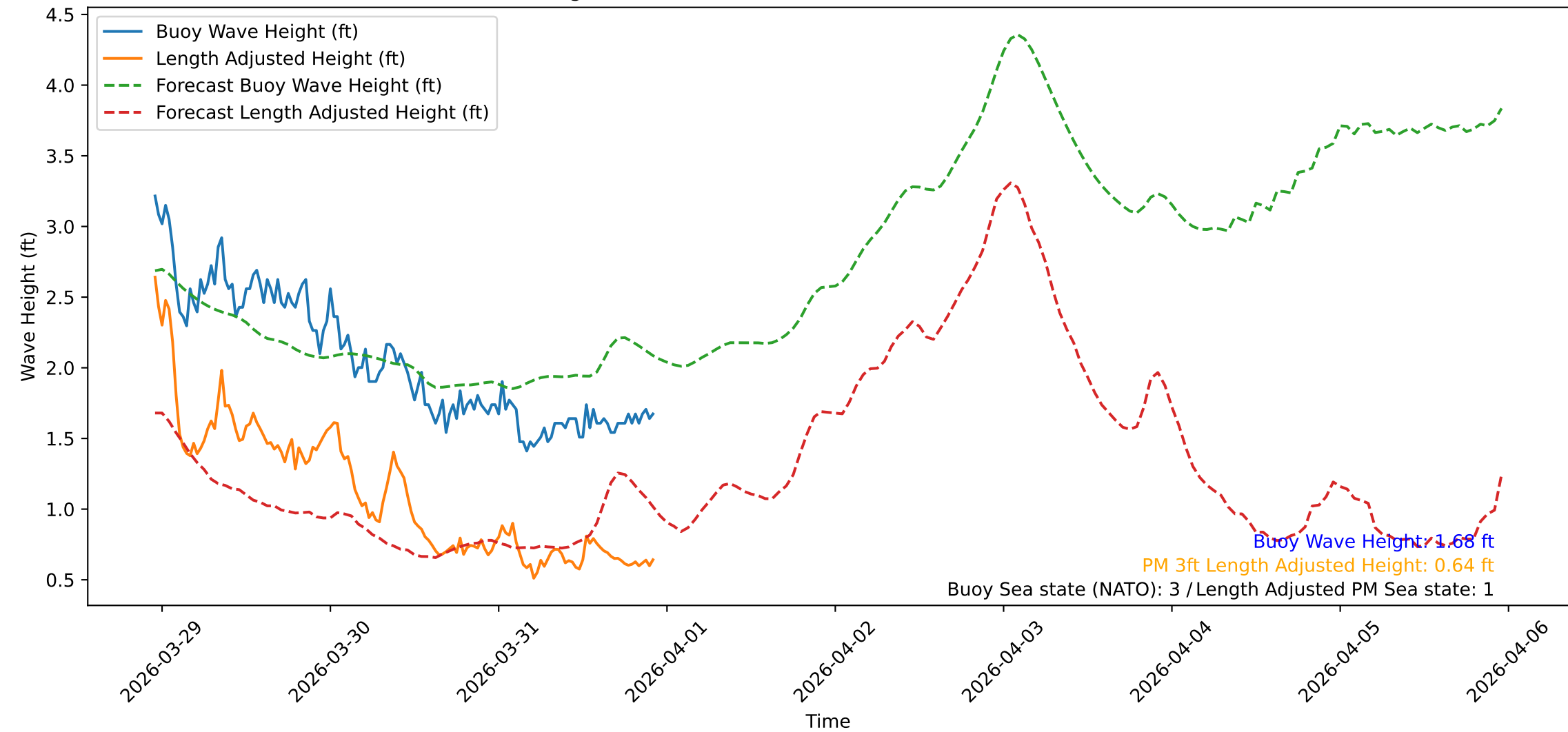
Wave Heights over Time for Green Beach at 2026-03-31 22:51:09
