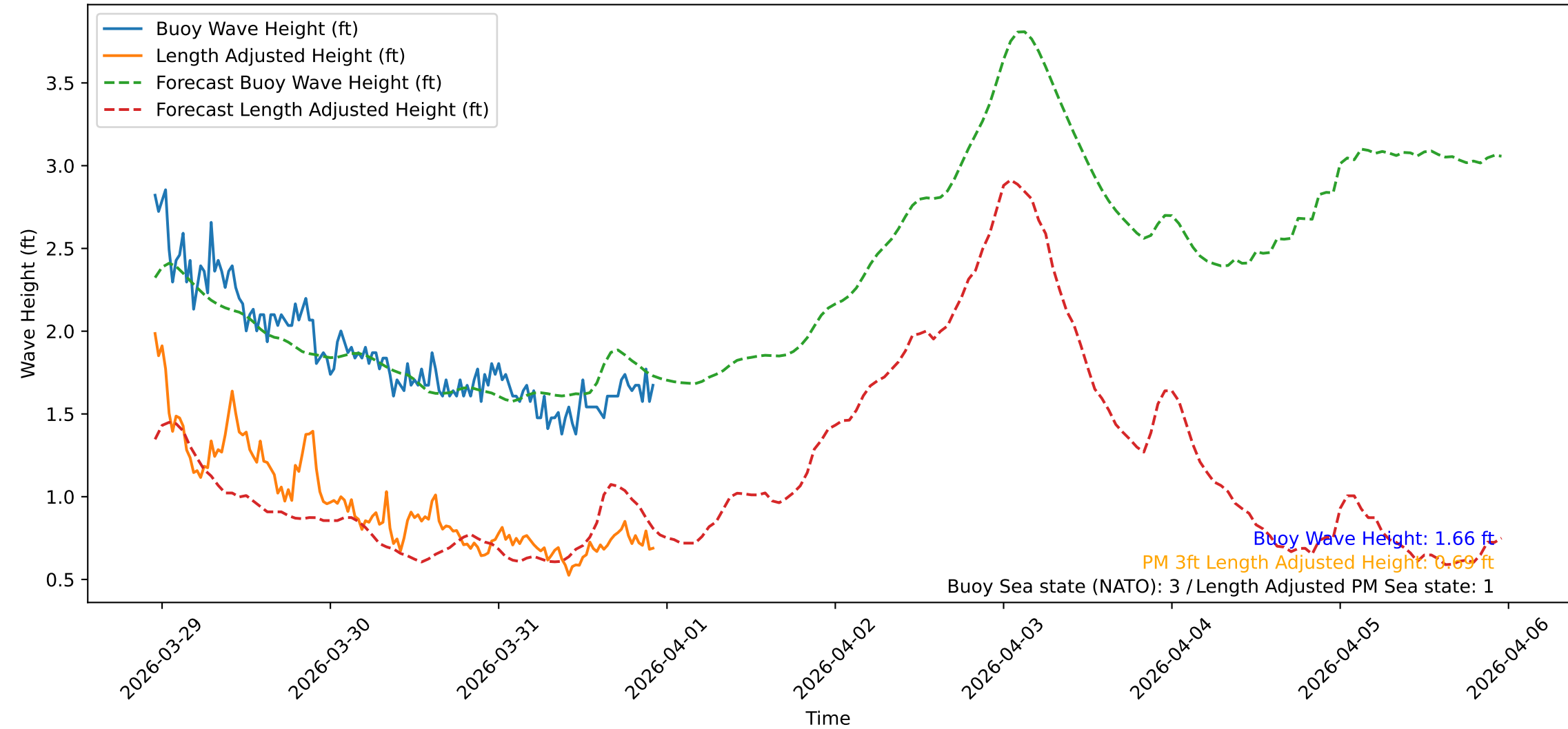
Wave Heights over Time for Red Beach at 2026-03-31 22:50:47
