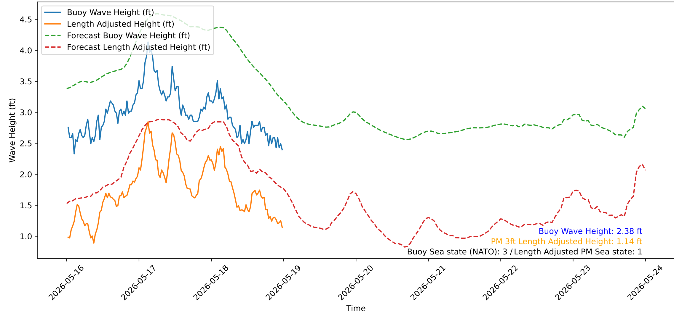
Wave Heights over Time for Red Beach at 2026-05-19 00:10:51
