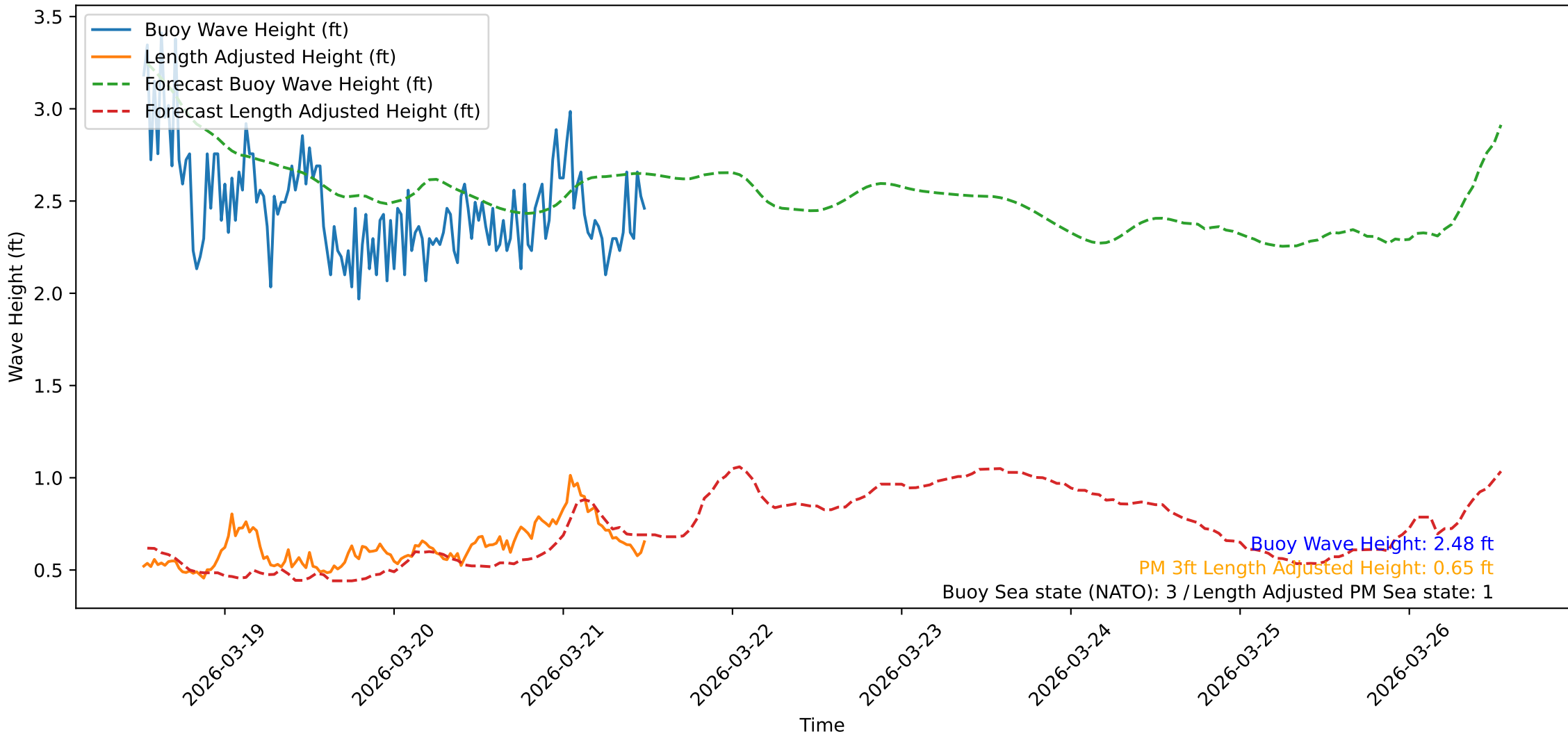
Wave Heights over Time for Oceanside Harbor at 2026-03-21 12:40:31
