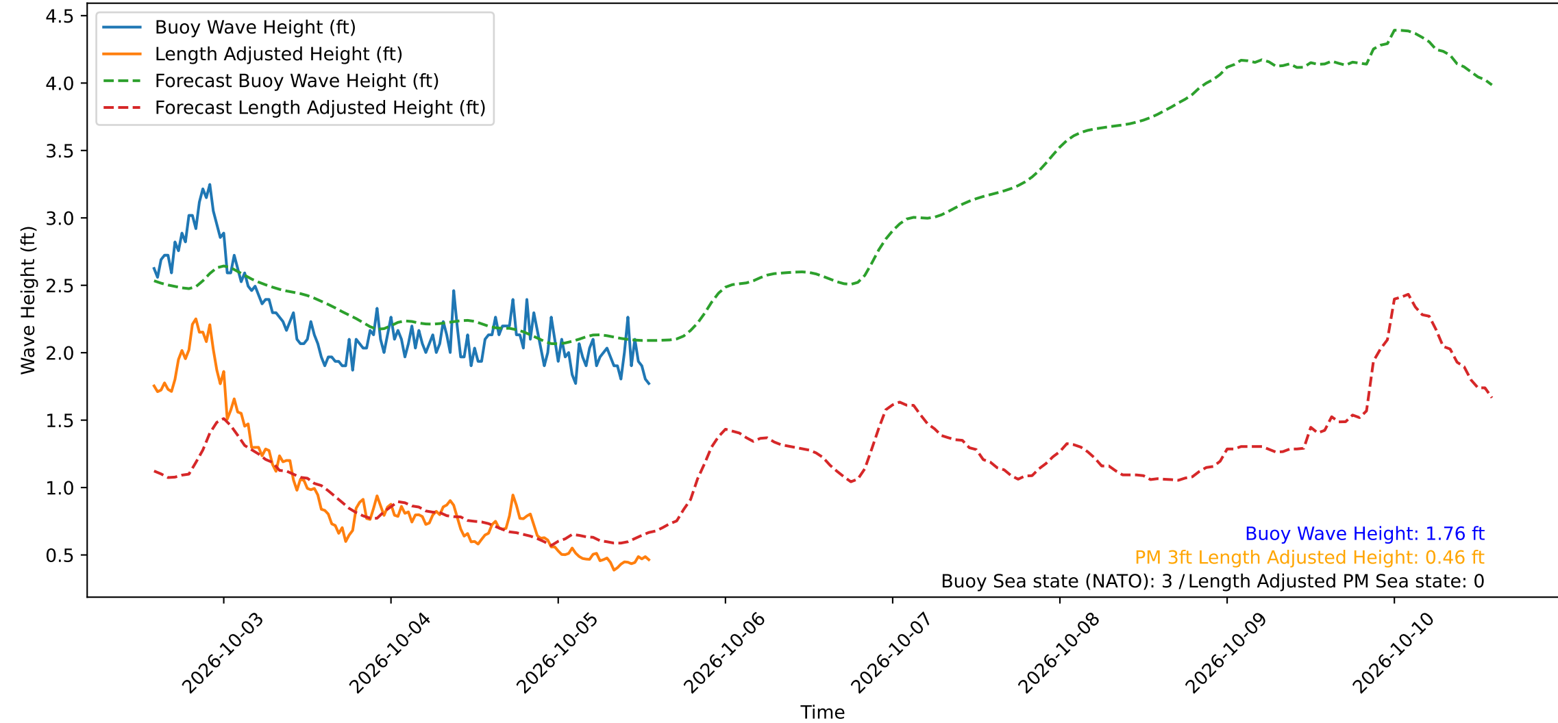
Wave Heights over Time for Red Beach at 2026-10-05 13:40:50
