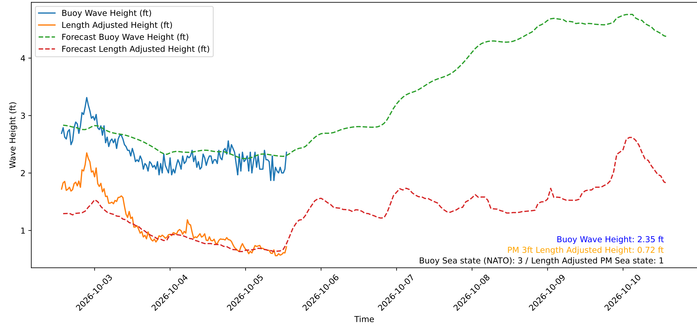
Wave Heights over Time for Oceanside Harbor at 2026-10-05 13:40:31
