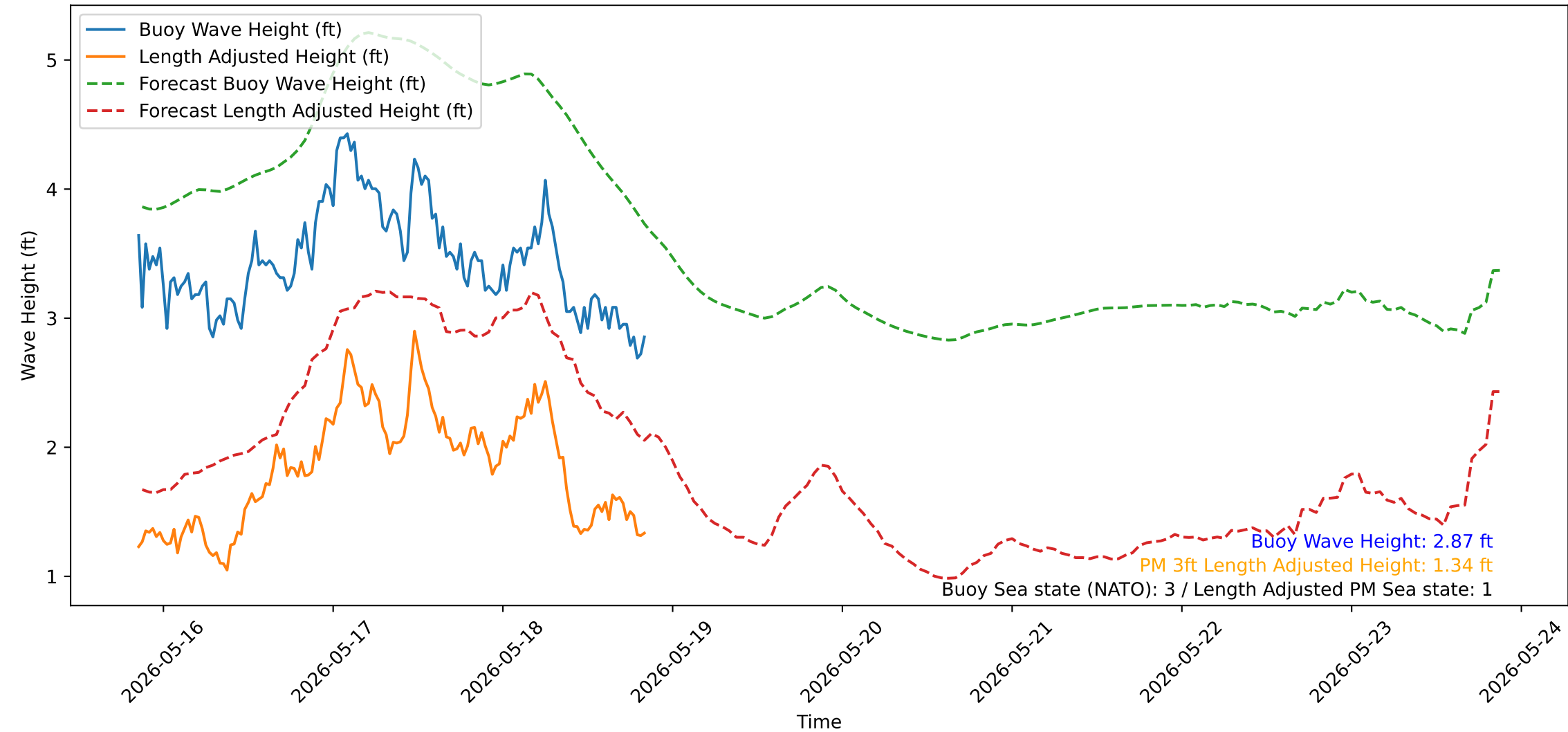
Wave Heights over Time for Green Beach at 2026-05-18 20:41:15
