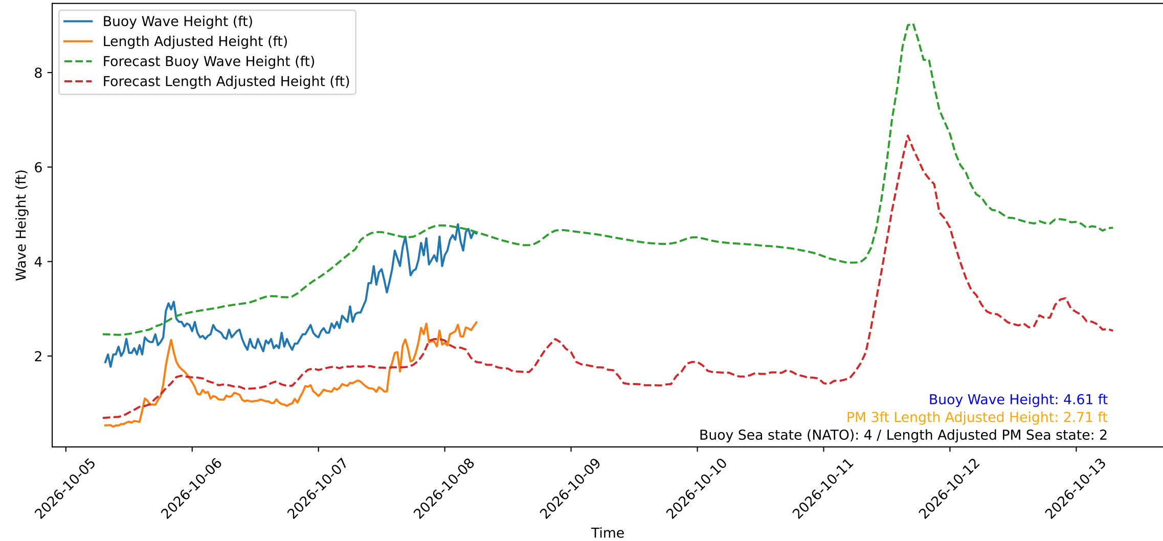
Wave Heights over Time for Green Beach at 2026-10-08 07:01:11
