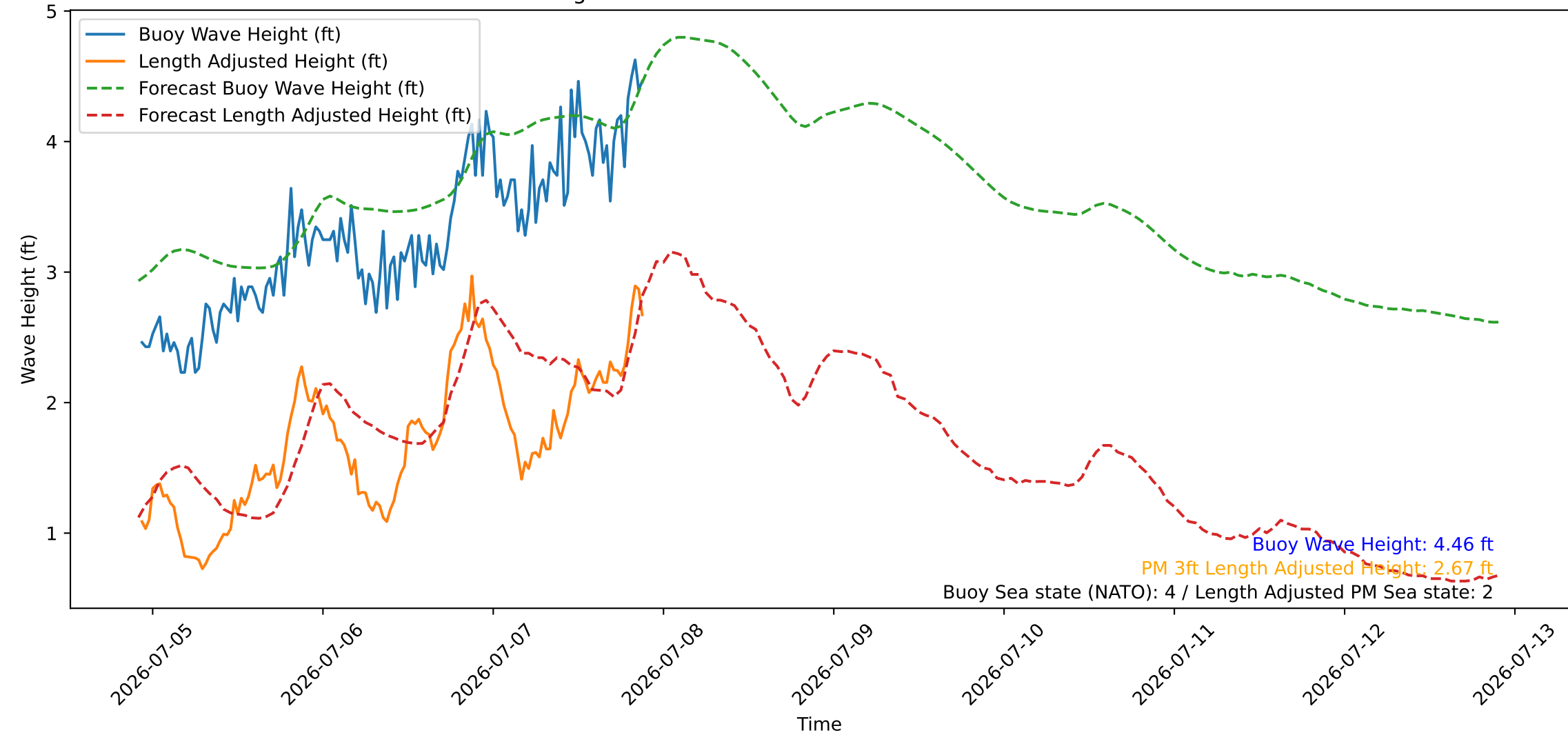
Wave Heights over Time for Red Beach at 2026-07-07 22:00:45
