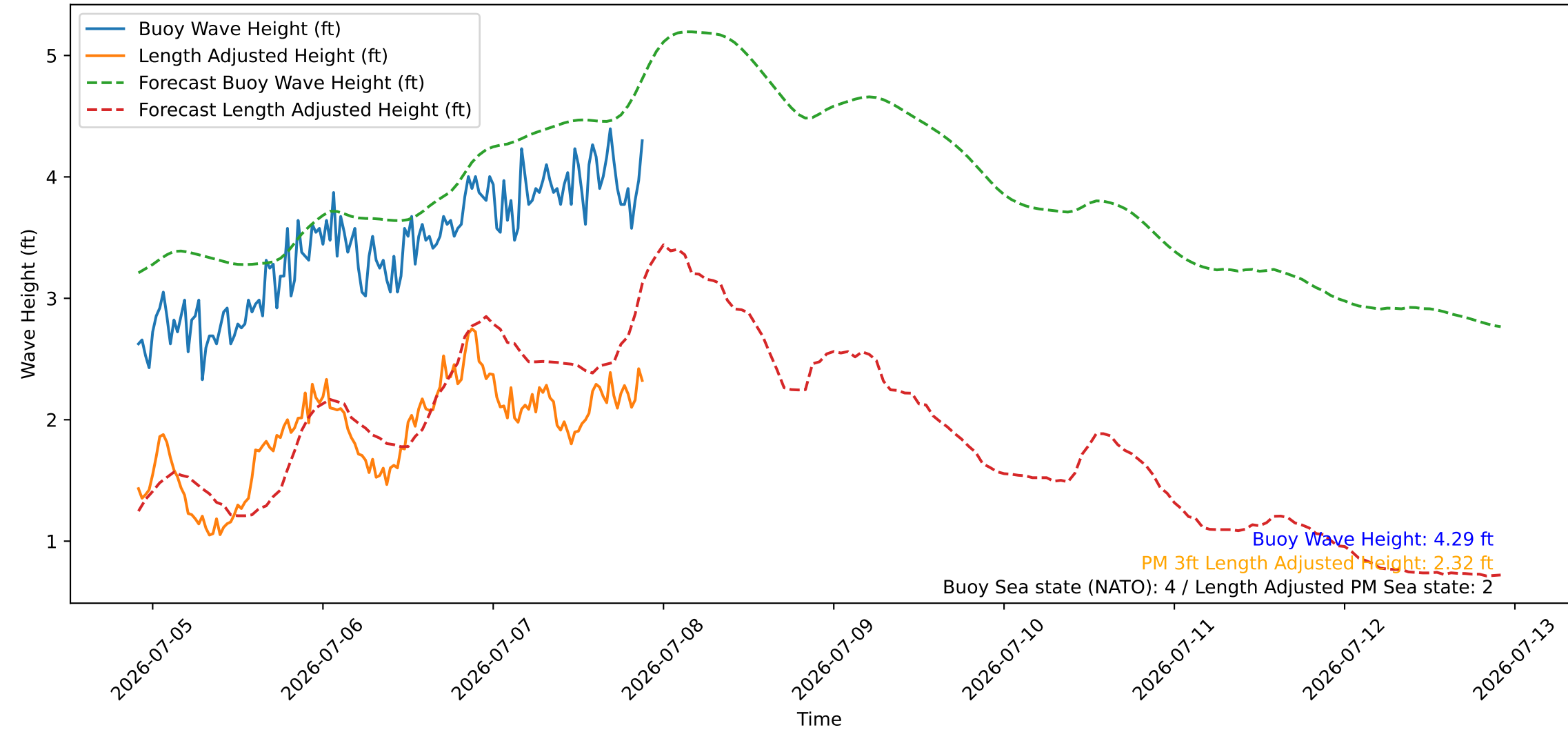
Wave Heights over Time for Oceanside Harbor at 2026-07-07 22:00:26
