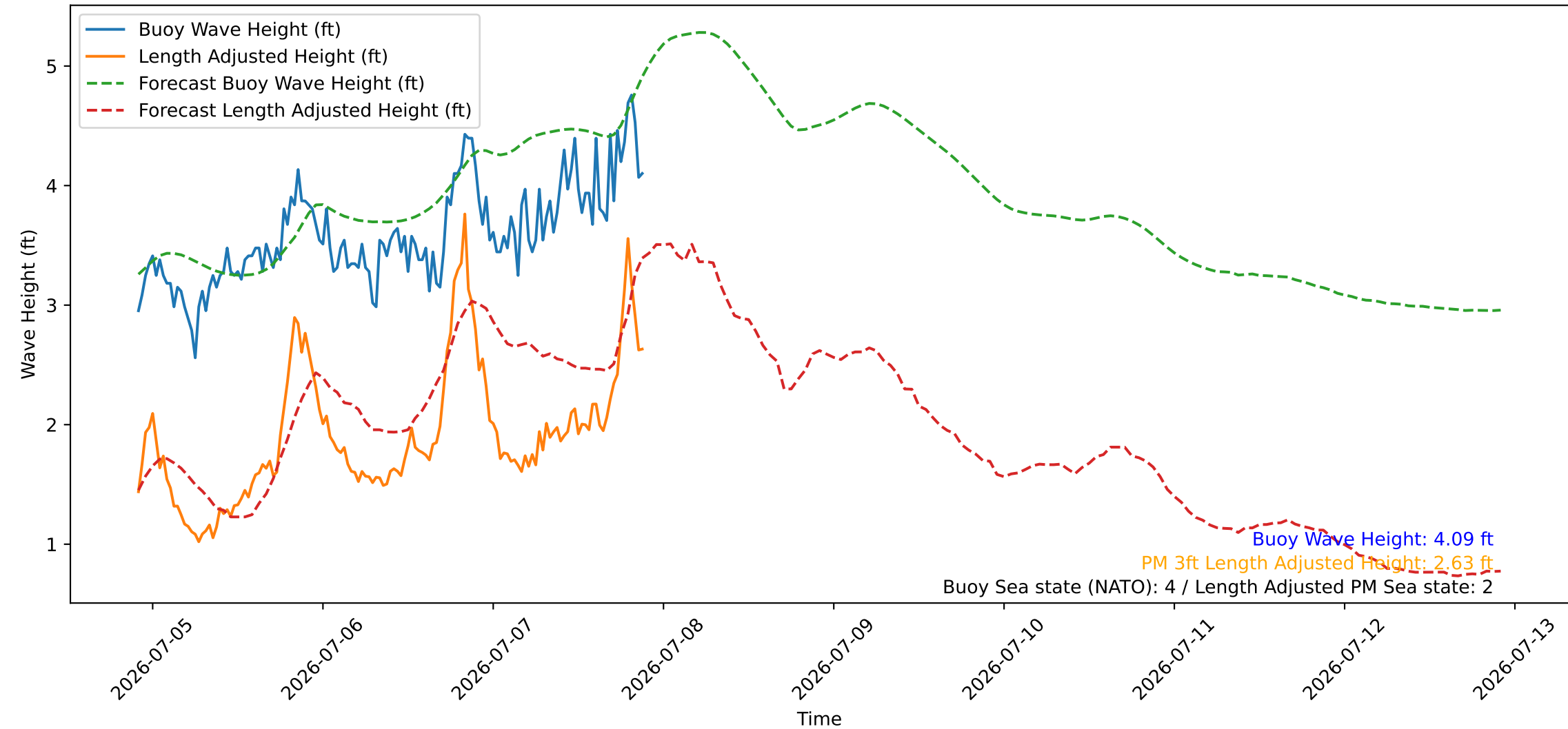
Wave Heights over Time for Green Beach at 2026-07-07 22:01:08
