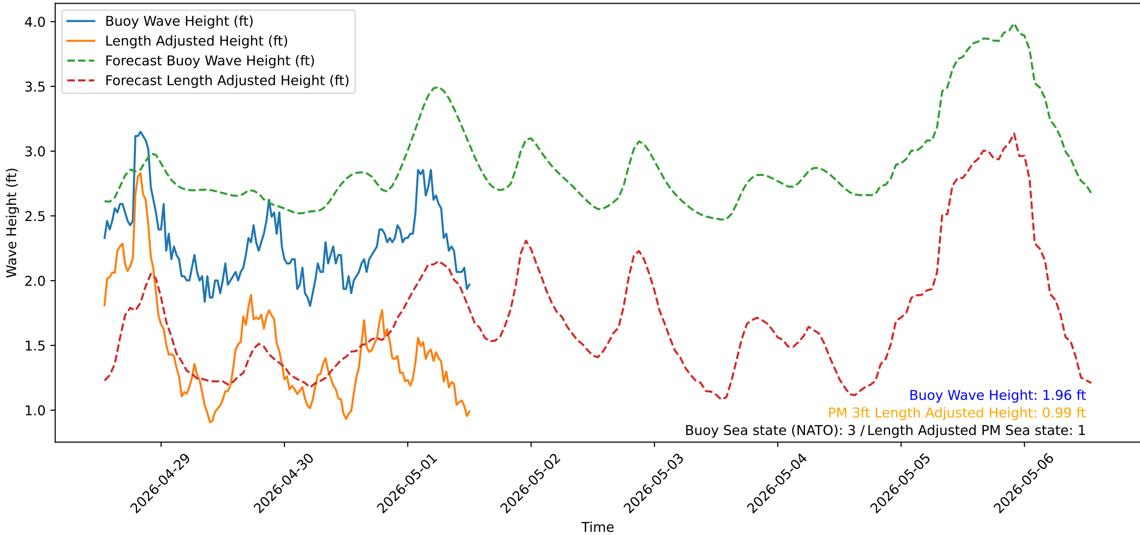
Wave Heights over Time for Green Beach at 2026-05-01 13:01:13
