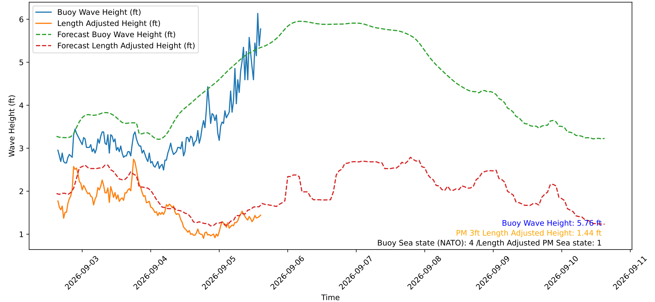
Wave Heights over Time for Green Beach at 2026-09-05 15:11:12
