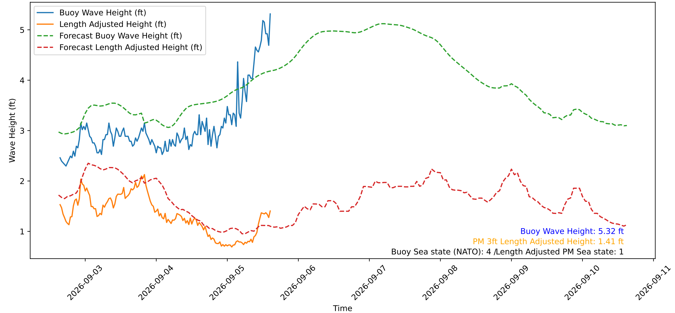
Wave Heights over Time for Red Beach at 2026-09-05 15:10:49
