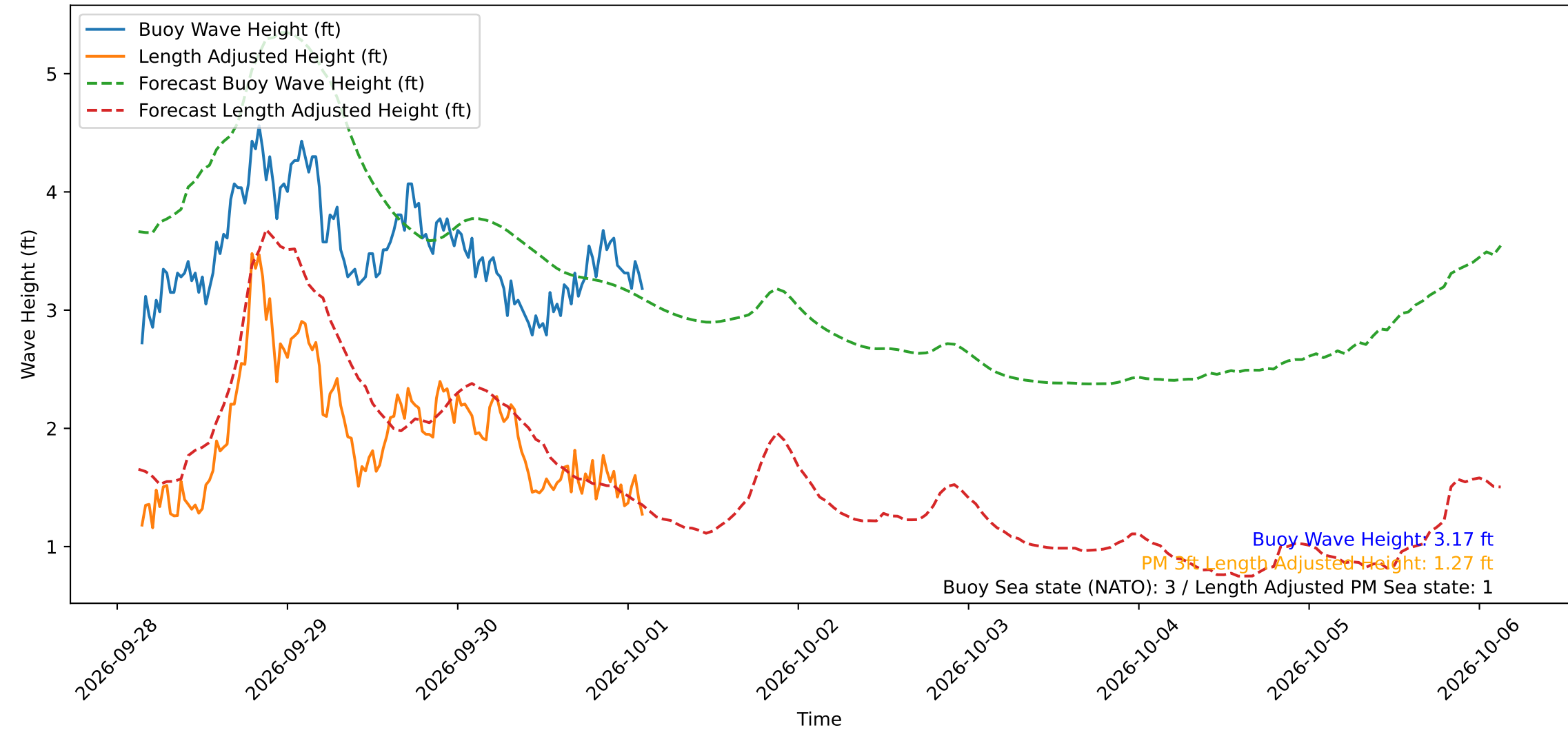
Wave Heights over Time for Green Beach at 2026-10-01 03:01:13
