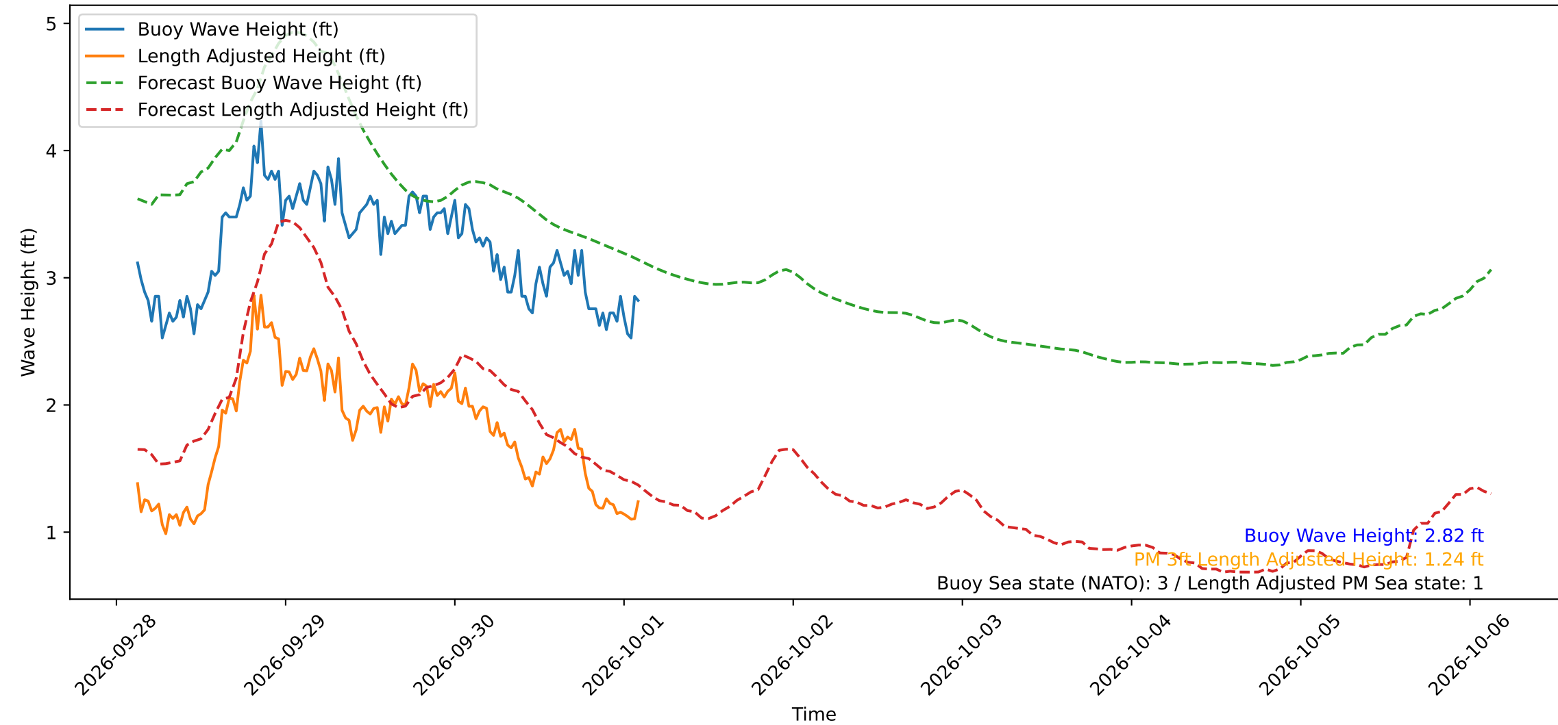
Wave Heights over Time for Oceanside Harbor at 2026-10-01 03:00:30
