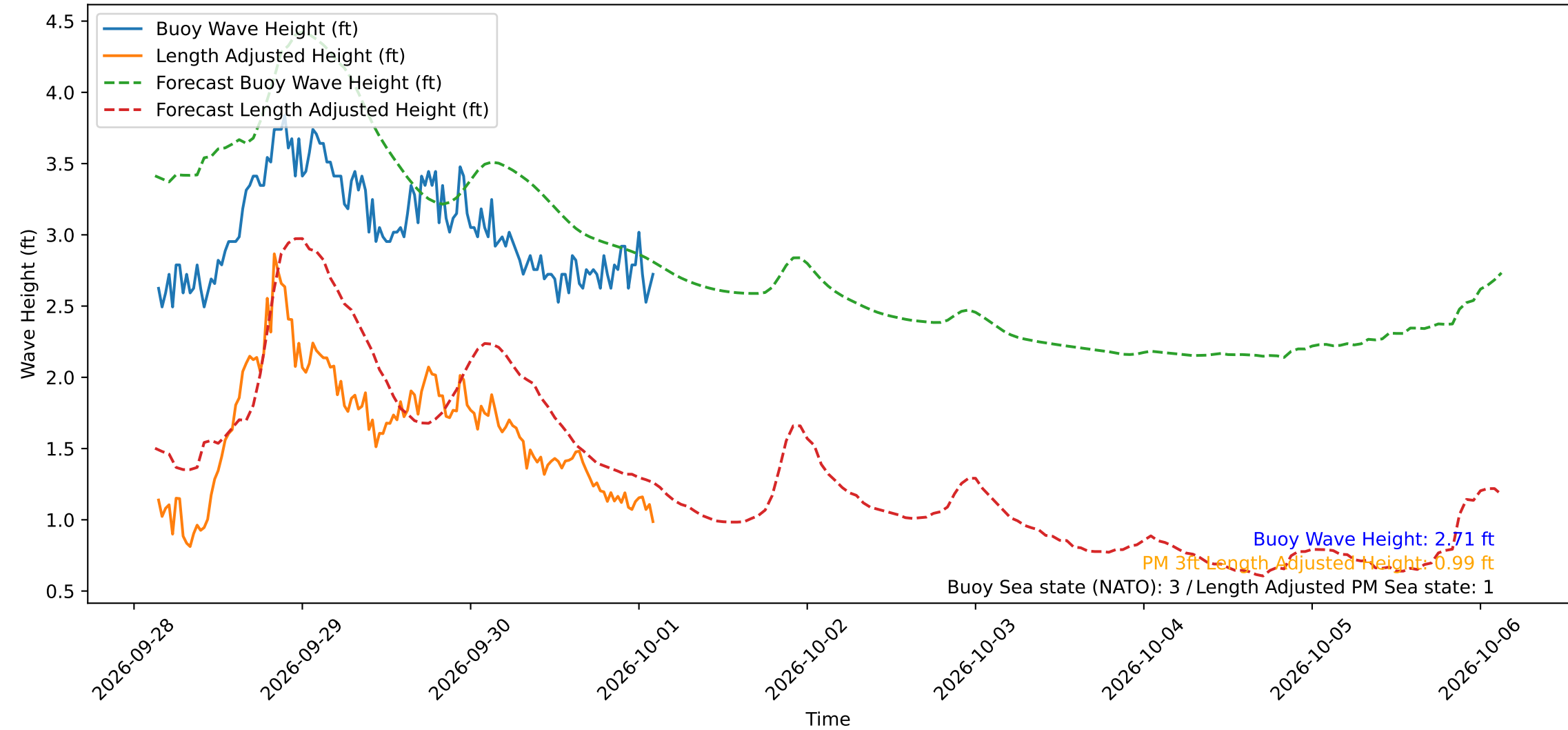
Wave Heights over Time for Red Beach at 2026-10-01 03:00:50
