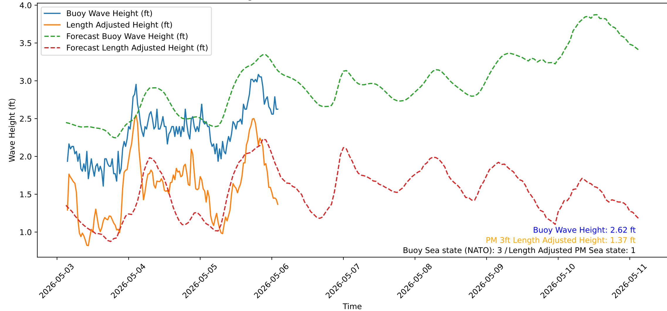
Wave Heights over Time for Red Beach at 2026-05-06 03:00:51
