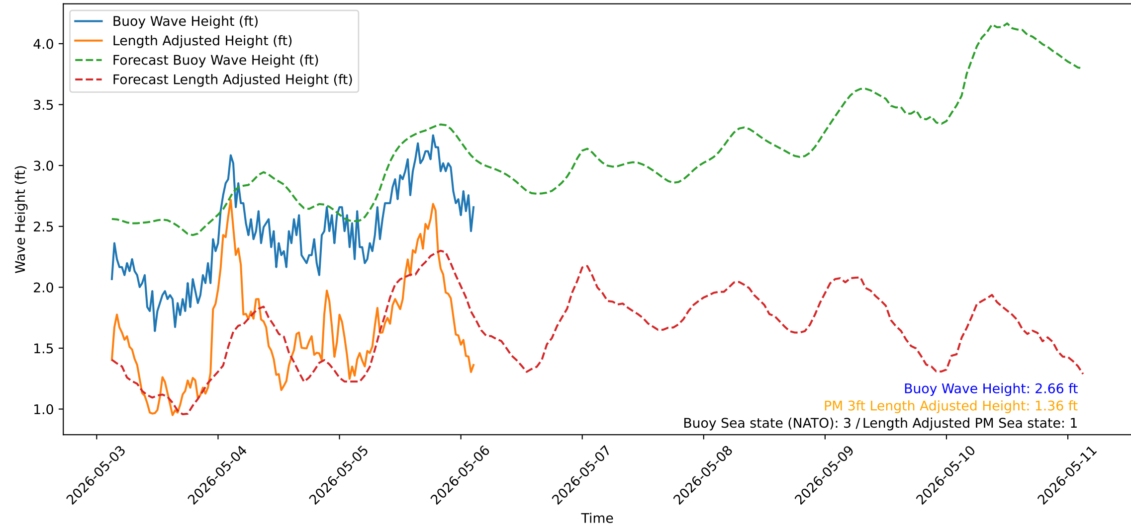
Wave Heights over Time for Oceanside Harbor at 2026-05-06 03:00:32
