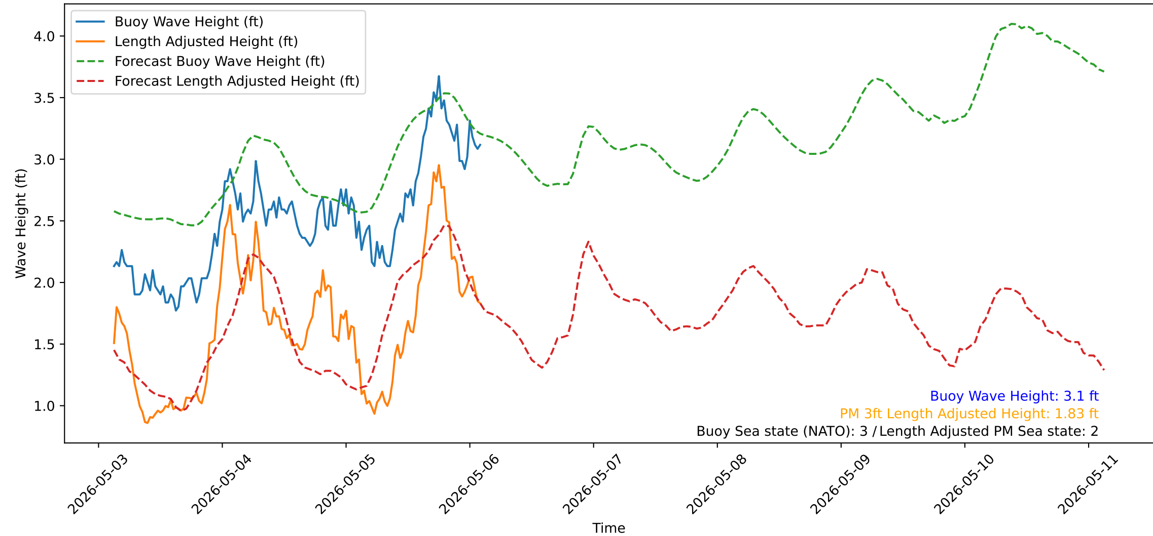
Wave Heights over Time for Green Beach at 2026-05-06 03:01:14
