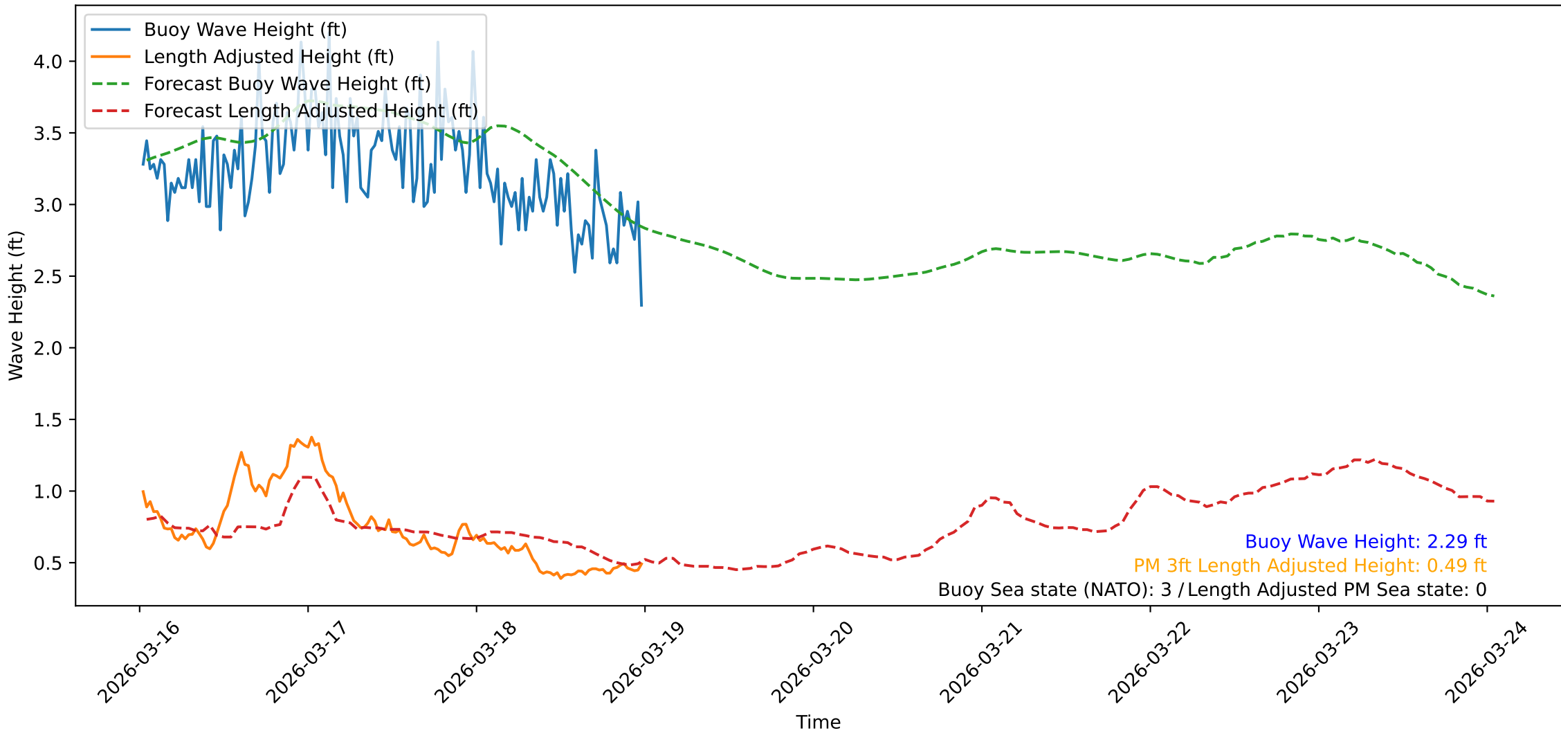
Wave Heights over Time for Green Beach at 2026-03-19 00:31:10
