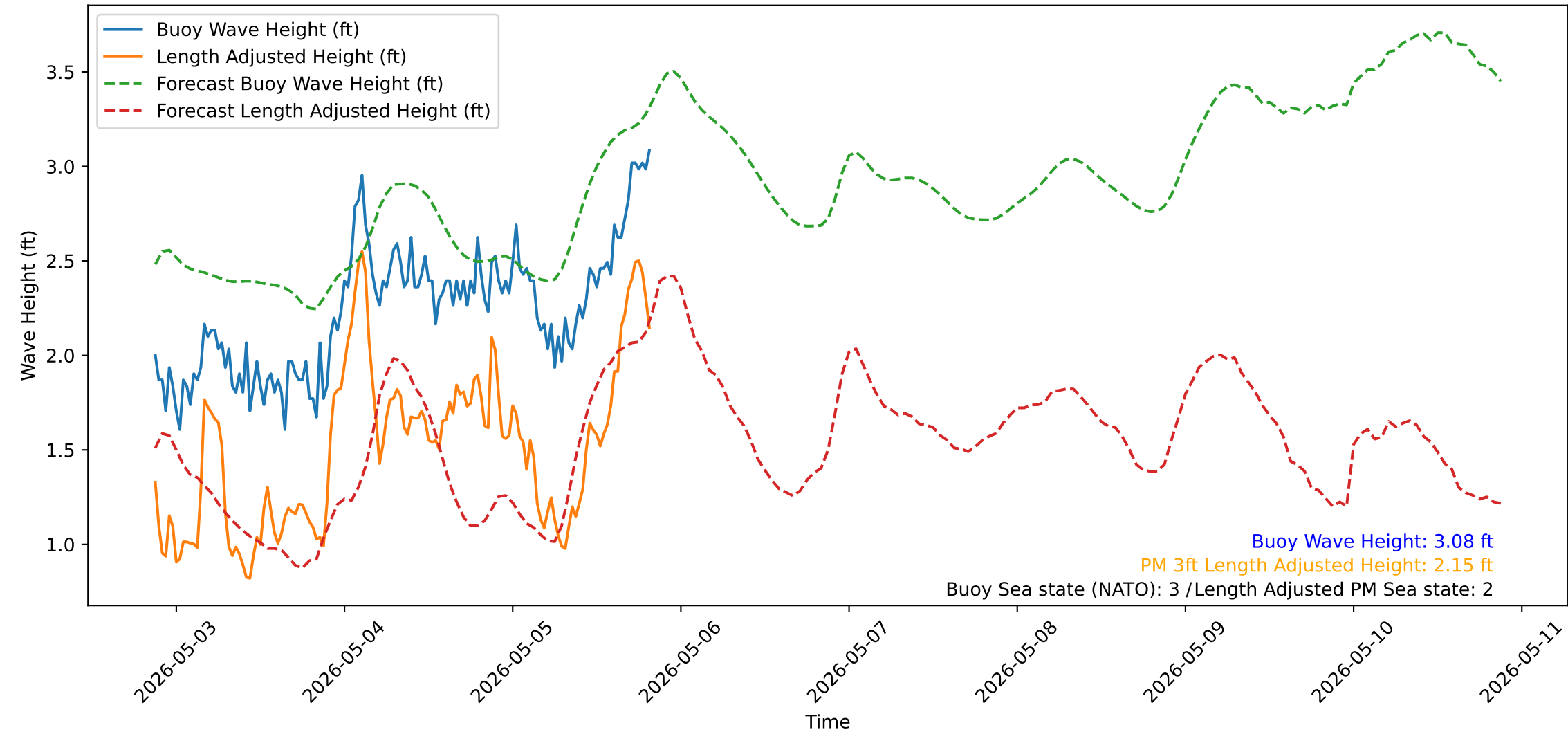
Wave Heights over Time for Red Beach at 2026-05-05 20:30:51
