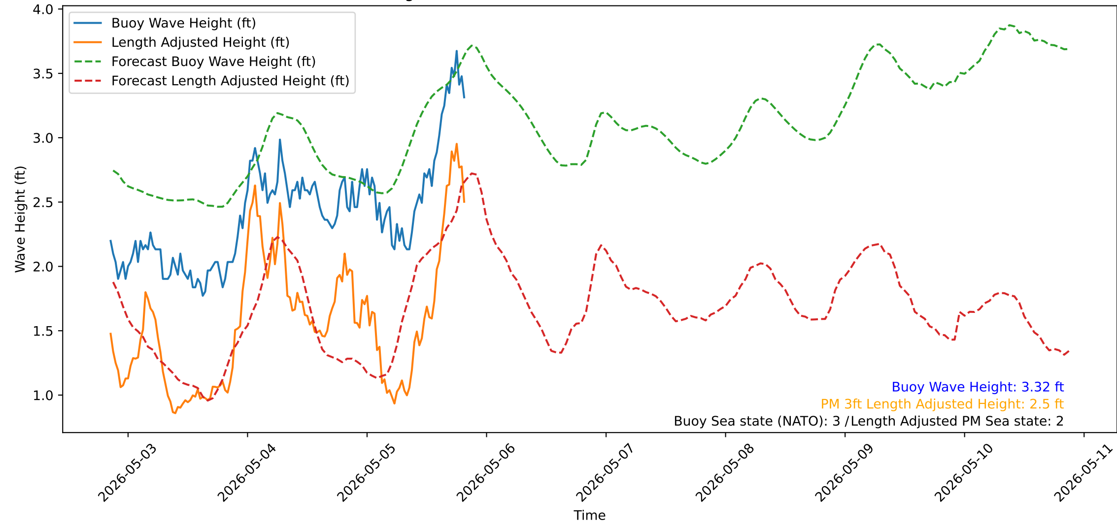
Wave Heights over Time for Green Beach at 2026-05-05 20:31:13
