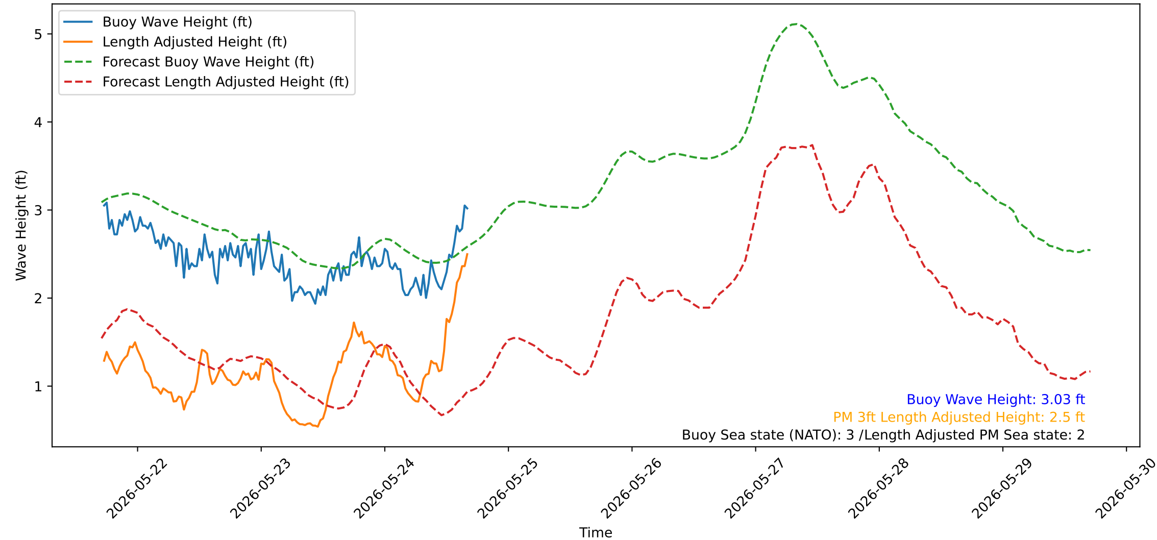
Wave Heights over Time for Red Beach at 2026-05-24 17:00:51
