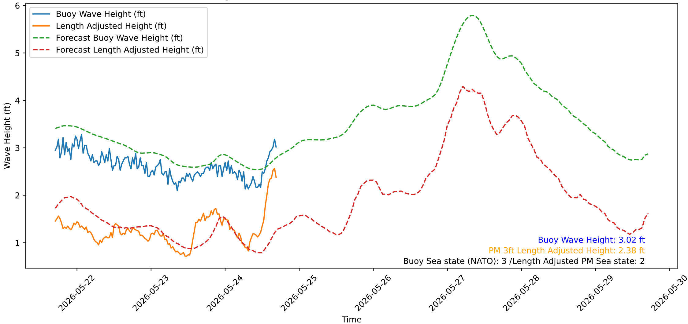
Wave Heights over Time for Oceanside Harbor at 2026-05-24 17:00:31
