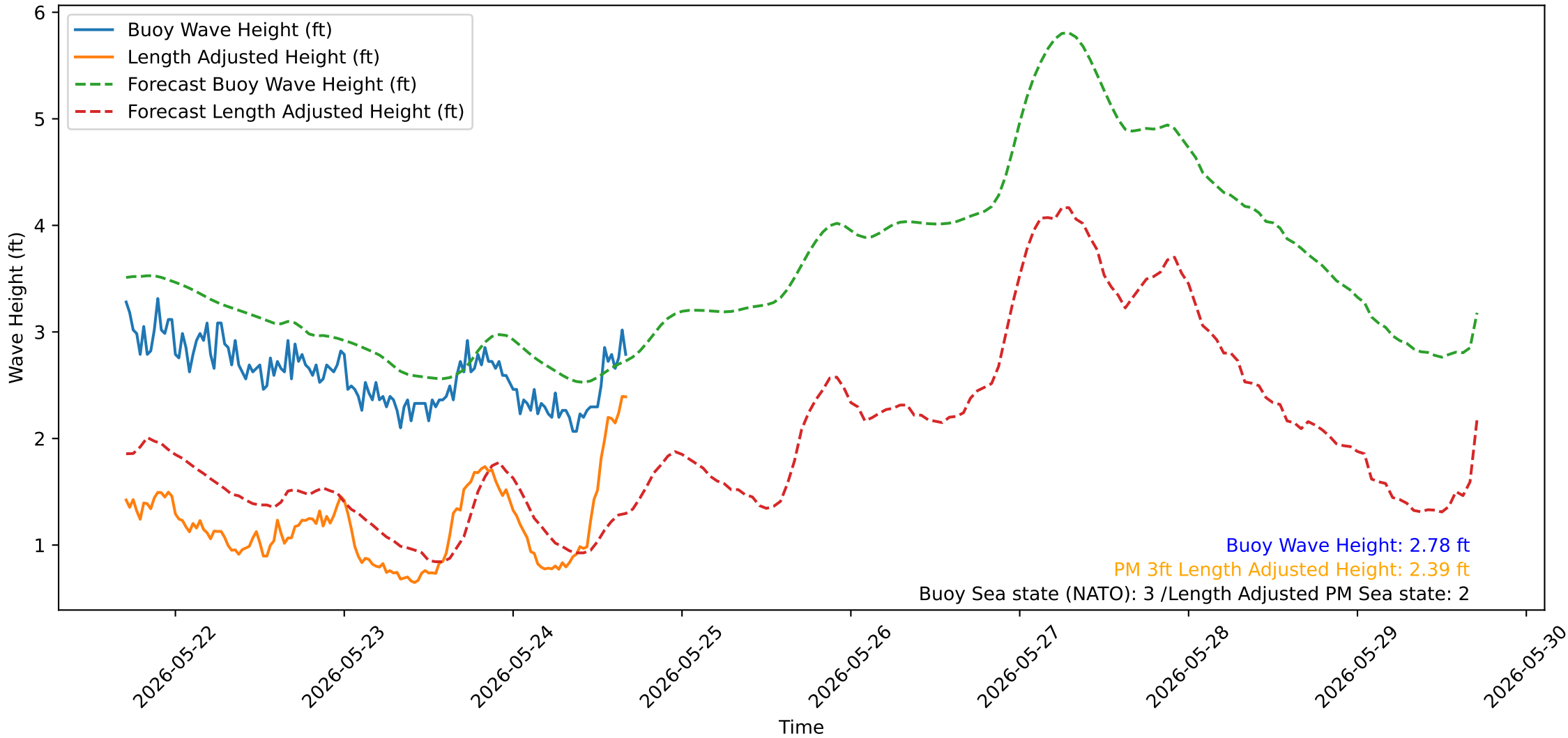
Wave Heights over Time for Green Beach at 2026-05-24 17:01:14
