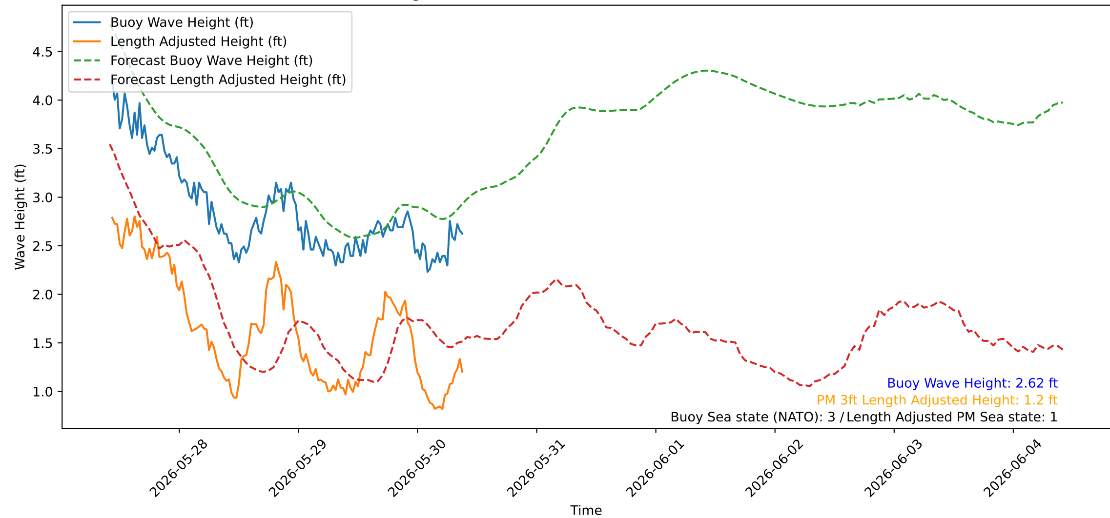
Wave Heights over Time for Red Beach at 2026-05-30 10:20:44
