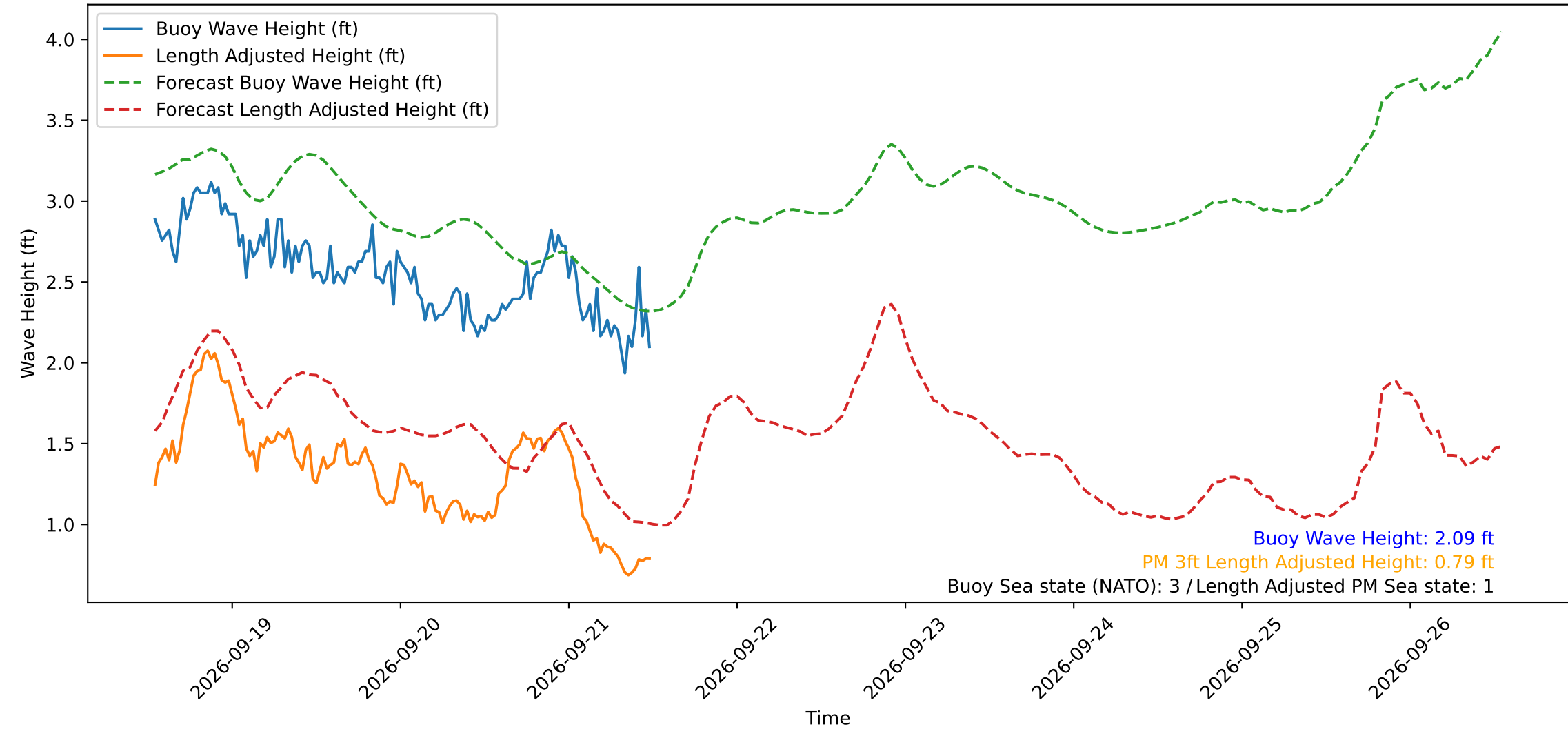
Wave Heights over Time for Green Beach at 2026-09-21 12:31:13
