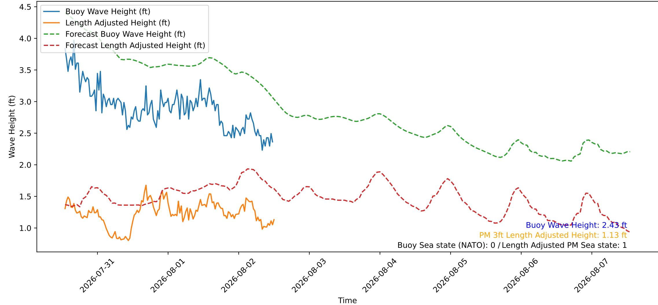
Wave Heights over Time for Red Beach at 2026-08-02 12:50:46
