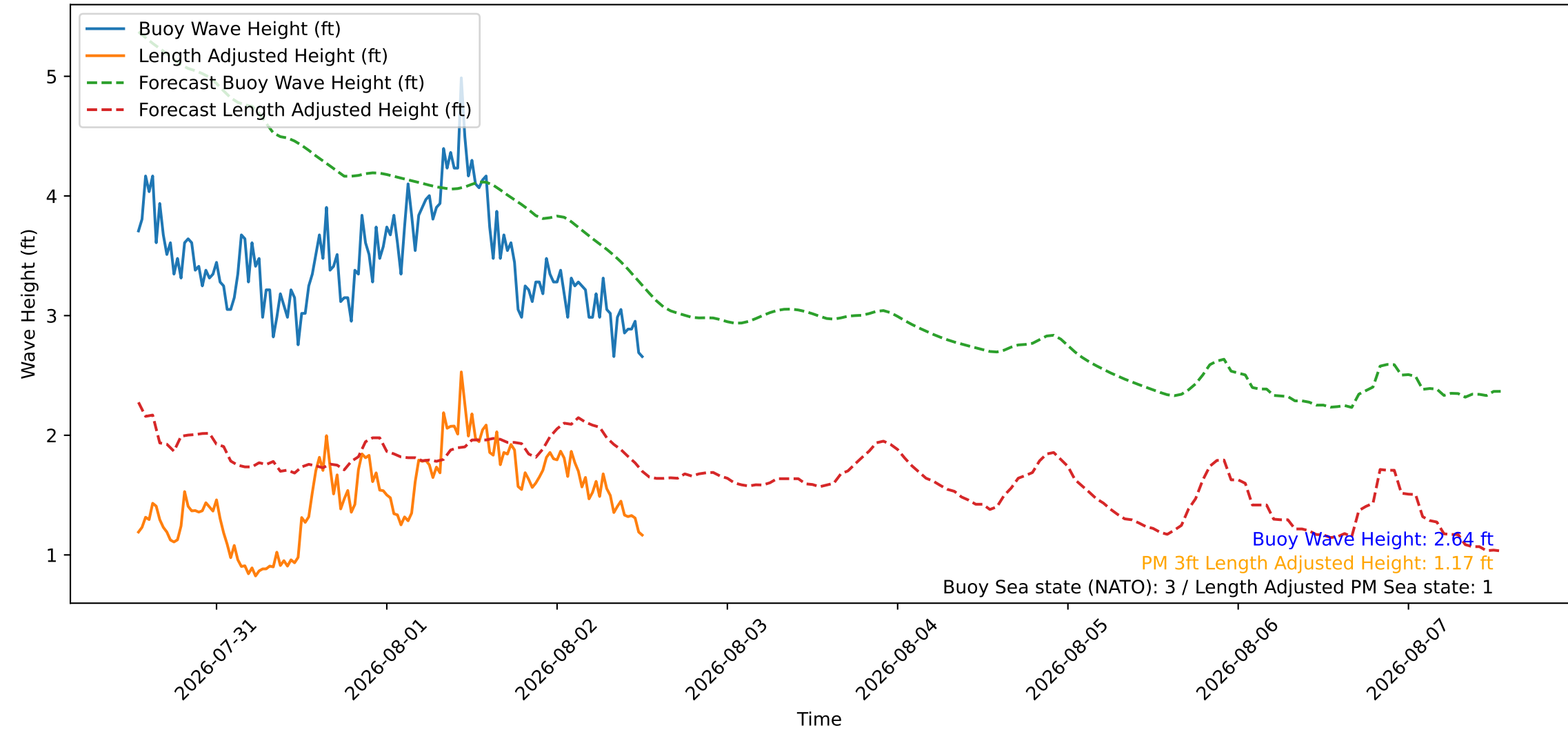
Wave Heights over Time for Green Beach at 2026-08-02 12:51:08
