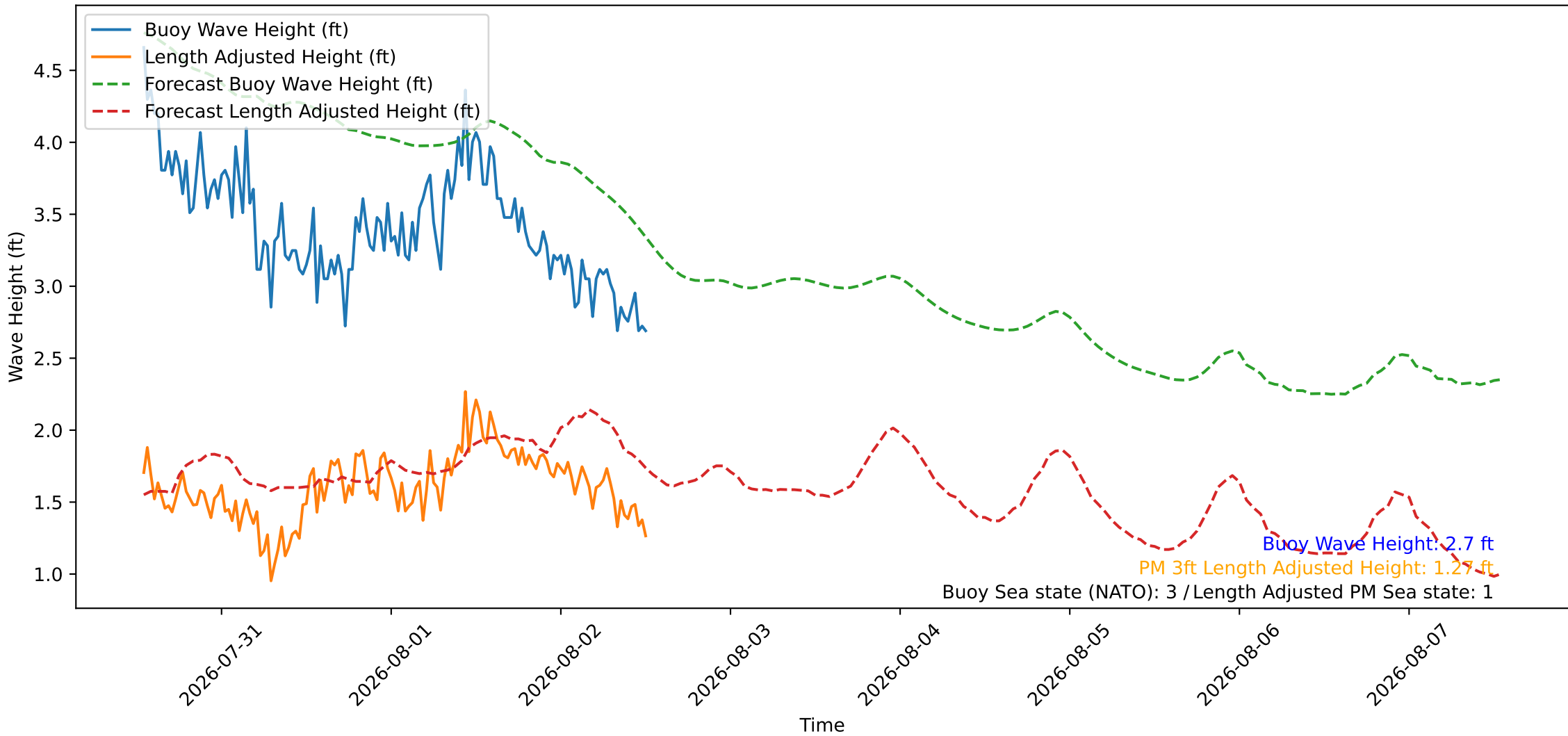
Wave Heights over Time for Oceanside Harbor at 2026-08-02 12:50:25
