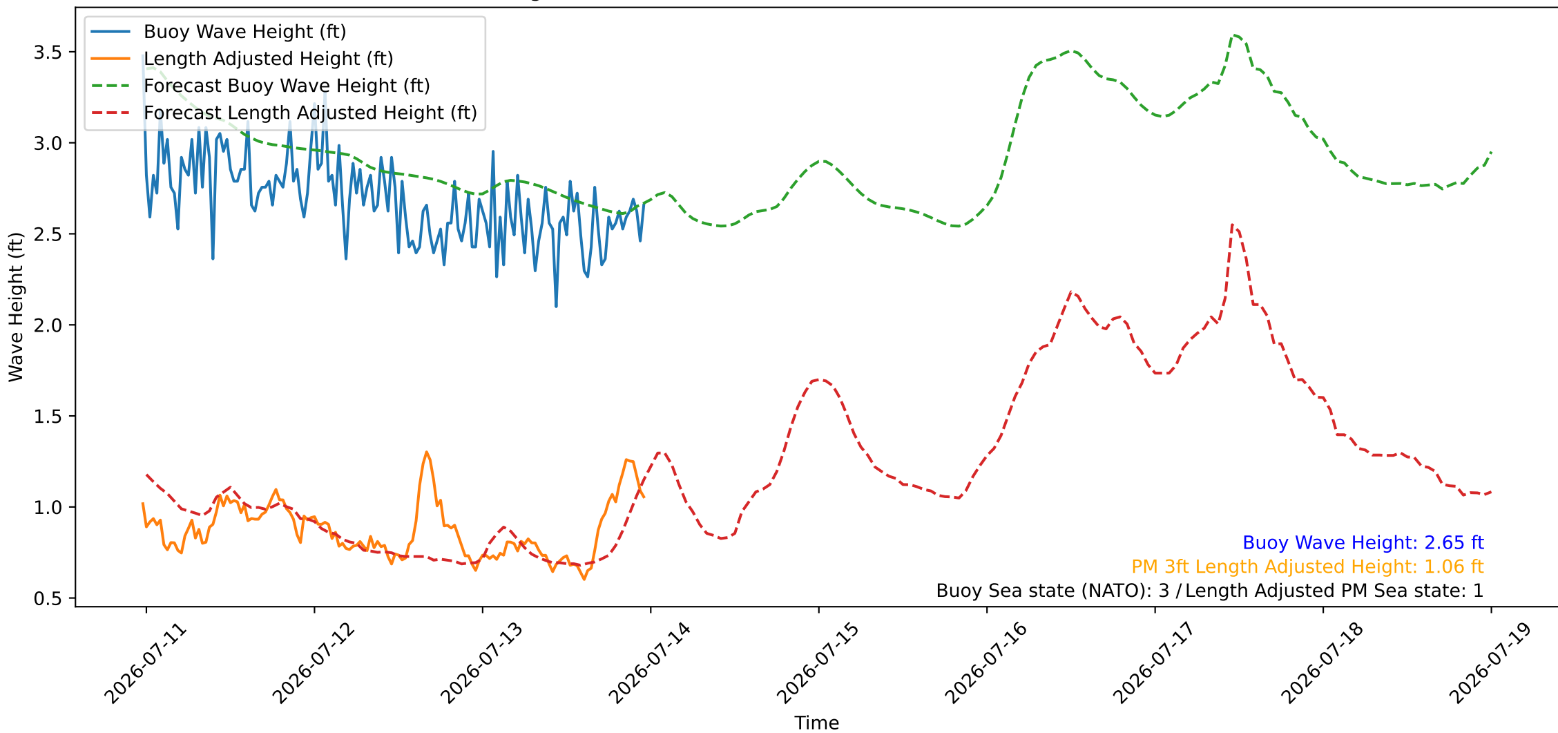
Wave Heights over Time for Oceanside Harbor at 2026-07-13 23:40:26
