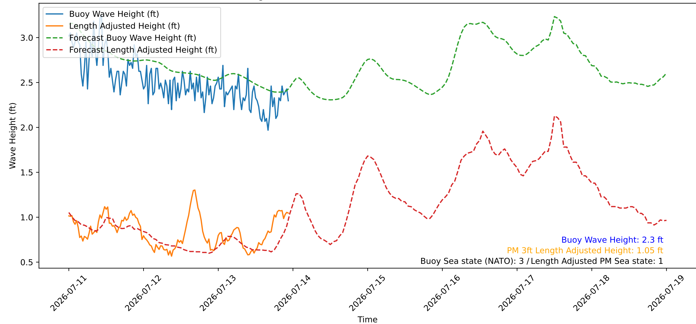
Wave Heights over Time for Red Beach at 2026-07-13 23:40:45
