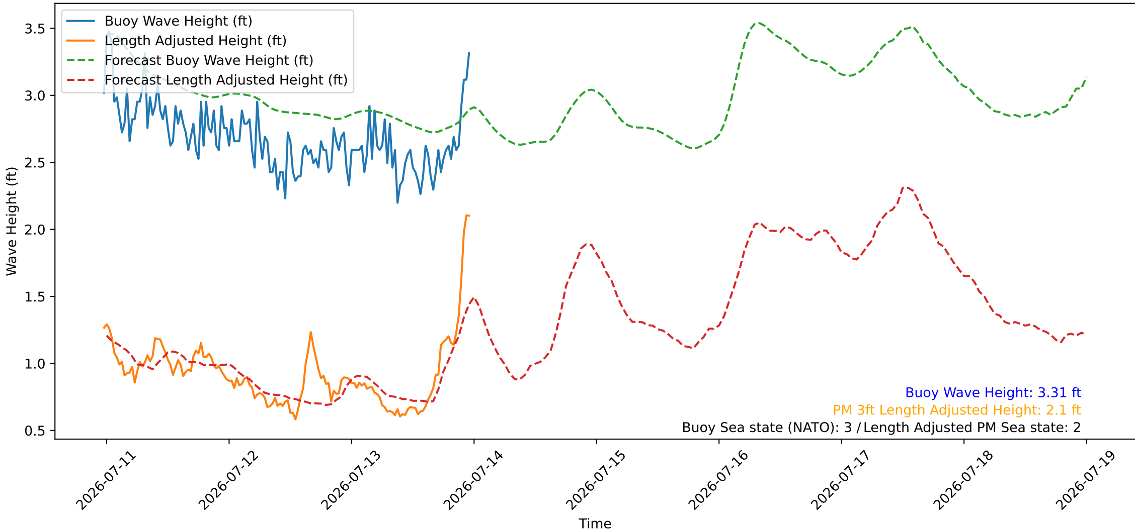
Wave Heights over Time for Green Beach at 2026-07-13 23:41:08
